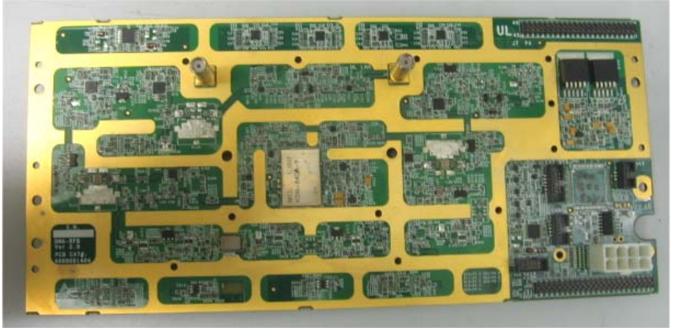
Photograph No.15 RF PCB front view
