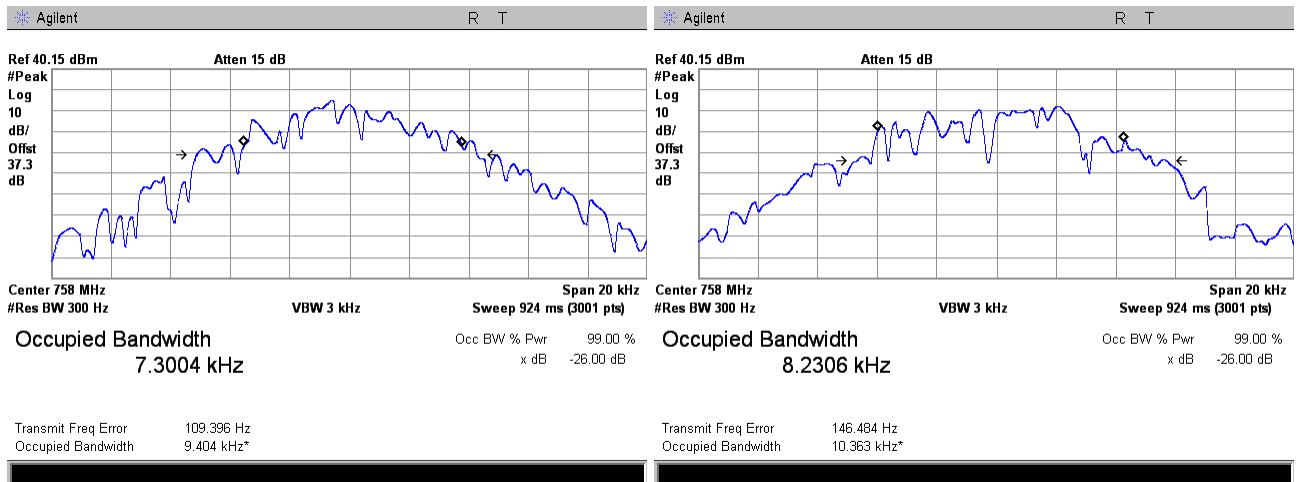
Plot 7.2.2 Occupied bandwidth test result at mid frequency carrier, Port 1
