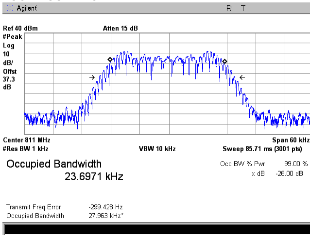
Plot 7.2.36 Occupied bandwidth test result at high frequency carrier, Port 2
