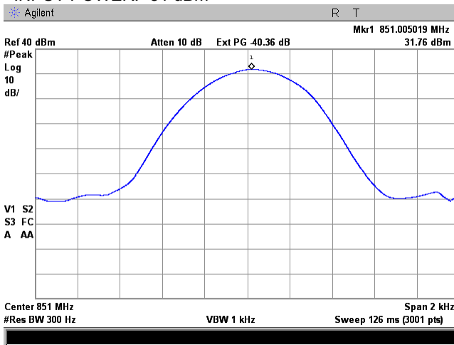
Plot 7.3.8 Reference level test results at mid carrier frequency, Port 1
