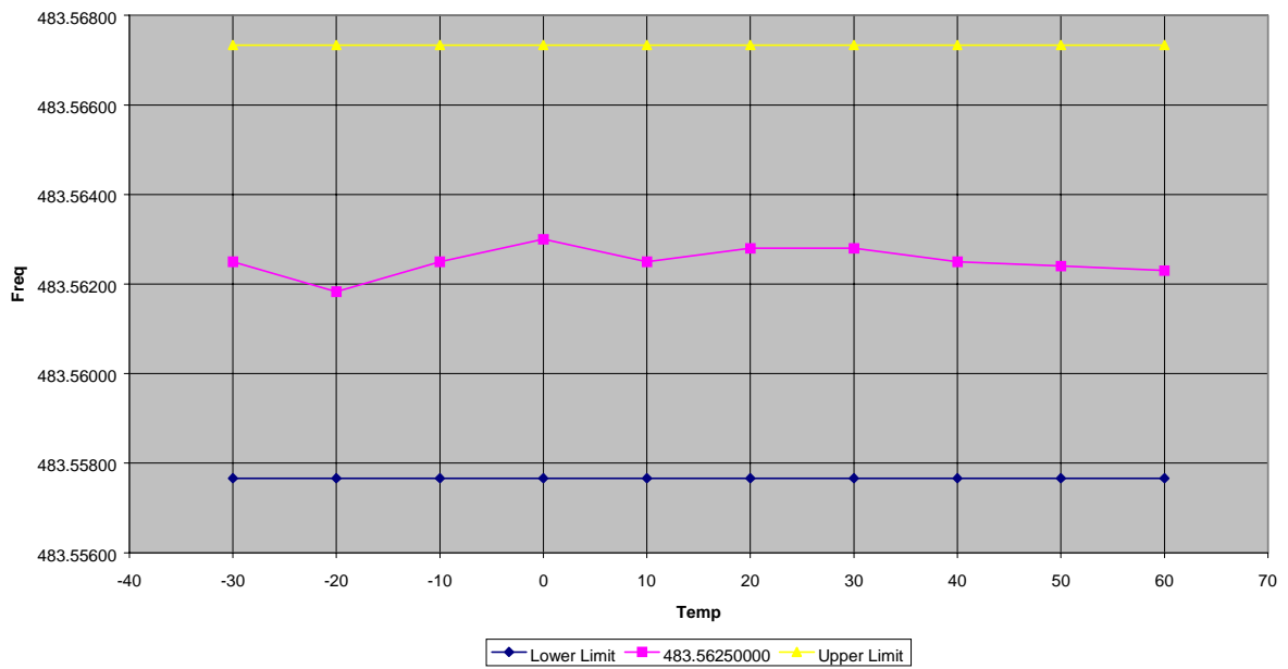
Downlink - 483.5625MHz Frequency Stability - Temperature
