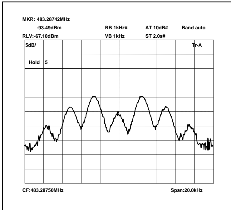
483.2875MHz Signal Generator deviation set to 5kHz
