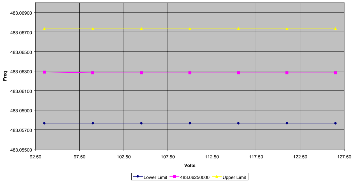
Downlink - 60-055902 - 483.0625MHz Frequency Stability - Voltage
