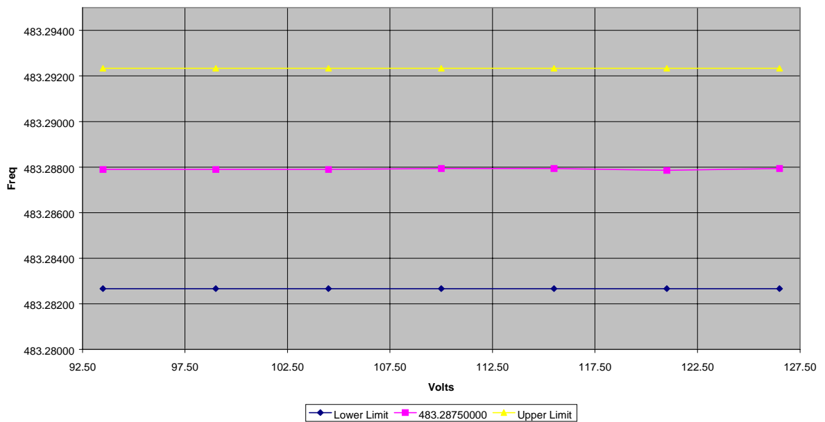
Downlink - 60-055902 - 483.2875MHz Frequency Stability - Voltage
