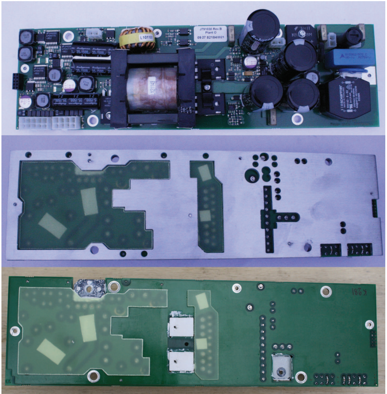
J791001 PSU
