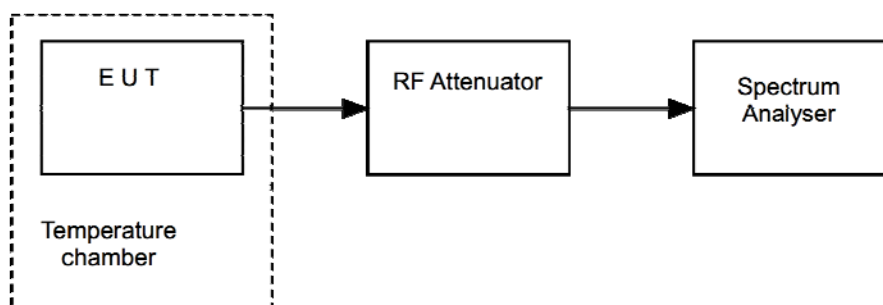
Figure x Test Setup
