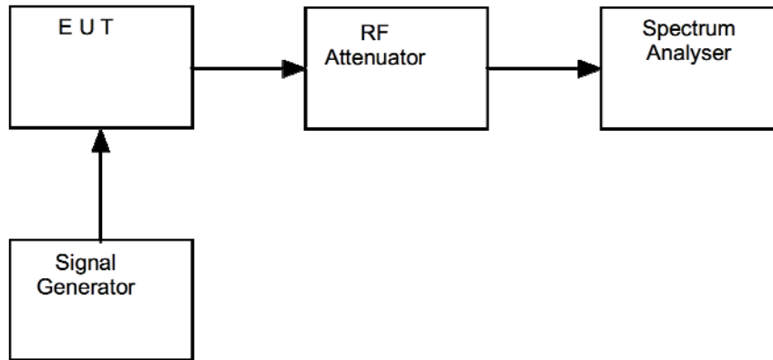
Figure iv Test Setup
