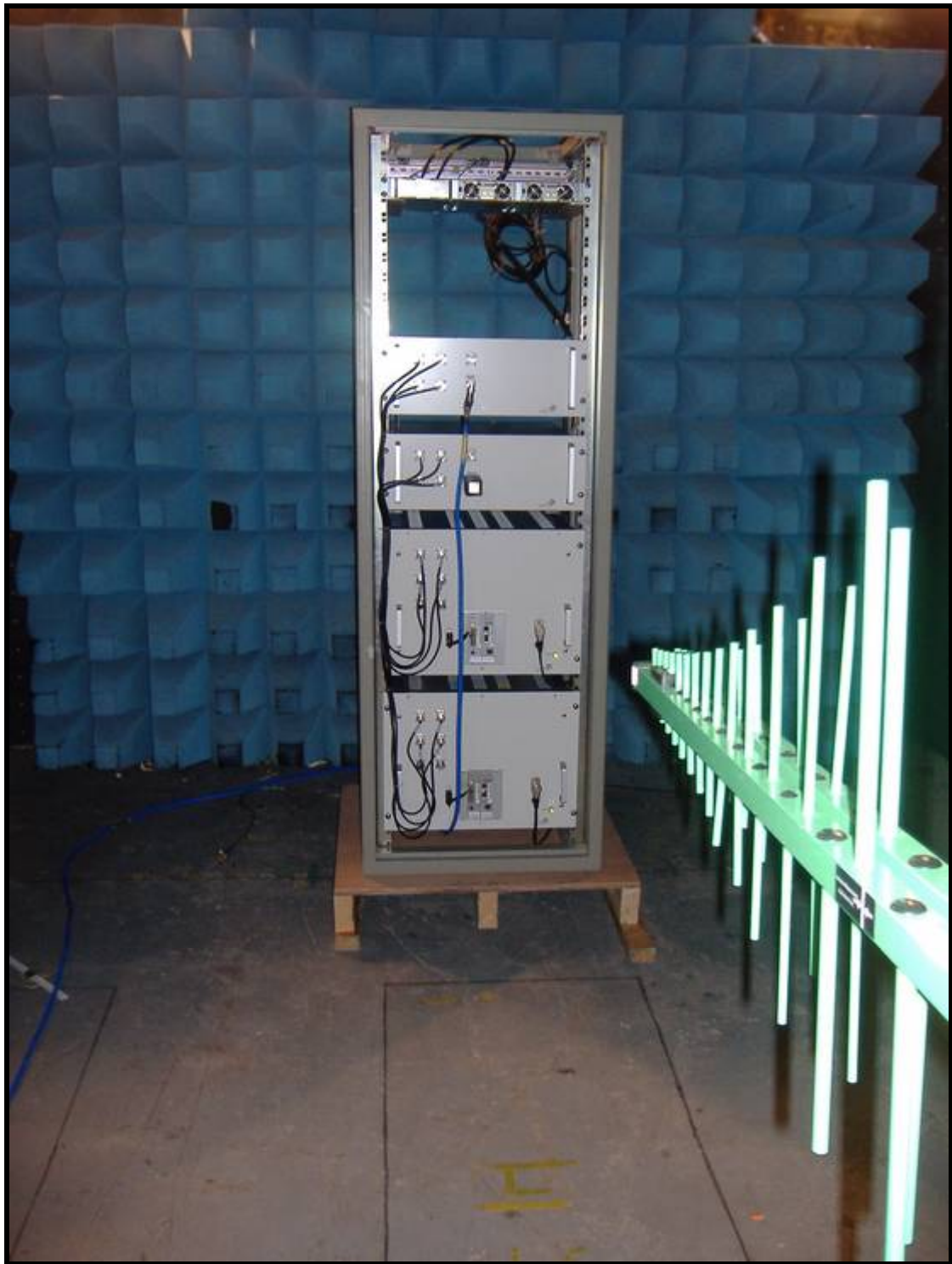
Radiated Test Setup (30MHz – 1GHz)
