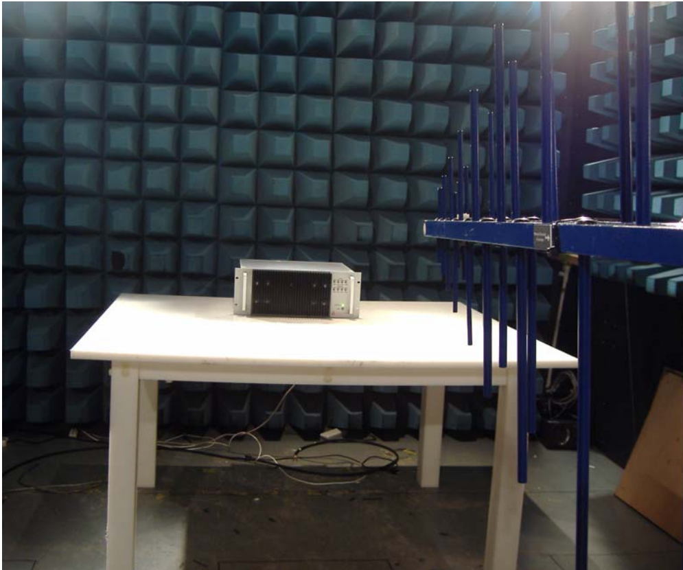
60-214802 Test Setup
