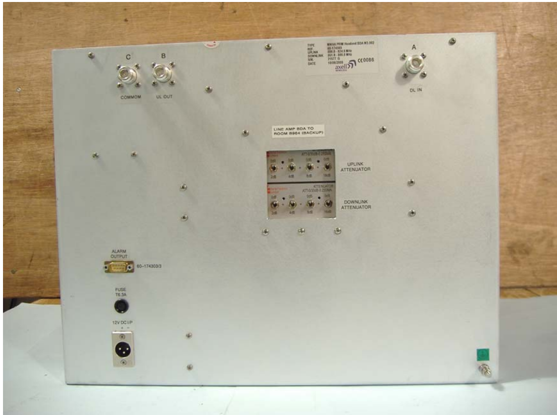
60 174303 Rear View
