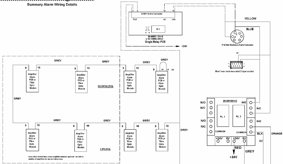
GENERIC CELL ENHANCER ALARM WIRING
