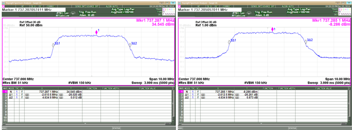
Plot 3.2.1: Input-versus-output signal comparison, AWGN 4.1MHz
