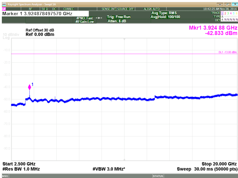
Plot 3.5.4: Spurious Emission Conducted Measurement, MSK Gaussian filter 0.3 data rate 270kbps, Fc = 1962.500, 2.5 GHz – 20.0 GHz
