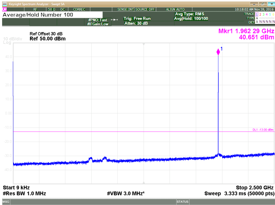
Plot 3.5.3: Spurious Emission Conducted Measurement, MSK Gaussian filter 0.3 data rate 270kbps, Fc = 1962.500, 9 kHz – 2.5 GHz
