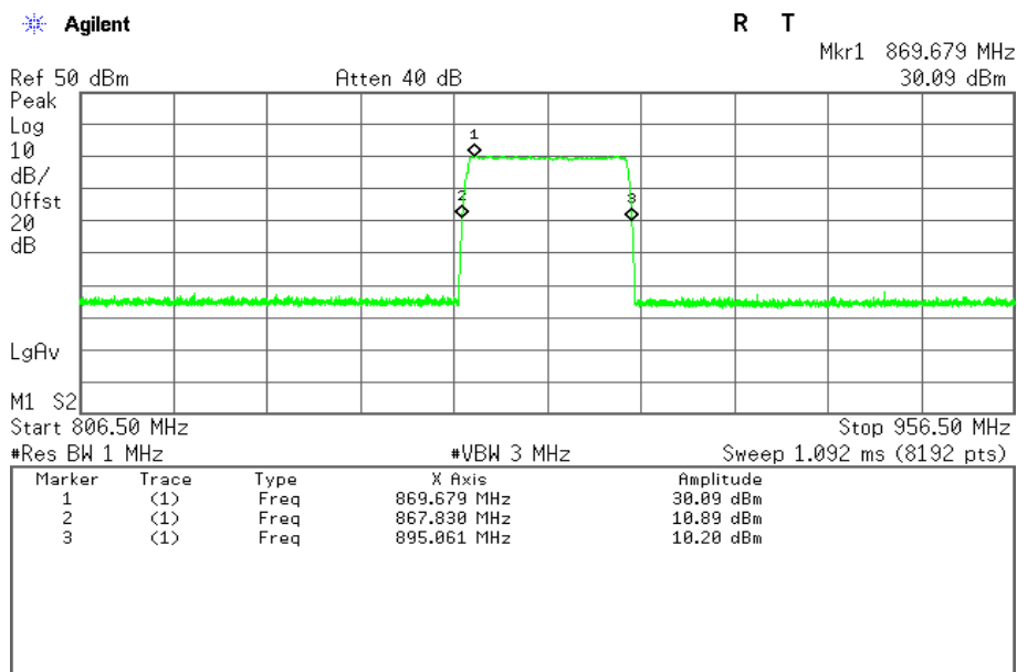
Plot 3.1: Out-of-Band rejection, CW
