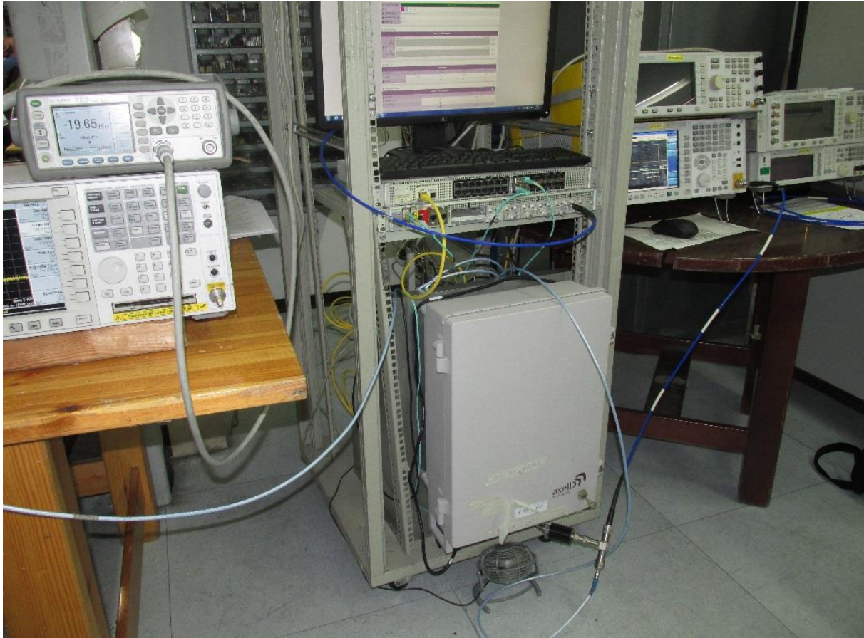
Figure 1 - Setup for Conducted Test @ antenna port
