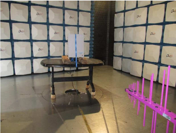
Figure 2 - Radiation Test Setup [1 of 3]
