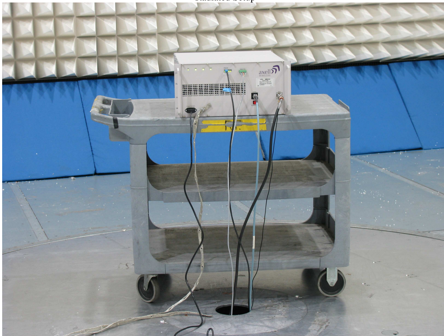
Radiated Setup
