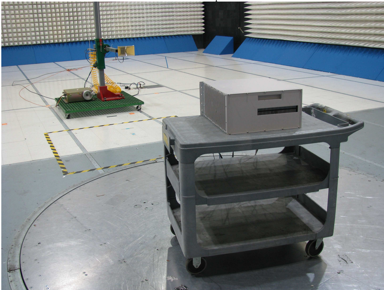
Radiated Setup
