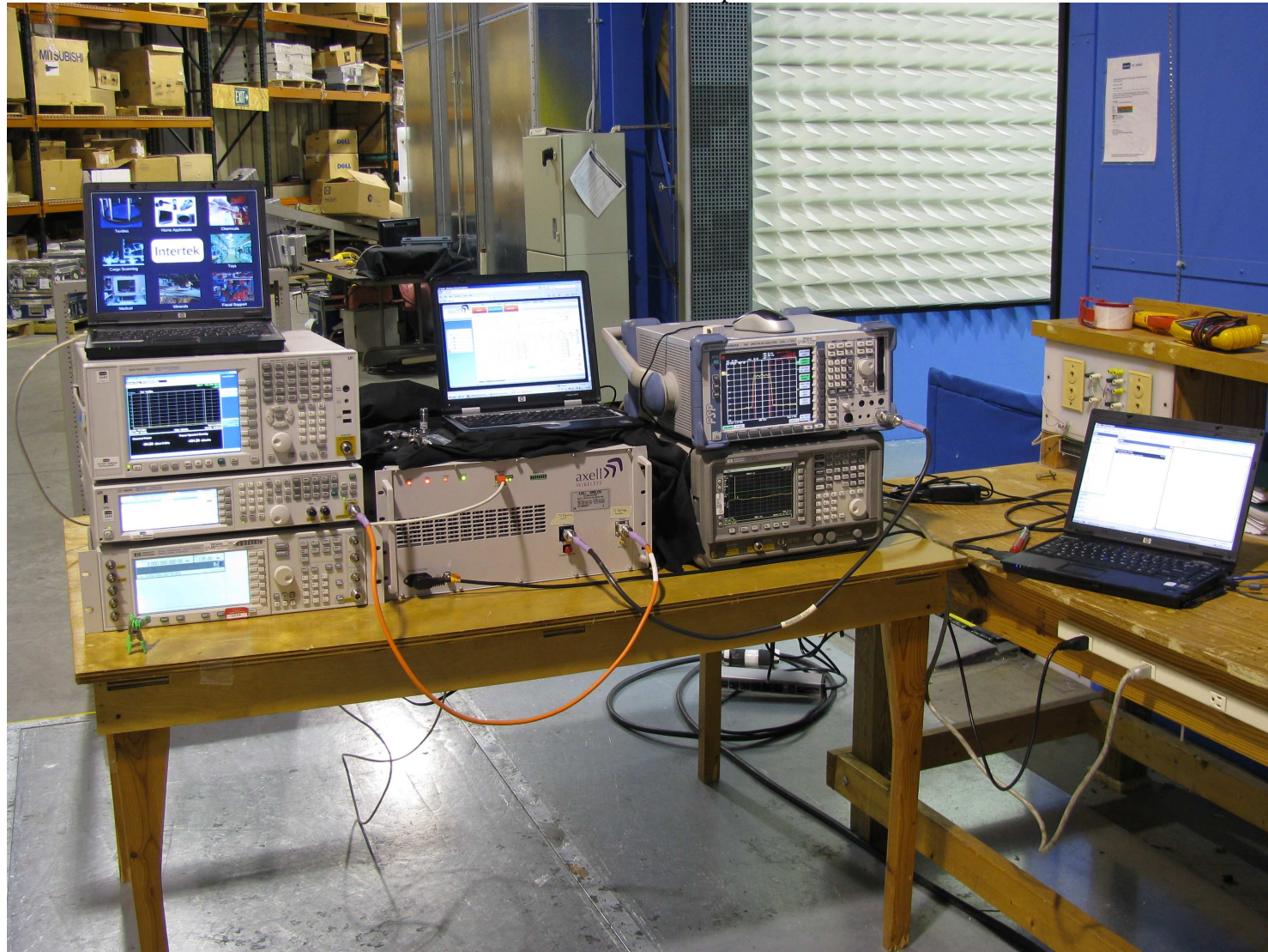
Conducted Setup
