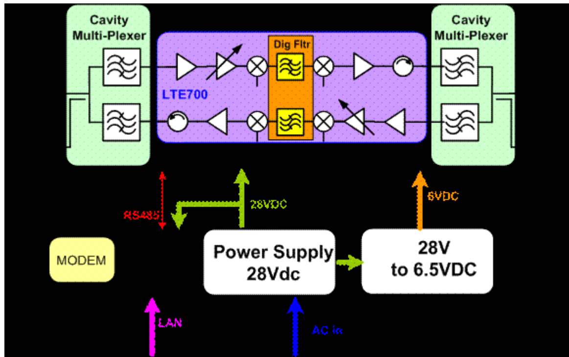
Axell 3307D Block Diagram
