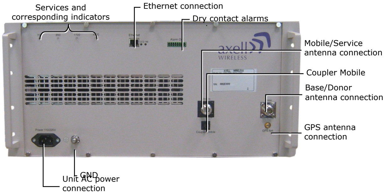
Figure 2. D-MBR Front Panel
