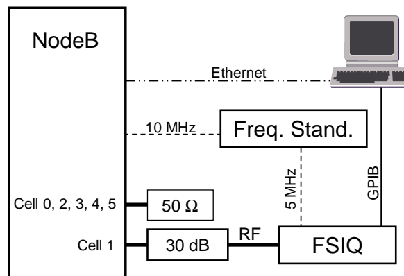
Fig. 1 – Test Configuration
