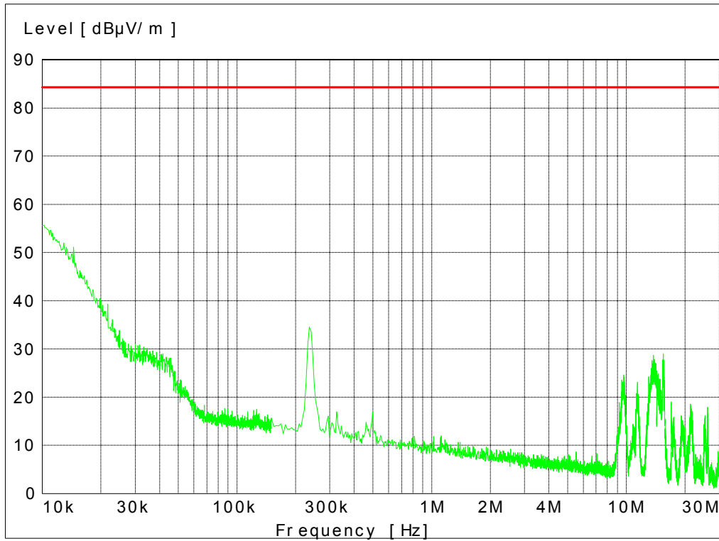
Fig. 30 – Radiated Emission 10 kHz – 30 MHz
