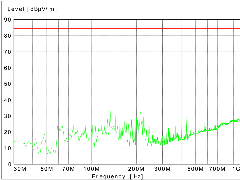
Fig. 31 – Radiated Emission 30 MHz – 1 GHz
