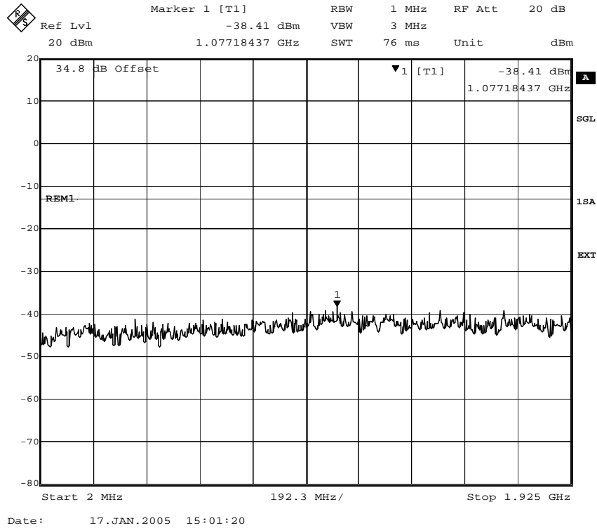
Fig. 24 – Spurious emissions in the frequency range 2 MHz – 1925 MHz (GMSK modulation).
