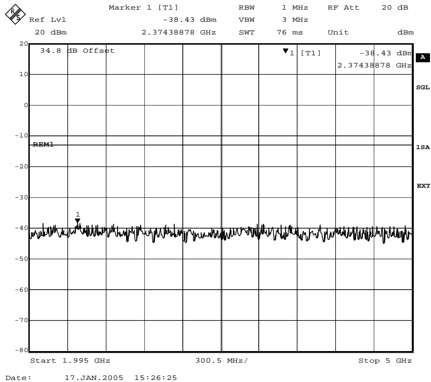
Fig. 63 – Spurious emissions in the frequency range 1995 MHz – 5000 MHz (8PSK modulation).
