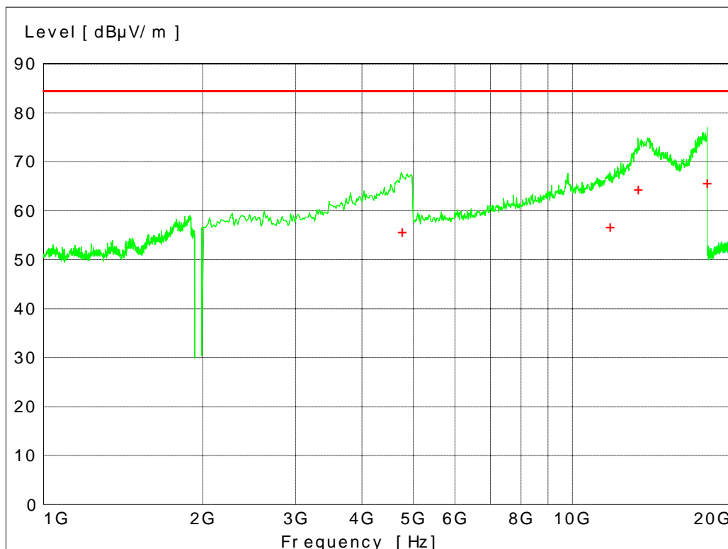
Fig. 73 – Radiated Emission 1 GHz – 20 GHz, GMSK modulation.
