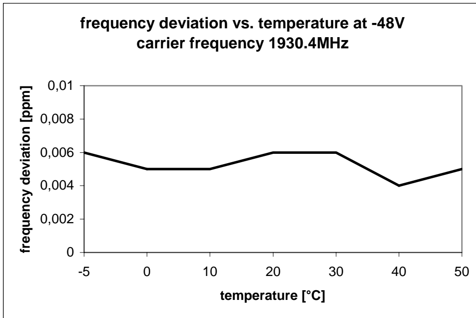
Fig. 75 – Frequency deviation vs. temperature (48V, 1930.4 MHz, GMSK modulation)
