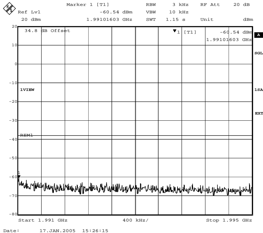
Fig. 61 – Spurious emissions in the frequency range 1991 MHz – 1995 MHz (8PSK modulation). Limit: -13dBm-25.2dB=-38.2dBm
