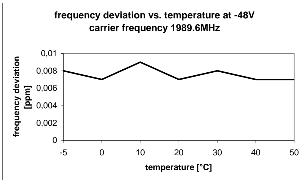
Fig. 78 – Frequency deviation vs. temperature (48V, 1989.6 MHz, 8PSK modulation)
