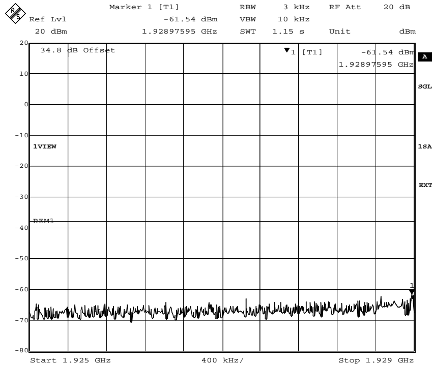
Fig. 26 – Spurious emissions in the frequency range 1925 MHz–1929 MHz (GMSK modulation). Limit: -13dBm–25.2dB–38.2dBm
