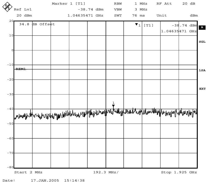
Fig. 39 – Spurious emissions in the frequency range 2 MHz – 1925 MHz (8PSK modulation).
