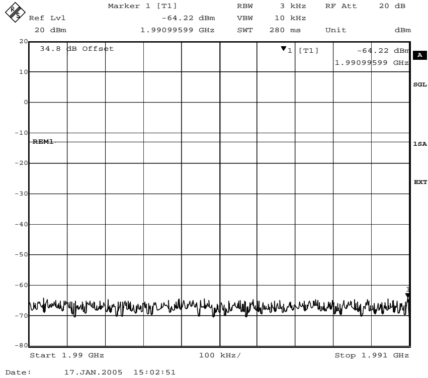
Fig. 30 – Spurious emissions in the frequency range 1990 MHz – 1991 MHz (GMSK modulation).
