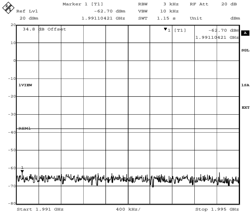
Fig. 46 – Spurious emissions in the frequency range 1991 MHz – 1995 MHz (GMSK modulation). Limit: -13dBm–25.2dB–38.2dBm
