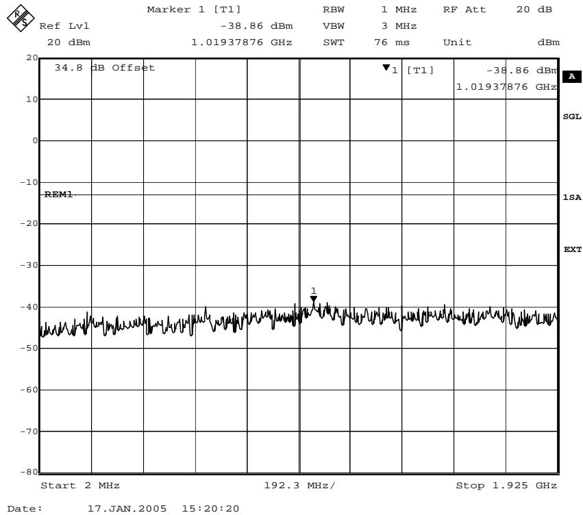
Fig. 52 – Spurious emissions in the frequency range 2 MHz – 1925 MHz (GMSK modulation).
