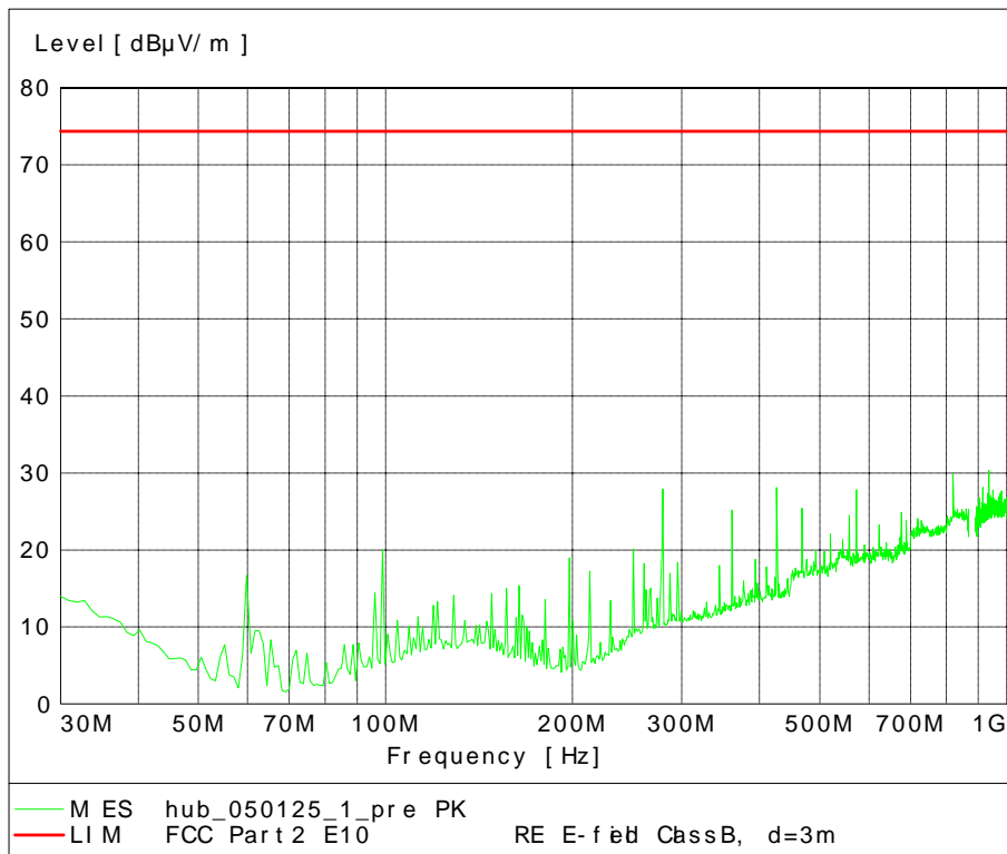
Fig. 71 – Radiated Emission 30 MHz – 1 GHz, GMSK modulation.
