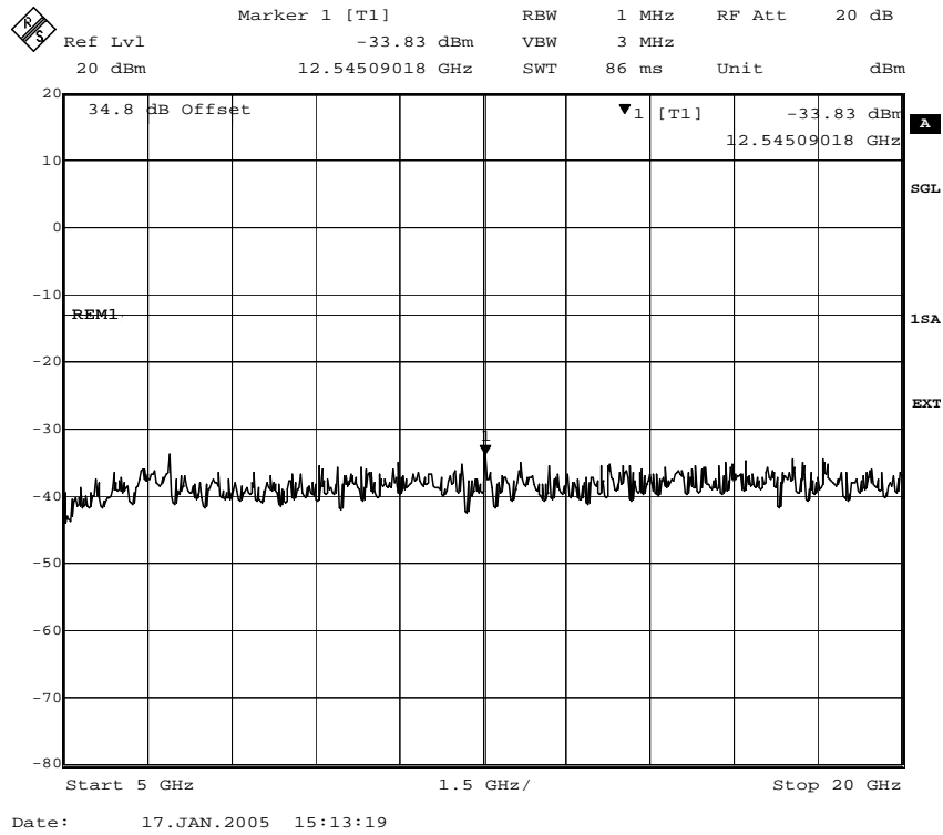
Fig. 50 – Spurious emissions in the frequency range 5000 MHz–20000 MHz (GMSK modulation).
