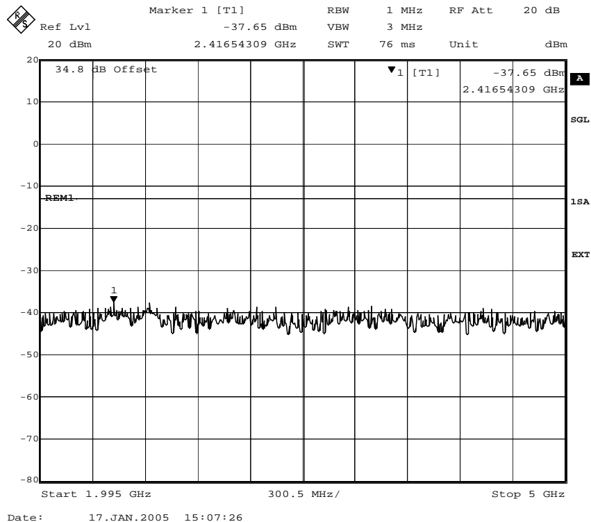
Fig. 35 – Spurious emissions in the frequency range 1995 MHz – 5000 MHz (8PSK modulation).
