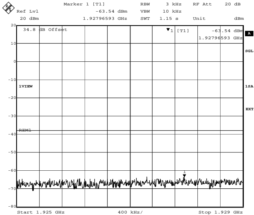
Fig. 40 – Spurious emissions in the frequency range 1925 MHz–1929 MHz (GMSK modulation). Limit: -13dBm–25.2dB–38.2dBm
