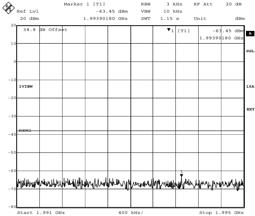
Fig. 32 – Spurious emissions in the frequency range 1991 MHz – 1995 MHz (GMSK modulation). Limit: -13dBm-25.2dB=-38.2dBm
