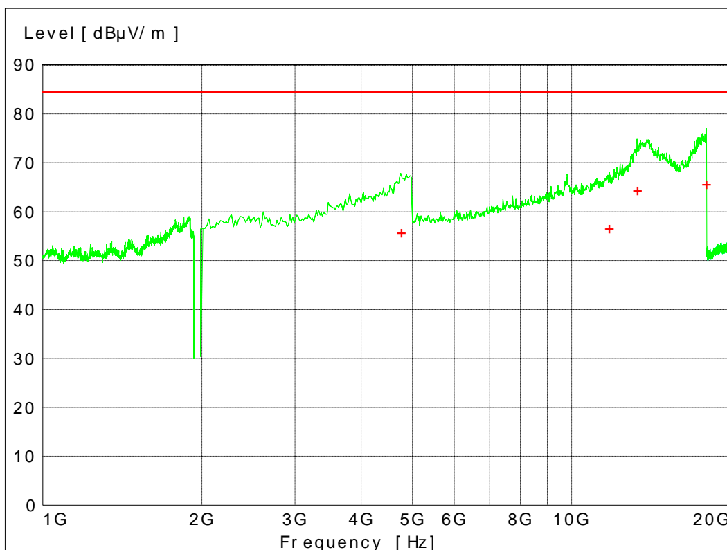
Fig. 74 – Radiated Emission 1 GHz – 20 GHz, 8PSK modulation.
