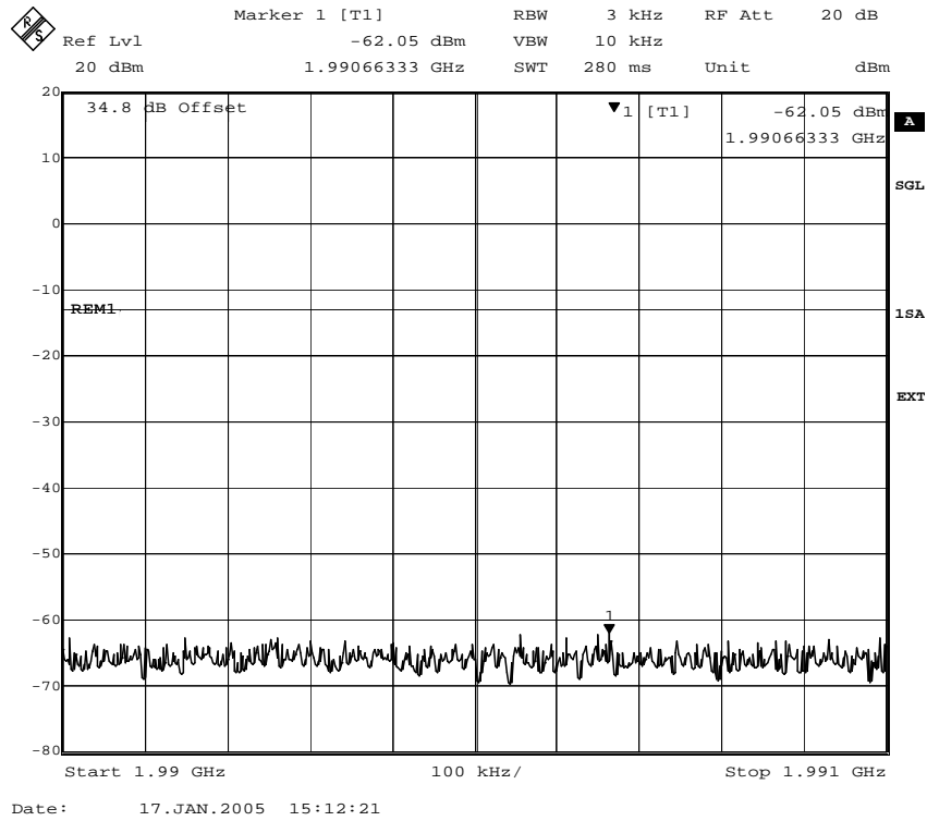
Fig. 44 – Spurious emissions in the frequency range 1990 MHz – 1991 MHz (GMSK modulation).
