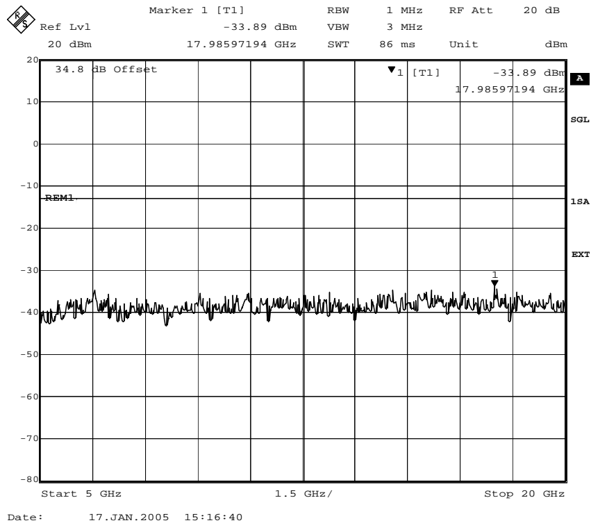
Fig. 51 – Spurious emissions in the frequency range 5000 MHz–20000 MHz (8PSK modulation).
