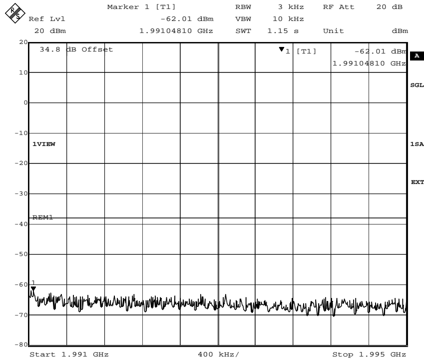
Fig. 60 – Spurious emissions in the frequency range 1991 MHz – 1995 MHz (GMSK modulation). Limit: -13dBm-25.2dB=-38.2dBm
