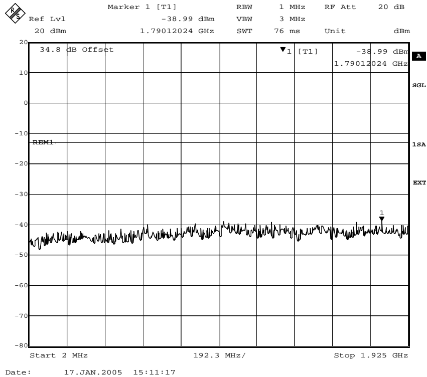
Fig. 38 – Spurious emissions in the frequency range 2 MHz – 1925 MHz (GMSK modulation).
