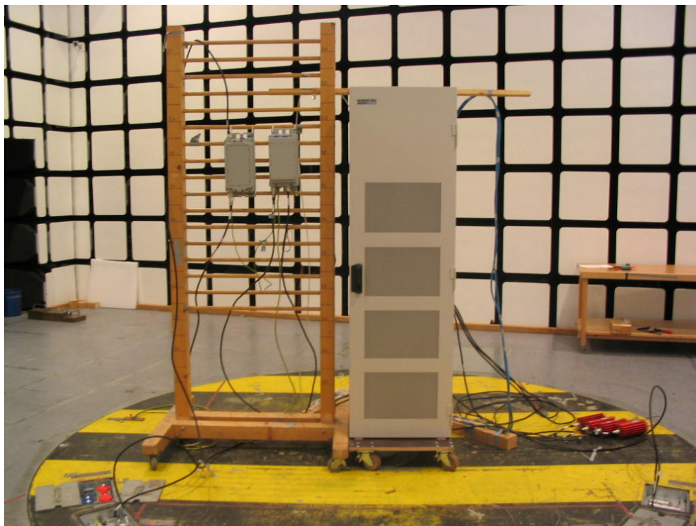
Fig. 67 – Photograph of the anechoic chamber with the EUT.
