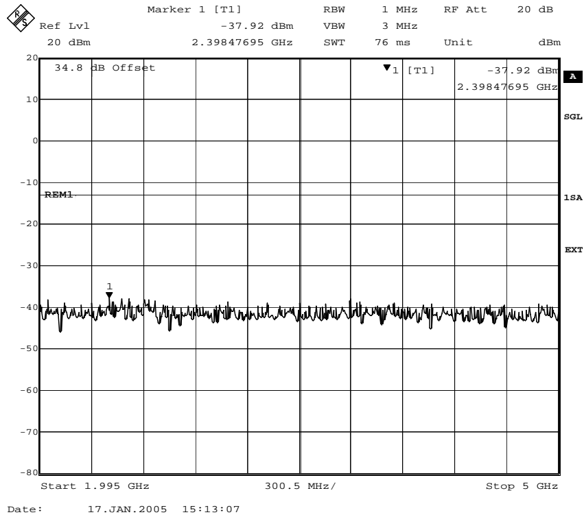
Fig. 48 – Spurious emissions in the frequency range 1995 MHz – 5000 MHz (GMSK modulation).
