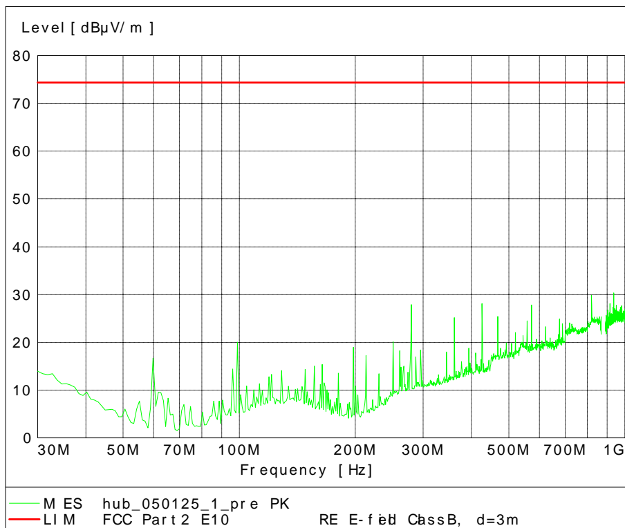
Fig. 72 – Radiated Emission 30 MHz – 1 GHz, 8PSK modulation.
