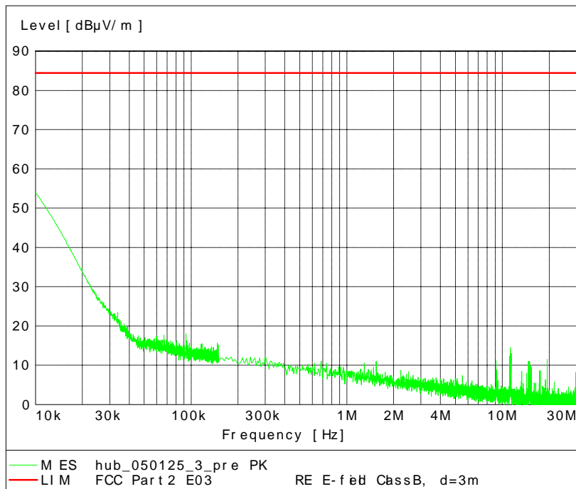
Fig. 70 – Radiated Emission 10 kHz – 30 MHz, 8PSK modulation.
