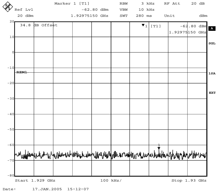
Fig. 42 – Spurious emissions in the frequency range 1929 MHz – 1930 MHz (GMSK modulation).
