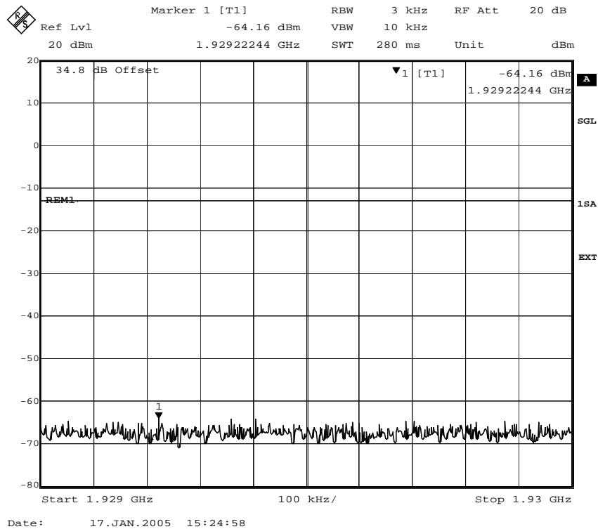
Fig. 57 – Spurious emissions in the frequency range 1929 MHz – 1930 MHz (8PSK modulation).
