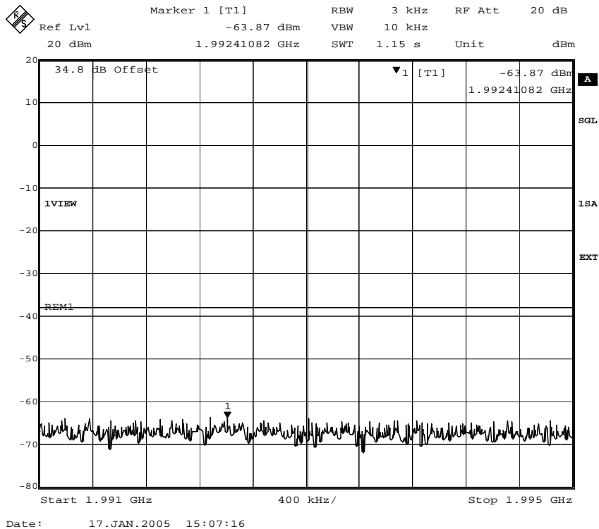
Fig. 33 – Spurious emissions in the frequency range 1991 MHz – 1995 MHz (8PSK modulation). Limit: -13dBm-25.2dB=-38.2dBm
