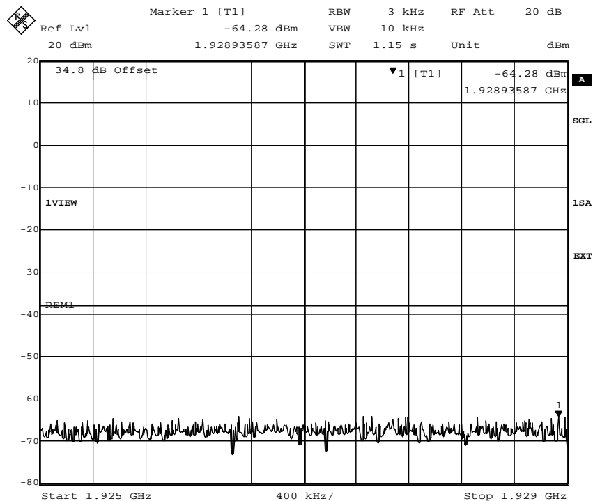
Fig. 54 – Spurious emissions in the frequency range 1925 MHz – 1929 MHz (GMSK modulation). Limit: -13dBm–25.2dB–38.2dBm
