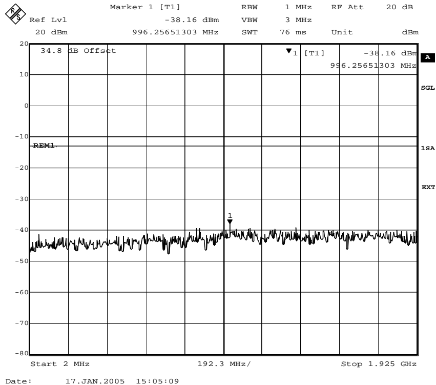
Fig. 25 – Spurious emissions in the frequency range 2 MHz – 1925 MHz (8PSK modulation).
