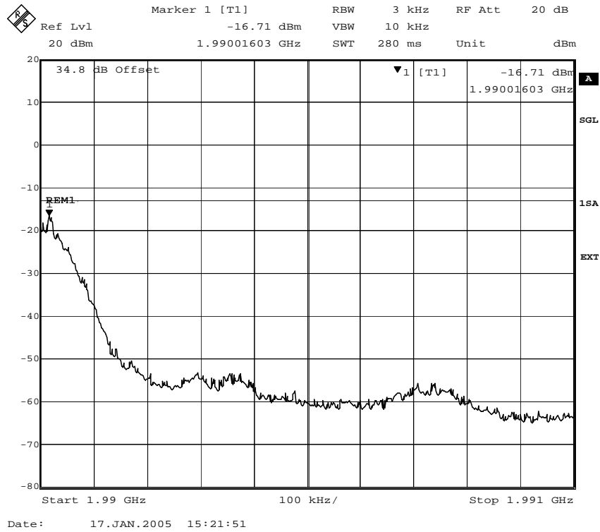
Fig. 58 – Spurious emissions in the frequency range 1990 MHz – 1991 MHz (GMSK modulation).
