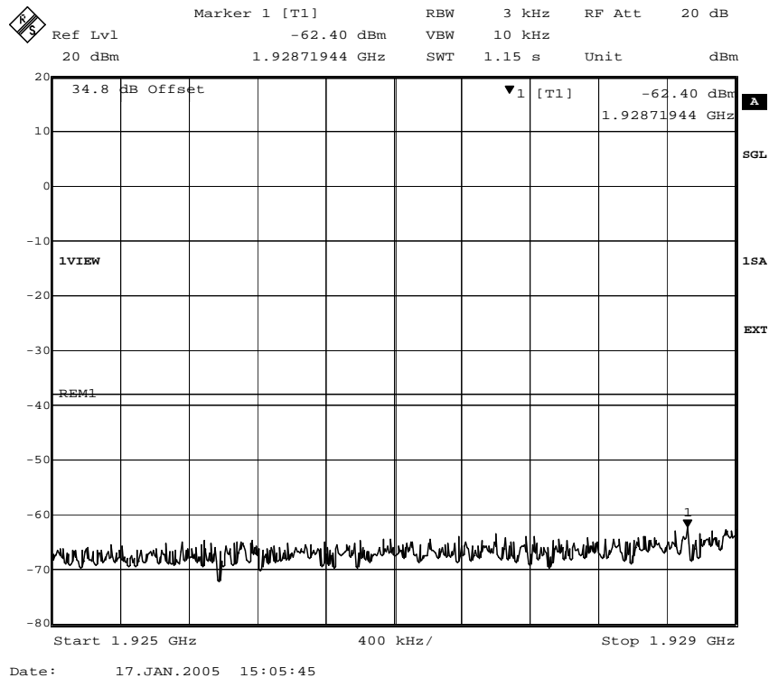
Fig. 27 – Spurious emissions in the frequency range 1925 MHz–1929 MHz (8PSK modulation). Limit: -13dBm–25.2dB–38.2dBm
