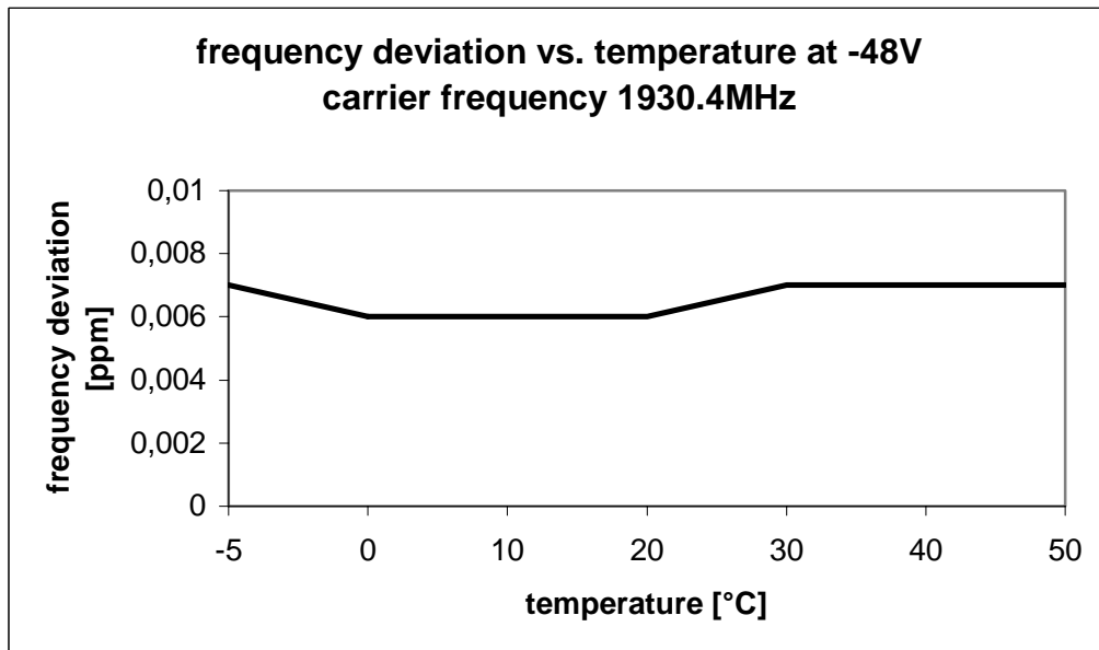
Fig. 76 – Frequency deviation vs. temperature (48V, 1930.4 MHz, 8PSK modulation)
