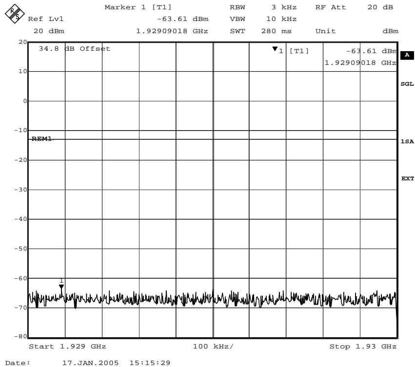
Fig. 43 – Spurious emissions in the frequency range 1929 MHz – 1930 MHz (8PSK modulation).
