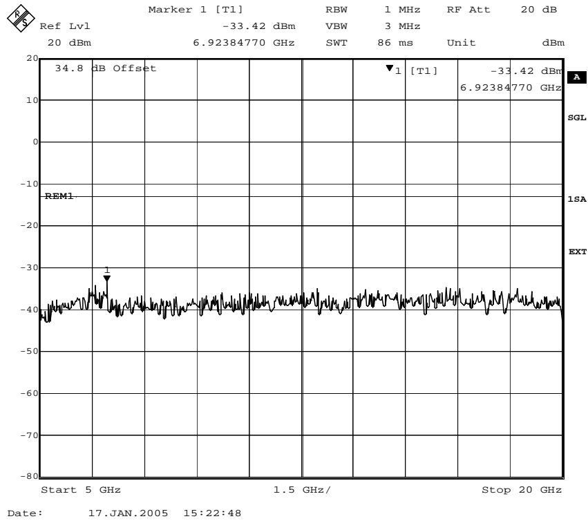
Fig. 64 – Spurious emissions in the frequency range 5000 MHz–20000 MHz (GMSK modulation).
