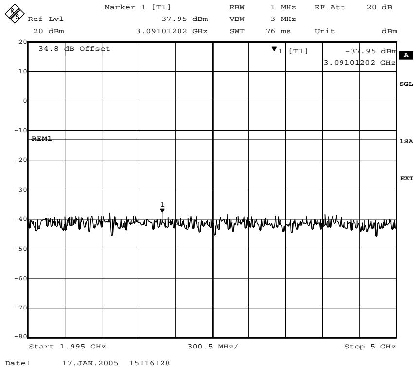
Fig. 49 – Spurious emissions in the frequency range 1995 MHz – 5000 MHz (8PSK modulation).
