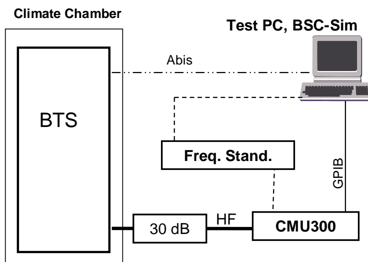
Fig. 2 – Measurement Test Configuration
