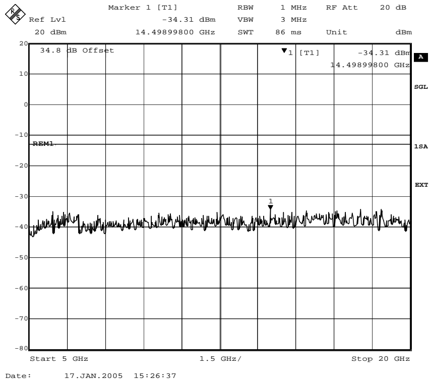
Fig. 65 – Spurious emissions in the frequency range 5000 MHz–20000 MHz (8PSK modulation).
