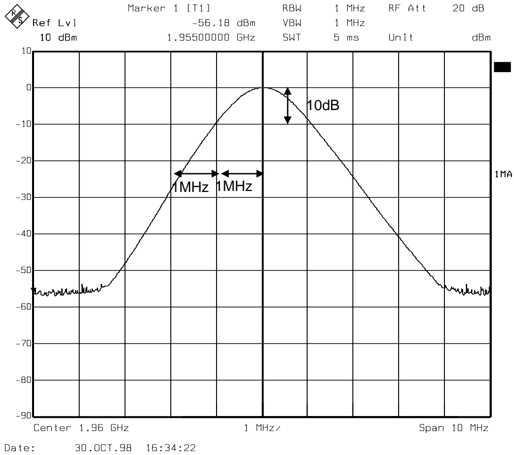
Fig. 66 – Filter characteristic of the 1 MHz resolution filter.
