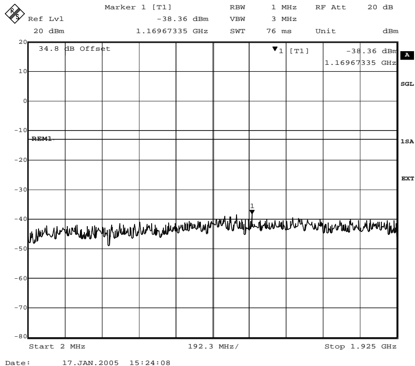
Fig. 53 – Spurious emissions in the frequency range 2 MHz – 1925 MHz (8PSK modulation).
