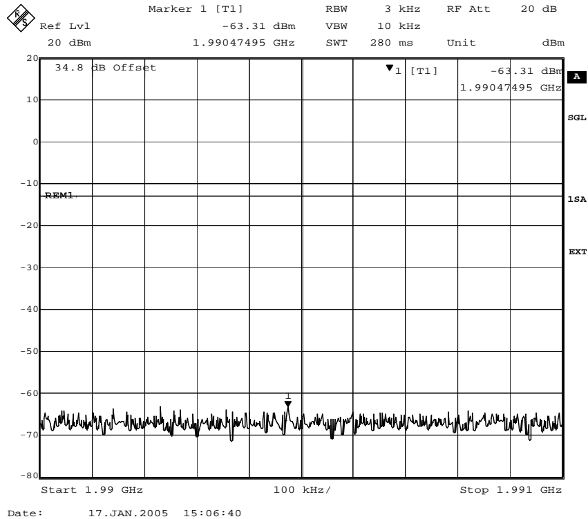
Fig. 31 – Spurious emissions in the frequency range 1990 MHz – 1991 MHz (8PSK modulation).
