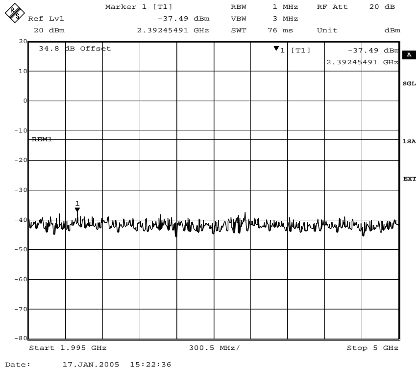
Fig. 62 – Spurious emissions in the frequency range 1995 MHz – 5000 MHz (GMSK modulation).
