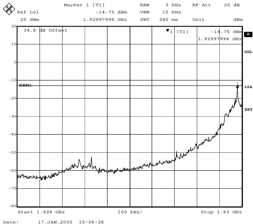
Fig. 29 – Spurious emissions in the frequency range 1929 MHz – 1930 MHz (8PSK modulation).
