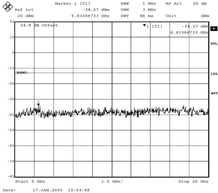
Fig. 36 – Spurious emissions in the frequency range 5000 MHz–20000 MHz (GMSK modulation).
