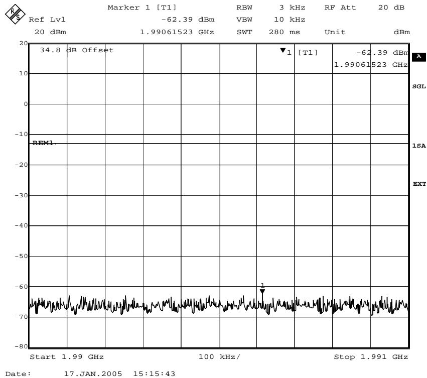
Fig. 45 – Spurious emissions in the frequency range 1990 MHz – 1991 MHz (8PSK modulation).
