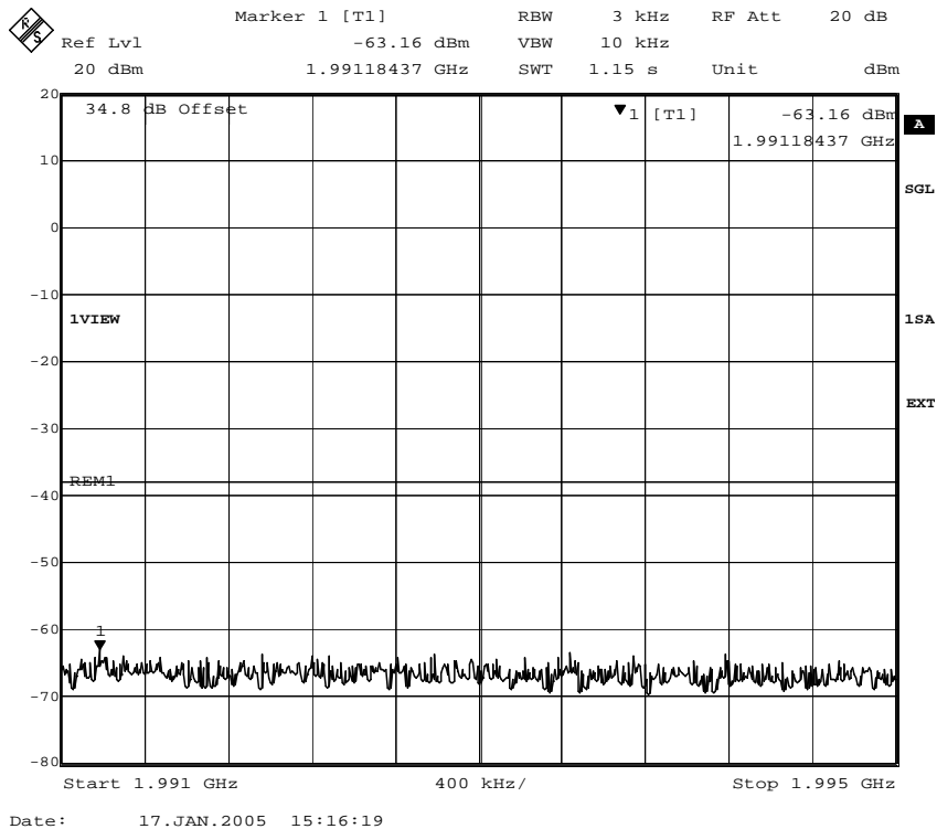
Fig. 47 – Spurious emissions in the frequency range 1991 MHz – 1995 MHz (8PSK modulation). Limit: -13dBm–25.2dB–38.2dBm
