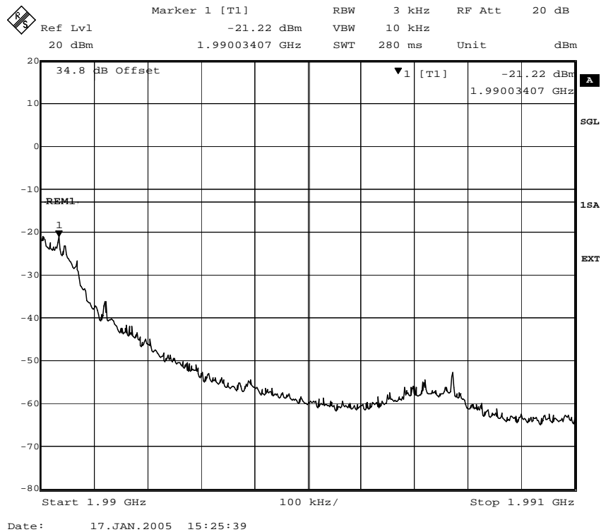
Fig. 59 – Spurious emissions in the frequency range 1990 MHz – 1991 MHz (8PSK modulation).
