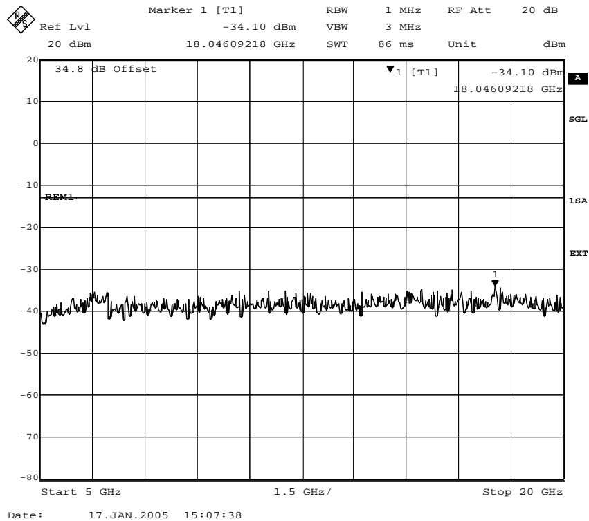
Fig. 37 – Spurious emissions in the frequency range 5000 MHz–20000 MHz (8PSK modulation).
