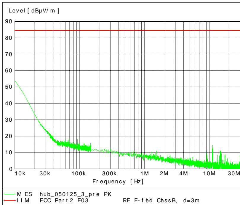
Fig. 69 – Radiated Emission 10 kHz – 30 MHz, GMSK modulation.
