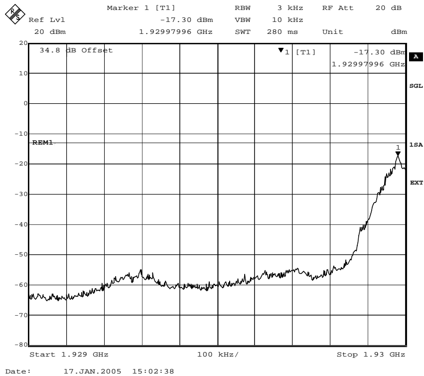
Fig. 28 – Spurious emissions in the frequency range 1929 MHz – 1930 MHz (GMSK modulation).
