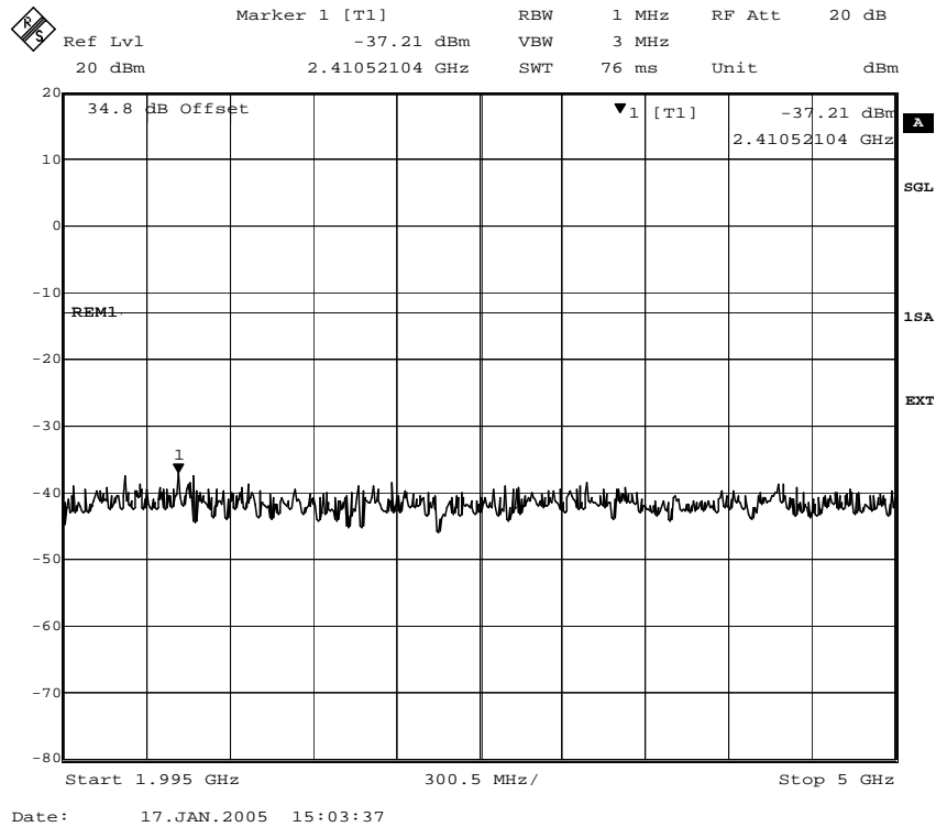
Fig. 34 – Spurious emissions in the frequency range 1995 MHz – 5000 MHz (GMSK modulation).
