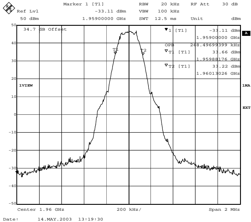
Fig. 32 – Occupied bandwidth (GMSK modulation).
