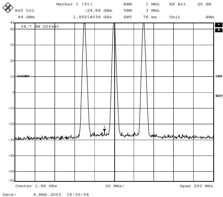
Fig. 111 – Slow frequency hopping – RBW = 1 MHz (GMSK modulation)
