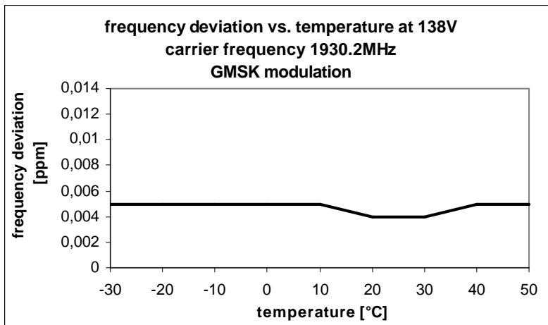
Fig. 101 – Frequency deviation vs. temperature (138V, 1930.2 MHz, GMSK modulation)
