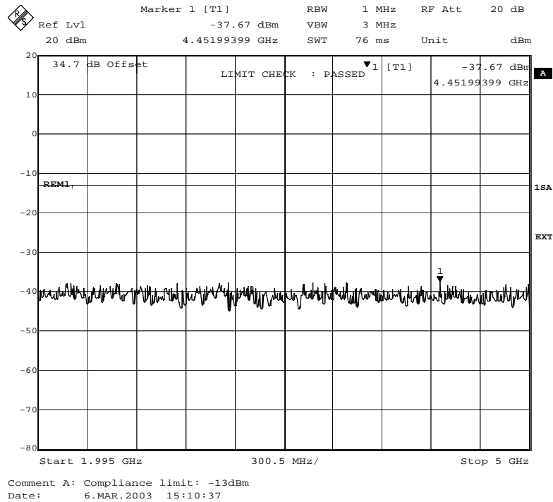
Fig. 70 – Spurious emissions in the frequency range 1995 MHz – 5000 MHz (GMSK modulation).
