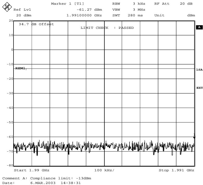
Fig. 53 – Spurious emissions in the frequency range 1990 MHz – 1991 MHz (8PSK modulation).
