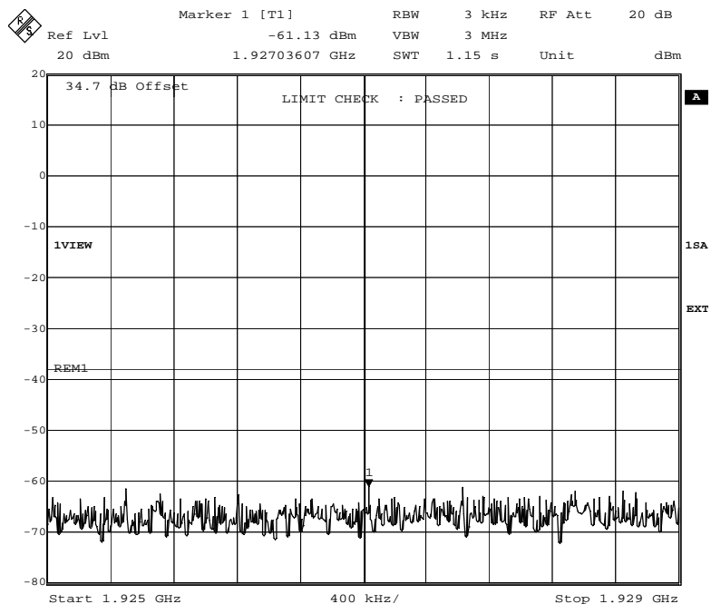
Fig. 76 – Spurious emissions in the frequency range 1925 MHz – 1929 MHz (GMSK modulation). Limit: -13dBm-25.2dB=-38.2dBm
