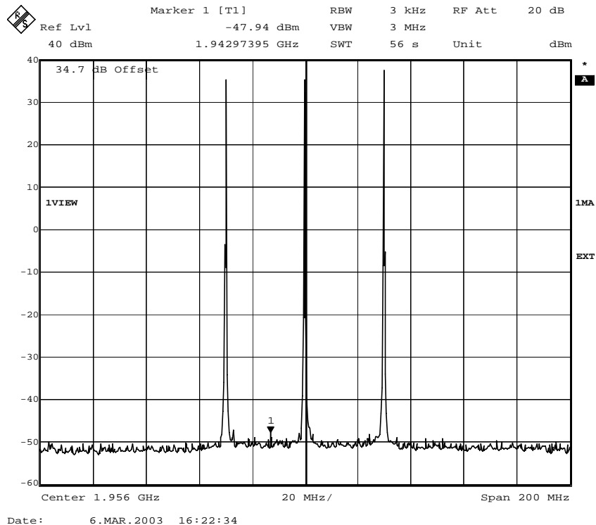
Fig. 116 – Slow frequency hopping – RBW = 3 kHz (8PSK modulation)
