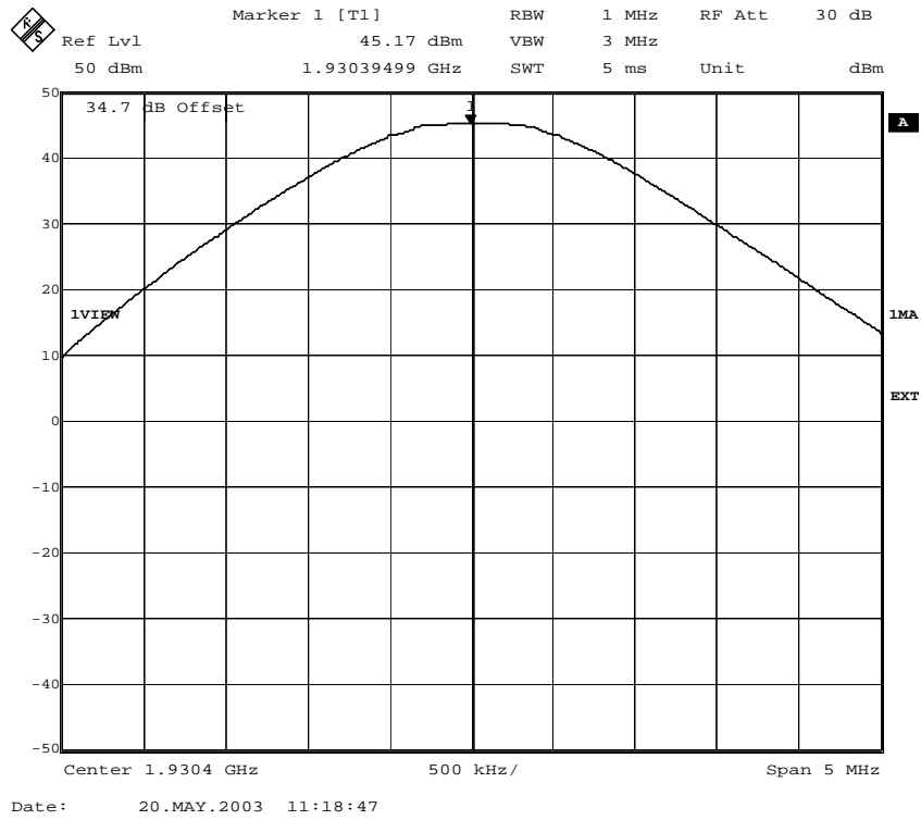
Fig. 10 – RF power at the antenna connector (GMSK modulation) for ECUPV2.
