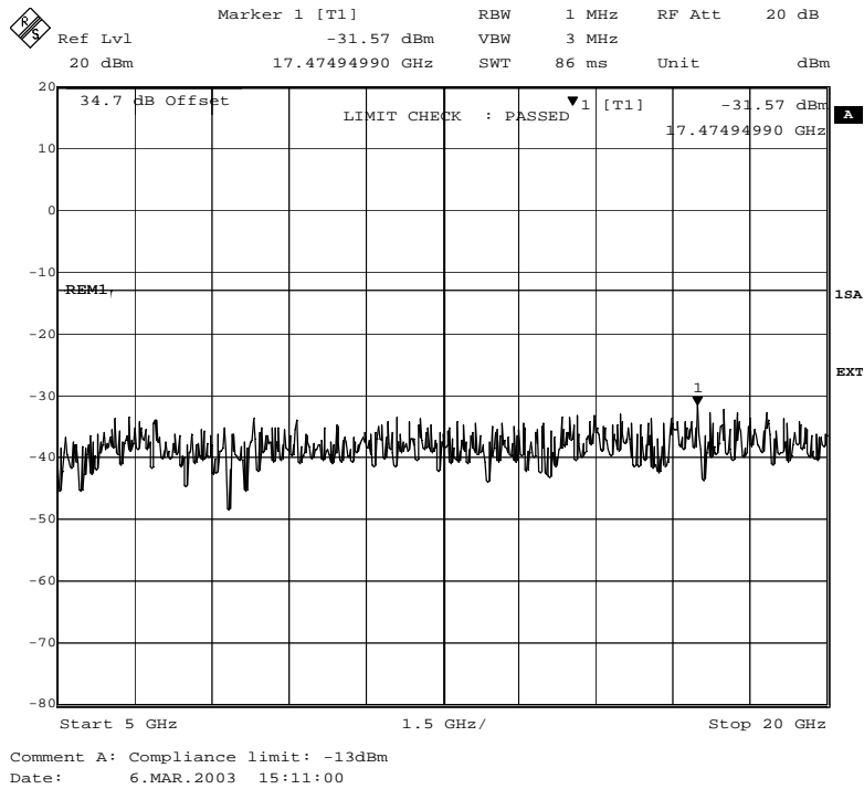
Fig. 72 – Spurious emissions in the frequency range 5000 MHz–20000 MHz (GMSK modulation).
