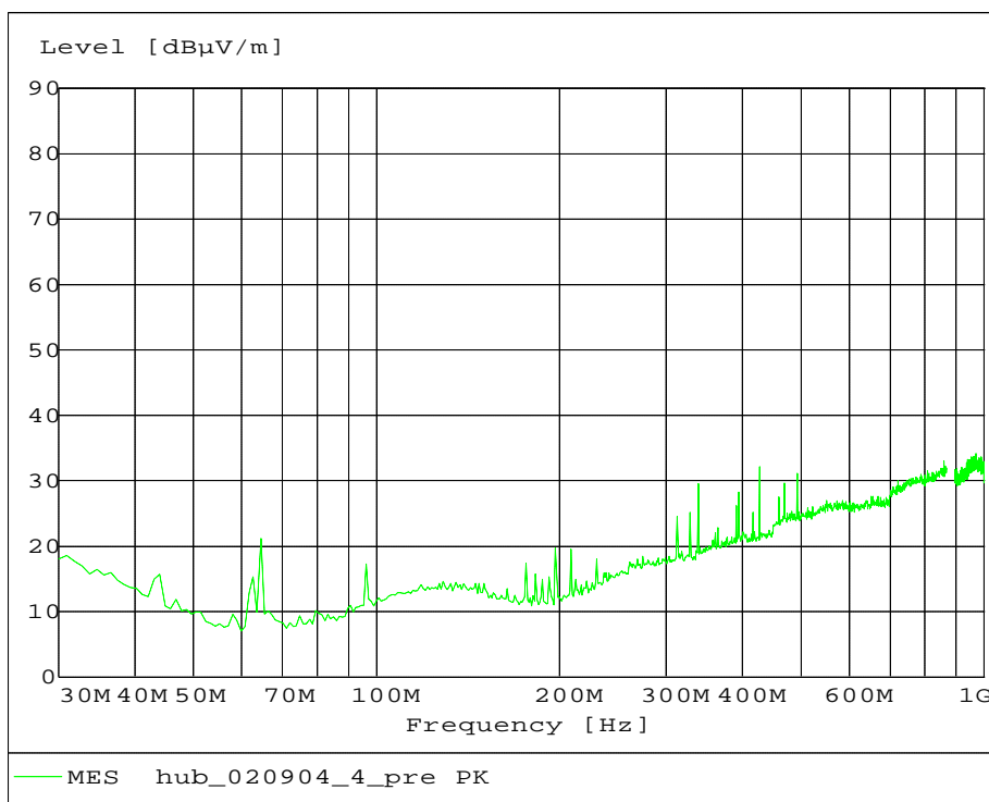
Fig. 96 – Radiated Emission 30 MHz – 1 GHz, 8PSK modulation.
