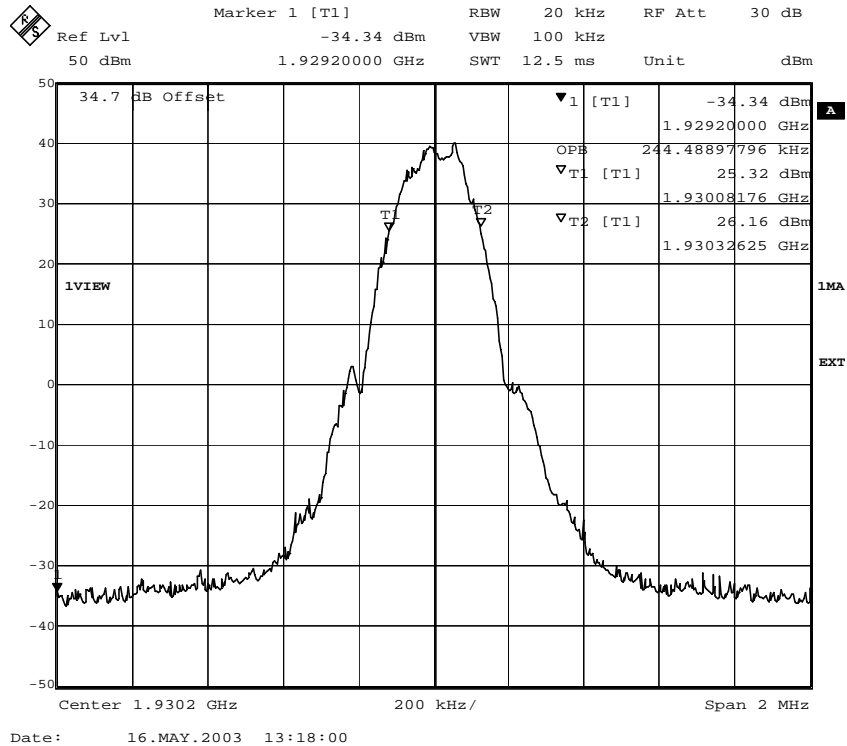
Fig. 25 – Occupied bandwidth (8PSK modulation).
