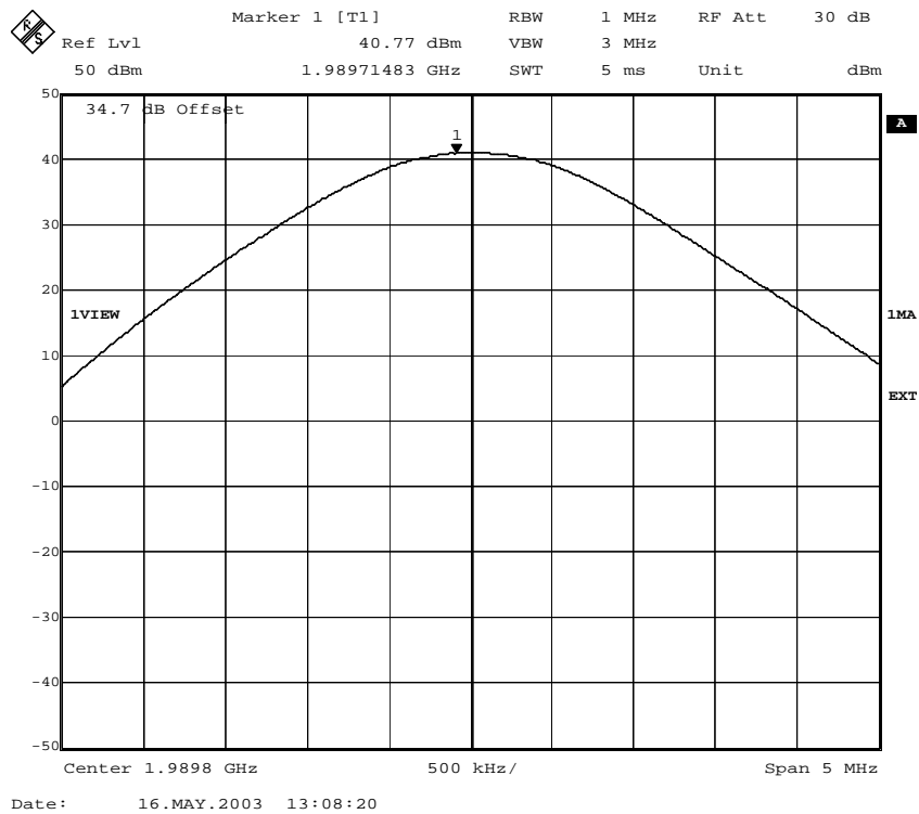
Fig. 20 – RF power at the antenna connector (GMSK modulation).
