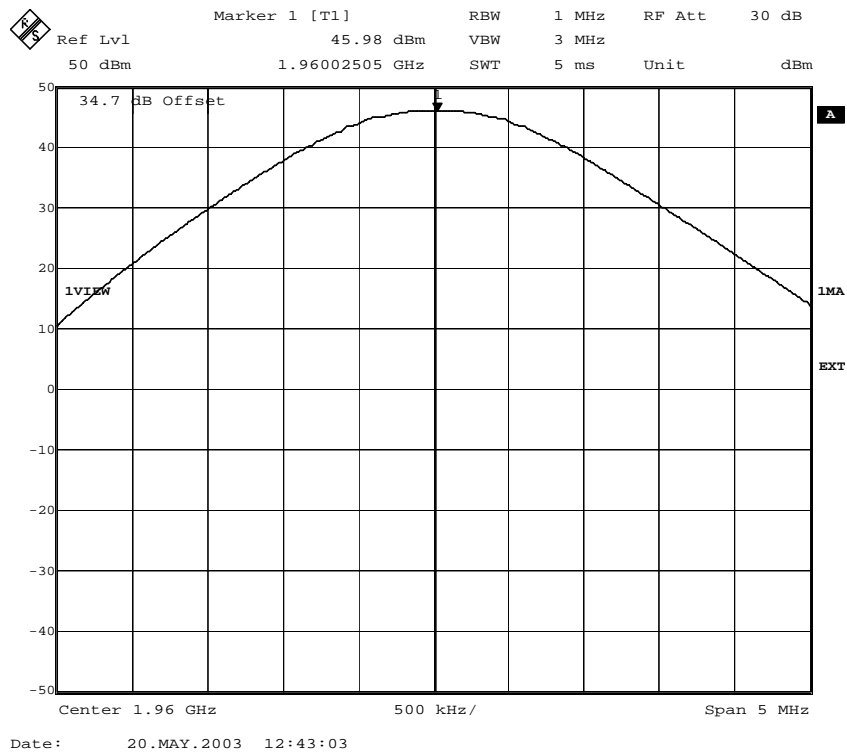
Fig. 14 – RF power at the antenna connector (GMSK modulation) for ECUPV2.
