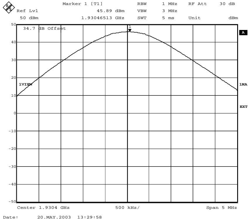
Fig. 11 – RF power at the antenna connector (8PSK modulation) for ECUPV2.
