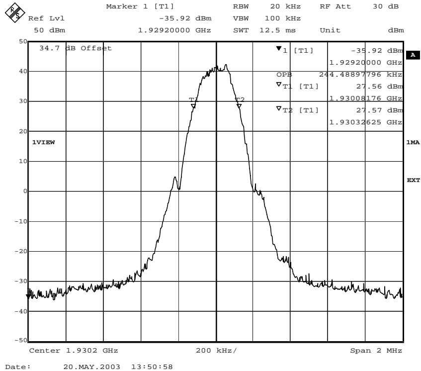
Fig. 27 – Occupied bandwidth (8PSK modulation) for ECUPV2.
