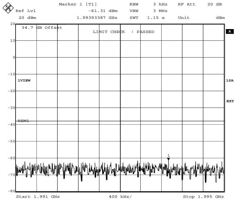
Fig. 54 – Spurious emissions in the frequency range 1991 MHz – 1995 MHz (GMSK modulation). Limit: -13dBm-25.2dB=-38.2dBm
