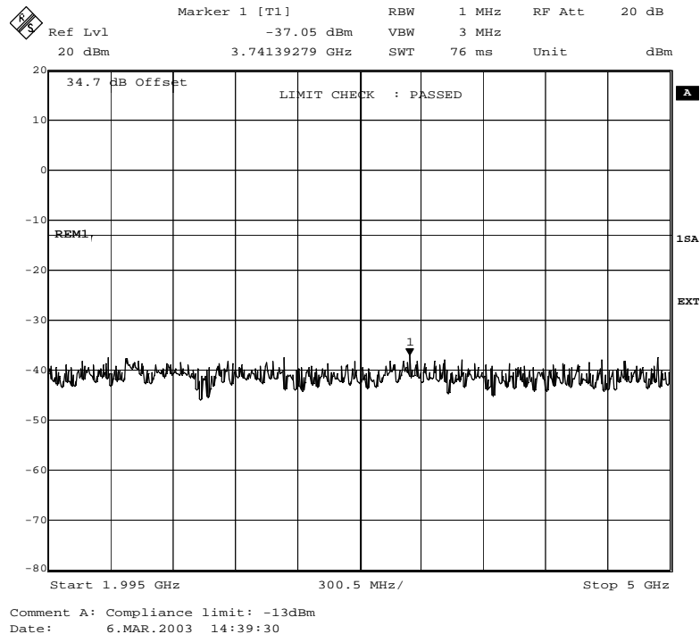
Fig. 57 – Spurious emissions in the frequency range 1995 MHz – 5000 MHz (8PSK modulation).
