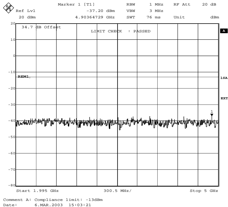
Fig. 56 – Spurious emissions in the frequency range 1995 MHz – 5000 MHz (GMSK modulation).
