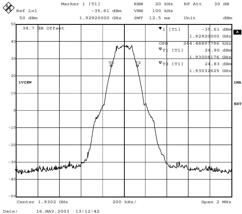
Fig. 24 – Occupied bandwidth (GMSK modulation).
