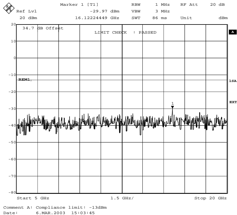
Fig. 58 – Spurious emissions in the frequency range 5000 MHz–20000 MHz (GMSK modulation).
