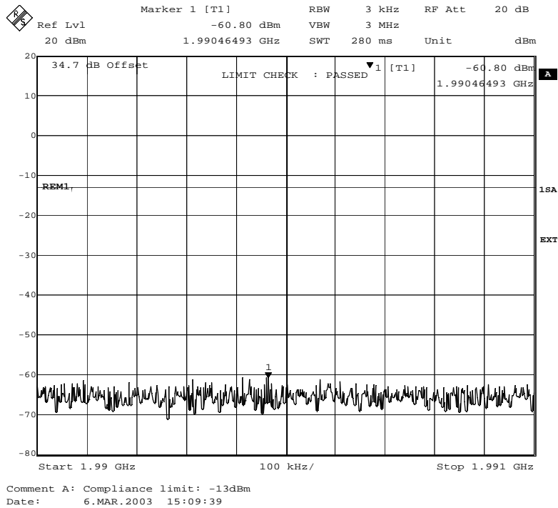
Fig. 66 – Spurious emissions in the frequency range 1990 MHz – 1991 MHz (GMSK modulation).
