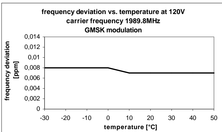
Fig. 106 – Frequency deviation vs. temperature (120V, 1989.8 MHz, GMSK modulation)
