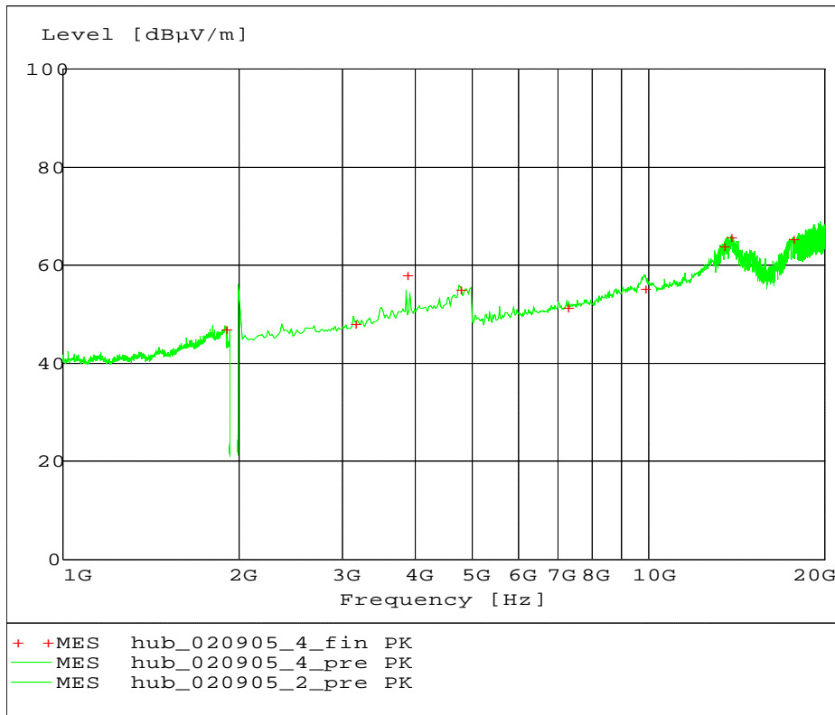
Fig. 97 – Radiated Emission 1 GHz – 20 GHz, GMSK modulation.
