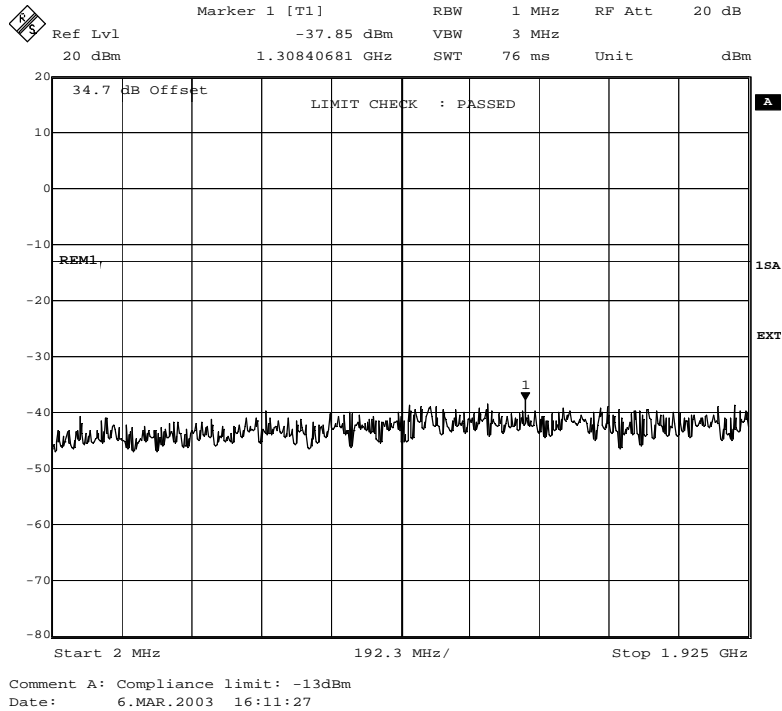
Fig. 75 – Spurious emissions in the frequency range 2 MHz – 1925 MHz (8PSK modulation).
