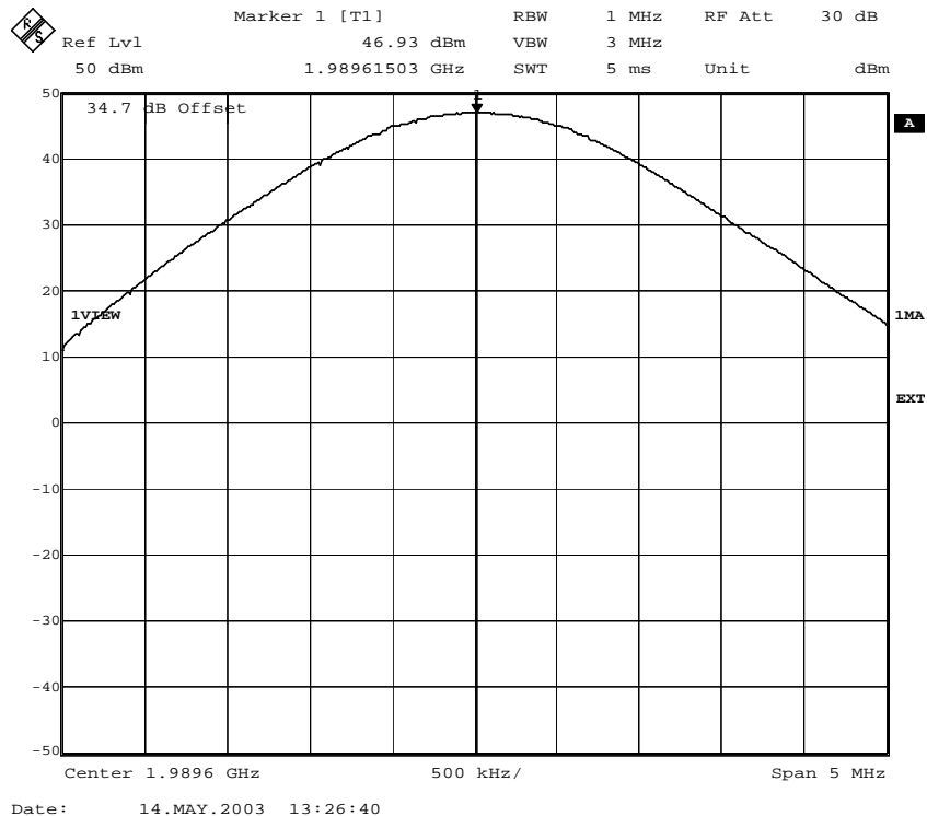
Fig. 17 – RF power at the antenna connector (8PSK modulation).
