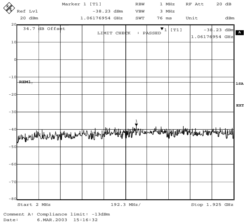
Fig. 61 – Spurious emissions in the frequency range 2 MHz – 1925 MHz (8PSK modulation).
