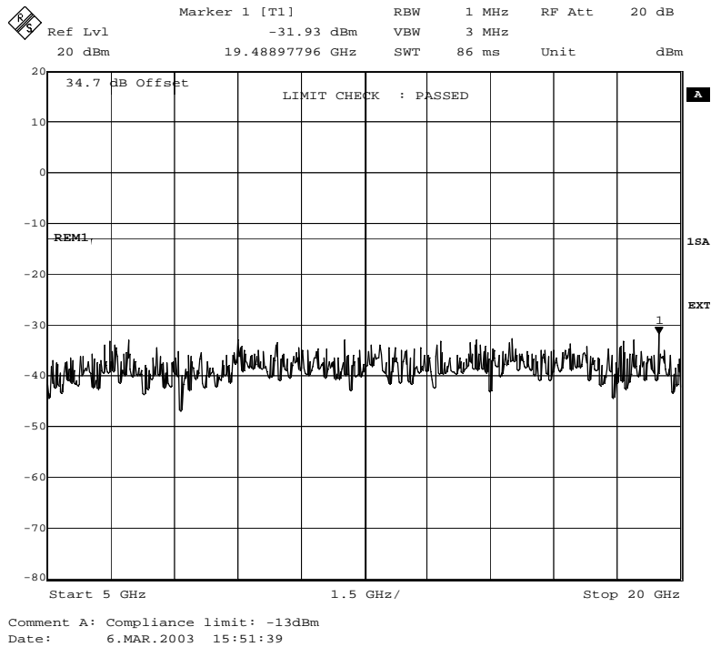
Fig. 88 – Spurious emissions in the frequency range 5000 MHz–20000 MHz (GMSK modulation).
