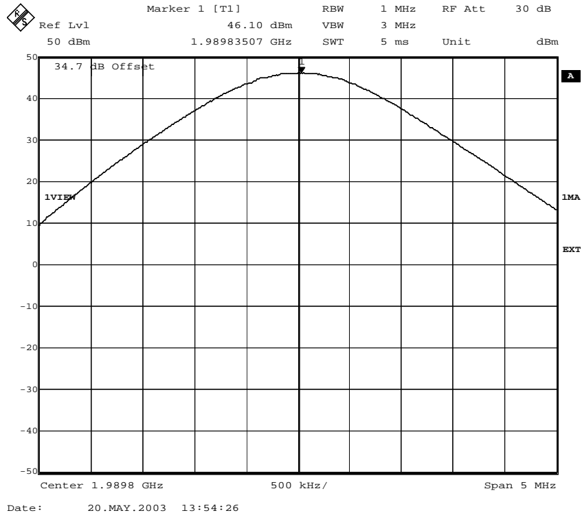
Fig. 23 – RF power at the antenna connector (8PSK modulation) for ECUPV2.
