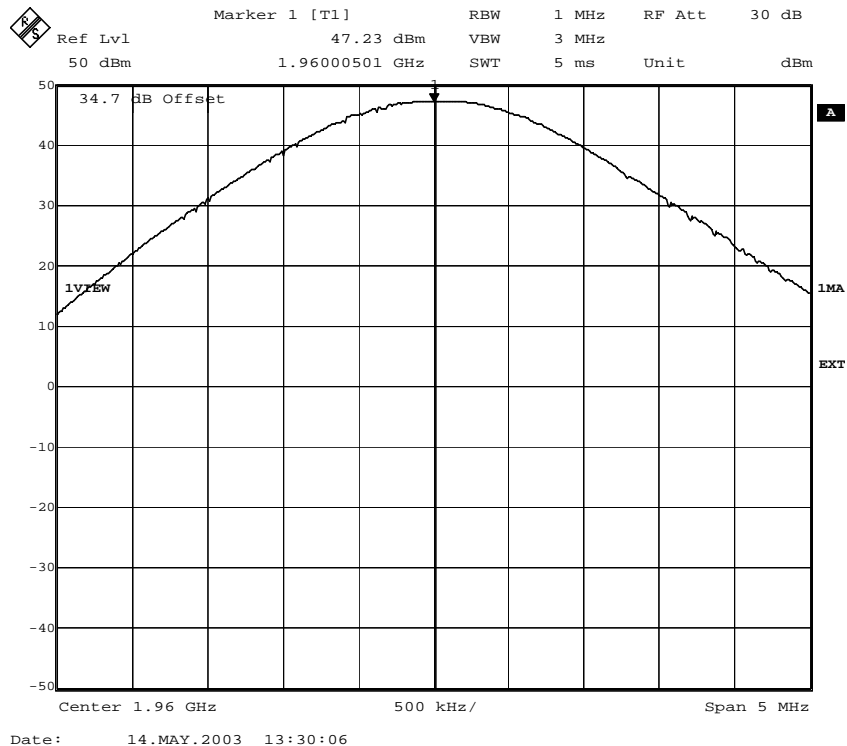
Fig. 13 – RF power at the antenna connector (8PSK modulation).
