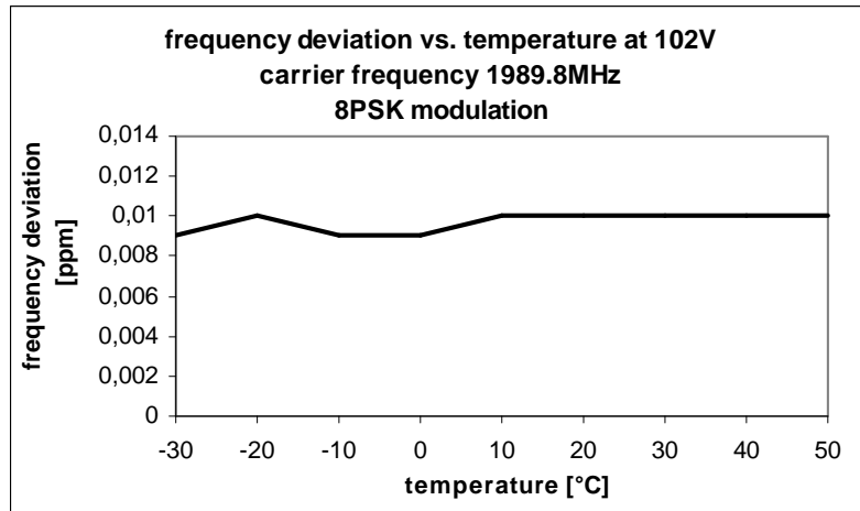
Fig. 108 – Frequency deviation vs. temperature (102V, 1989.8 MHz, 8PSK modulation)
