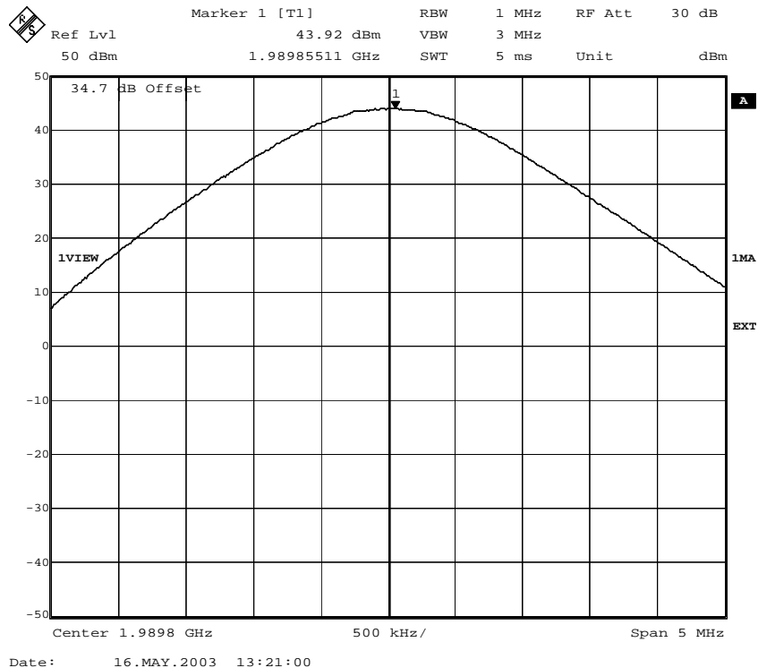
Fig. 21 – RF power at the antenna connector (8PSK modulation).
