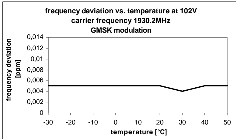
Fig. 99 – Frequency deviation vs. temperature (102V, 1930.2 MHz, GMSK modulation)
