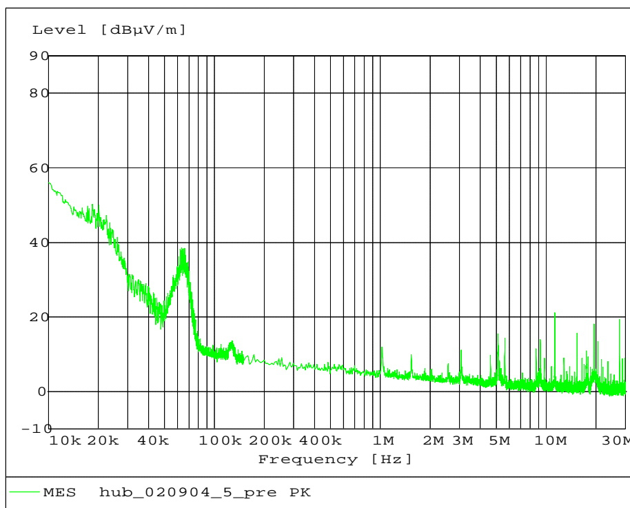
Fig. 94 – Radiated Emission 10 kHz – 30 MHz, 8PSK modulation.
