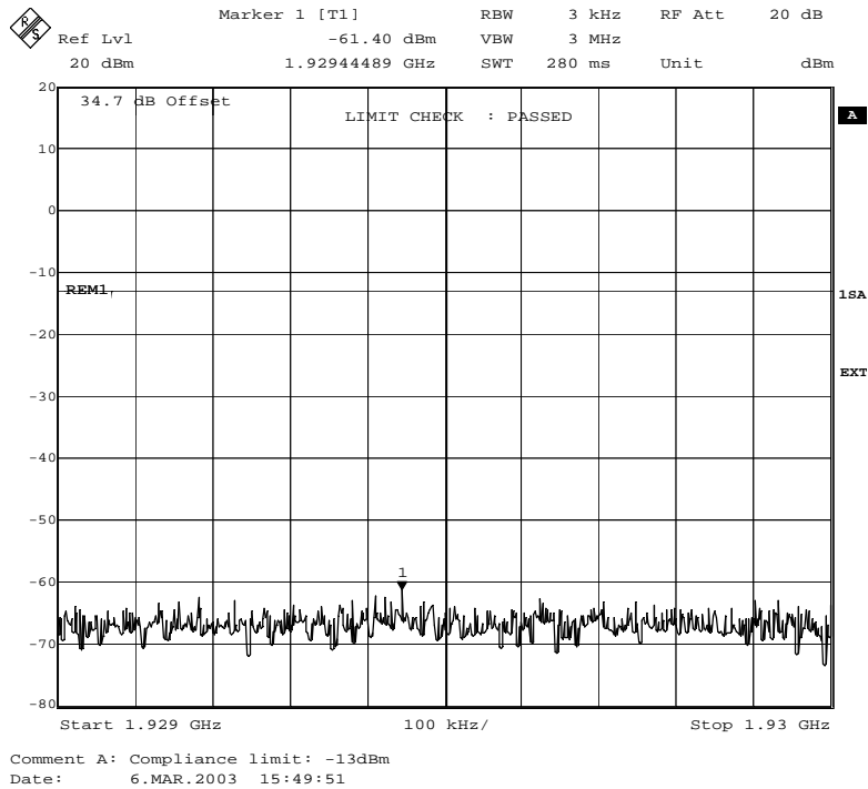
Fig. 78 – Spurious emissions in the frequency range 1929 MHz – 1930 MHz (GMSK modulation).
