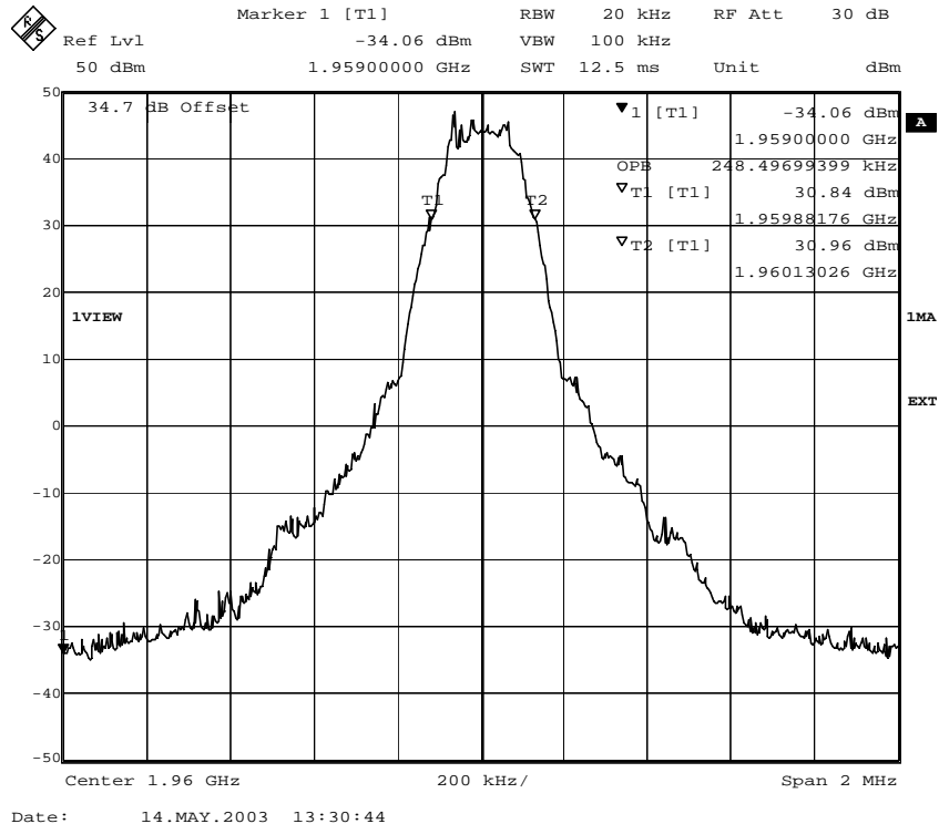
Fig. 33 – Occupied bandwidth (8PSK modulation).
