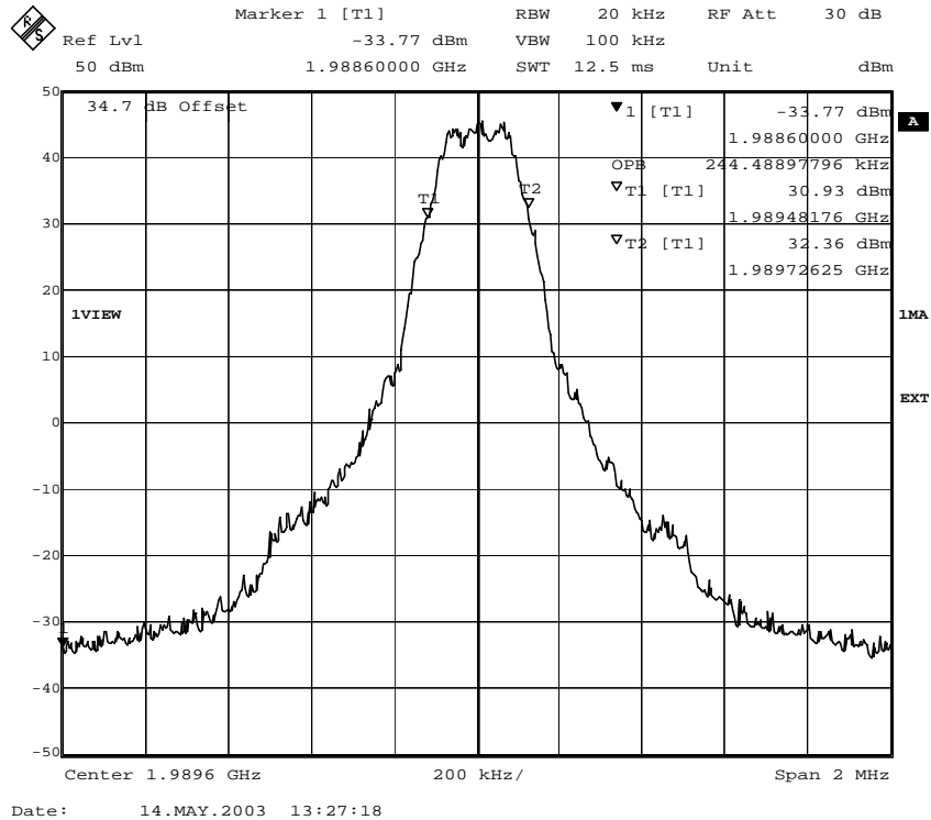
Fig. 37 – Occupied bandwidth (8PSK modulation).
