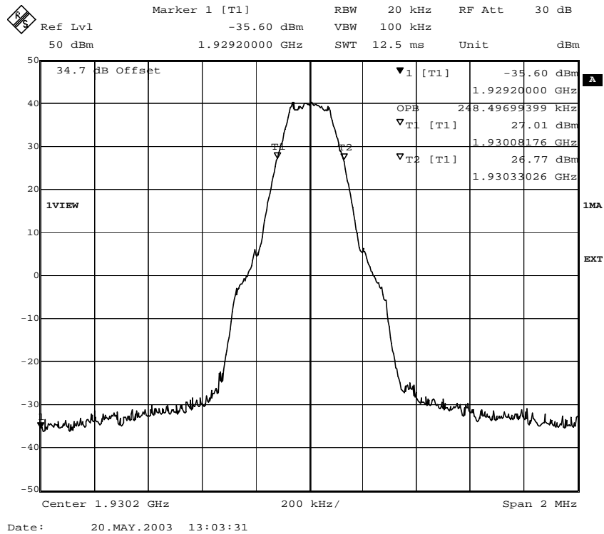
Fig. 26 – Occupied bandwidth (GMSK modulation) for ECUPV2.
