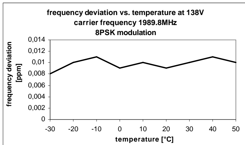
Fig. 110 – Frequency deviation vs. temperature (138V, 1989.8 MHz, 8PSK modulation)
