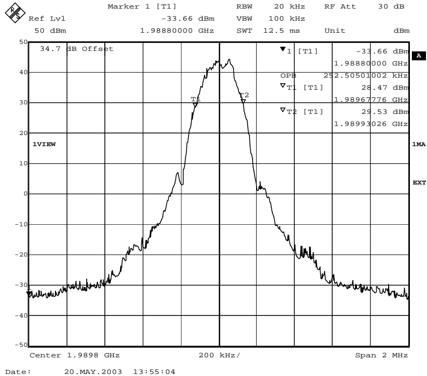
Fig. 43 – Occupied bandwidth (8PSK modulation) for ECUPV2.
