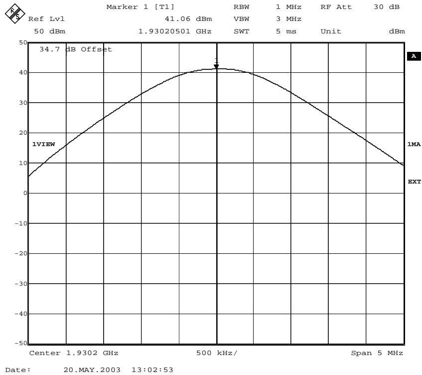
Fig. 6 – RF power at the antenna connector (GMSK modulation) for ECUPV2.
