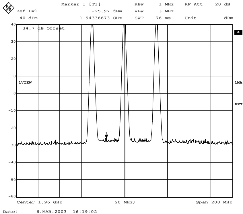
Fig. 112 – Slow frequency hopping – RBW = 1 MHz (8PSK modulation)
