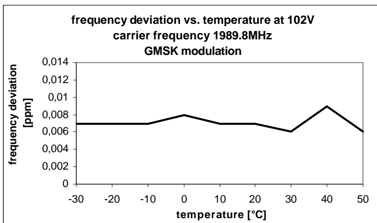
Fig. 105 – Frequency deviation vs. temperature (102V, 1989.8 MHz, GMSK modulation)
