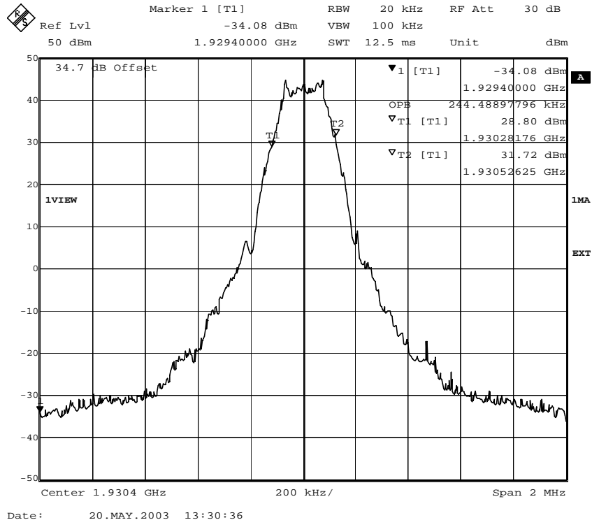
Fig. 31 – Occupied bandwidth (8PSK modulation) for ECUPV2.
