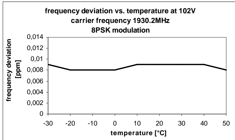
Fig. 102 – Frequency deviation vs. temperature (102V, 1930.2 MHz, 8PSK modulation)
