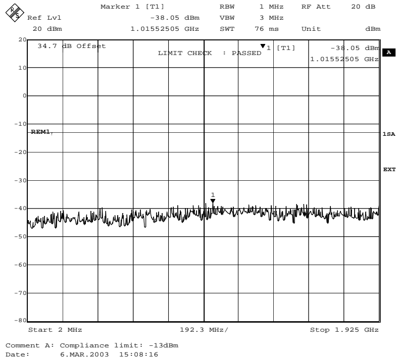
Fig. 60 – Spurious emissions in the frequency range 2 MHz – 1925 MHz (GMSK modulation).
