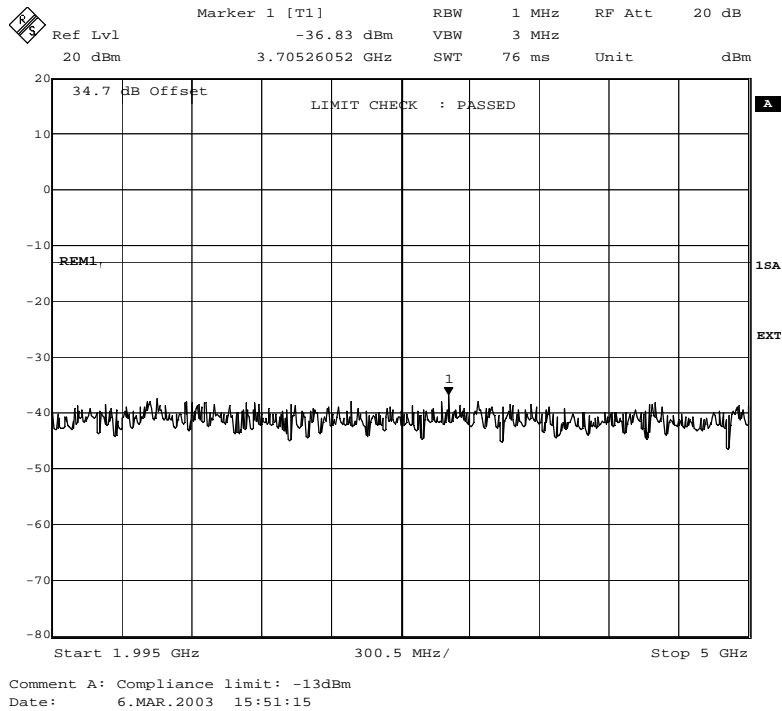
Fig. 86 – Spurious emissions in the frequency range 1995 MHz – 5000 MHz (GMSK modulation).
