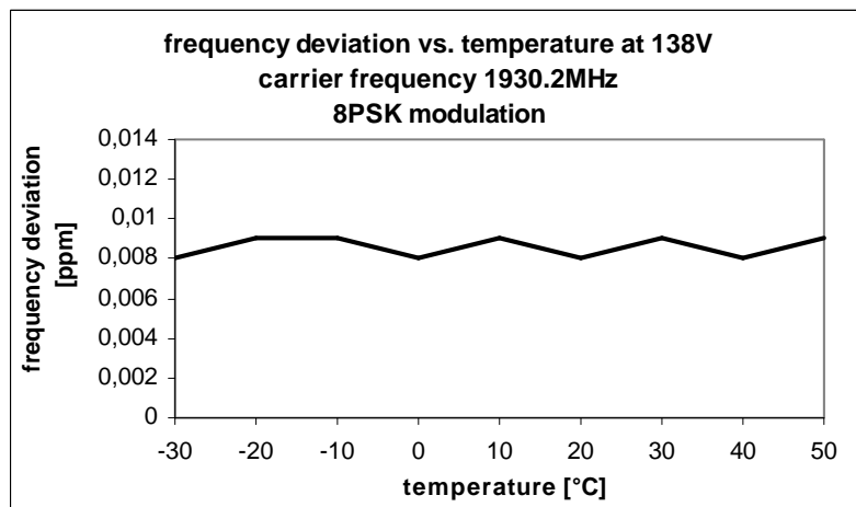
Fig. 104 – Frequency deviation vs. temperature (138V, 1930.2 MHz, 8PSK modulation)
