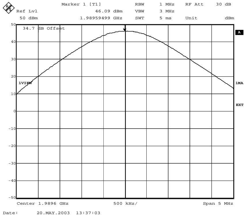
Fig. 19 – RF power at the antenna connector (8PSK modulation) for ECUPV2.
