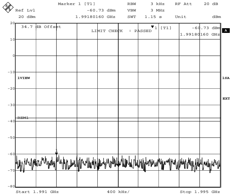
Fig. 68 – Spurious emissions in the frequency range 1991 MHz – 1995 MHz (GMSK modulation). Limit: -13dBm-25.2dB=-38.2dBm
