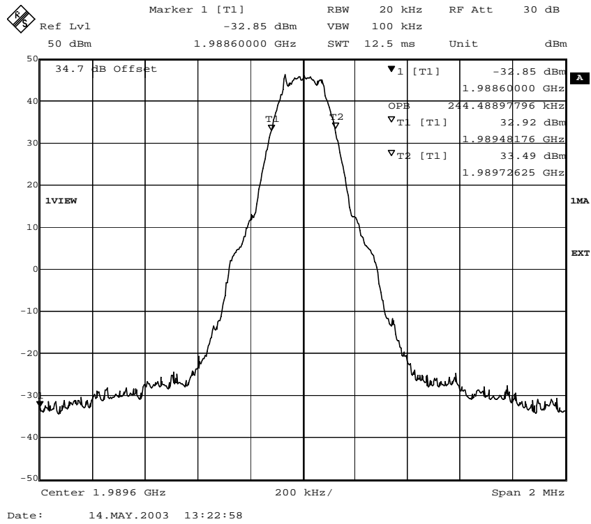
Fig. 36 – Occupied bandwidth (GMSK modulation).
