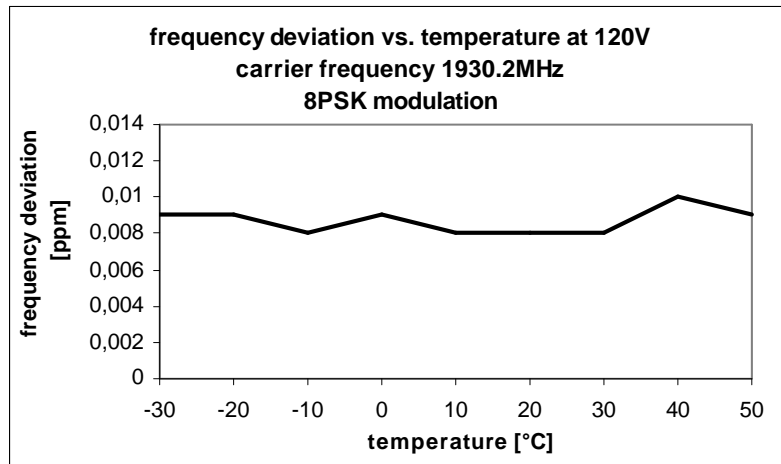
Fig. 103 – Frequency deviation vs. temperature (120V, 1930.2 MHz, 8PSK modulation)
