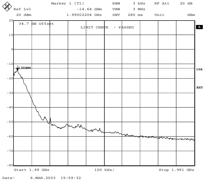
Fig. 80 – Spurious emissions in the frequency range 1990 MHz – 1991 MHz (GMSK modulation).
