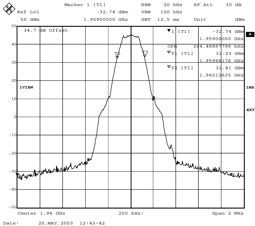
Fig. 34 – Occupied bandwidth (GMSK modulation) for ECUPV2.
