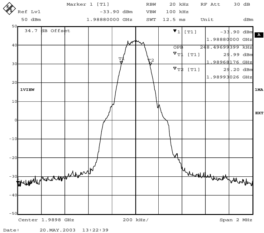
Fig. 42 – Occupied bandwidth (GMSK modulation) for ECUPV2.
