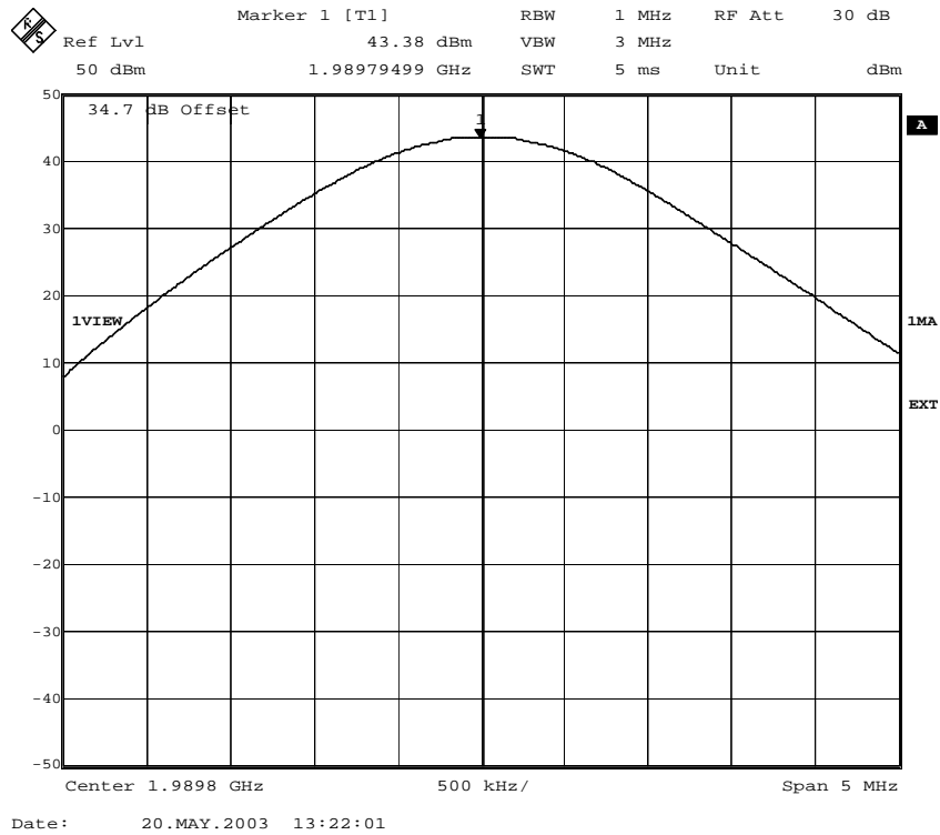
Fig. 22 – RF power at the antenna connector (GMSK modulation) for ECUPV2.
