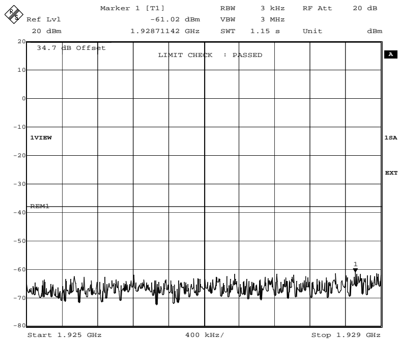
Fig. 46 – Spurious emissions in the frequency range 1925 MHz–1929 MHz (GMSK modulation). Limit: -13dBm–25.2dB=-38.2dBm
