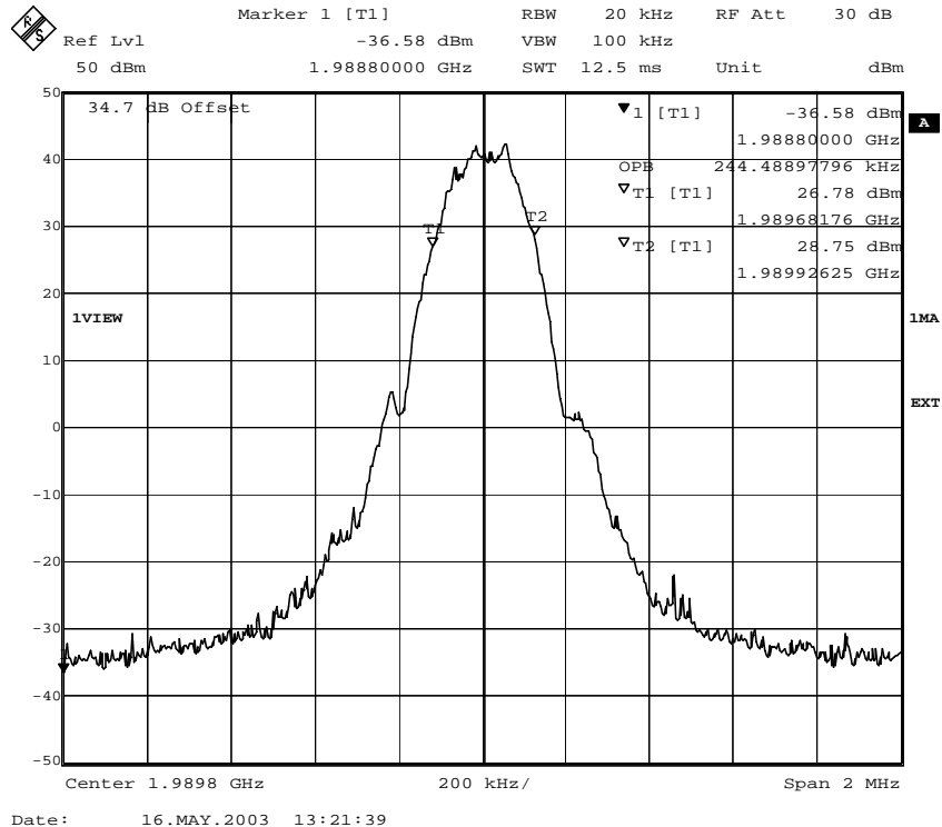
Fig. 41 – Occupied bandwidth (8PSK modulation).
