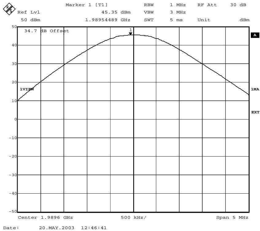
Fig. 18 – RF power at the antenna connector (GMSK modulation) for ECUPV2.
