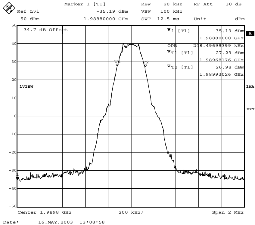
Fig. 40 – Occupied bandwidth (GMSK modulation).
