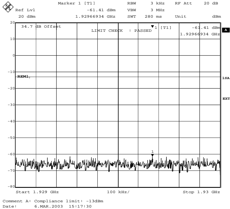
Fig. 65 – Spurious emissions in the frequency range 1929 MHz – 1930 MHz (8PSK modulation).
