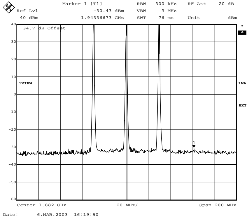
Fig. 114 – Slow frequency hopping – RBW = 300 kHz (8PSK modulation)
