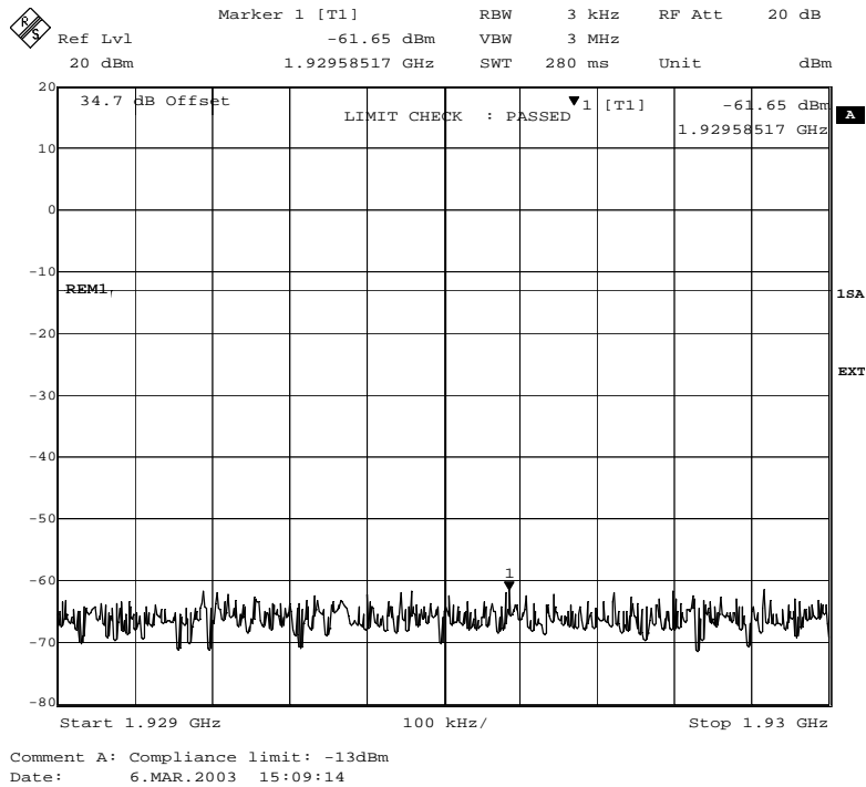
Fig. 64 – Spurious emissions in the frequency range 1929 MHz – 1930 MHz (GMSK modulation).
