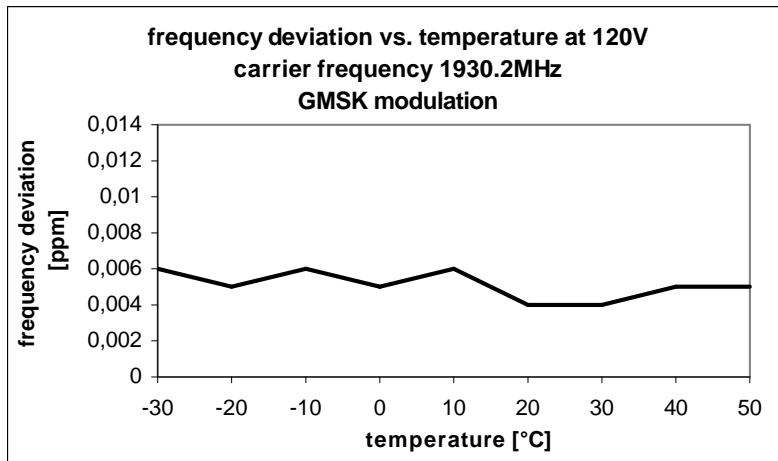
Fig. 100 – Frequency deviation vs. temperature (120V, 1930.2 MHz, GMSK modulation)
