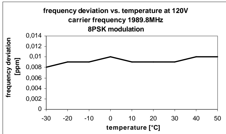
Fig. 109 – Frequency deviation vs. temperature (120V, 1989.8 MHz, 8PSK modulation)
