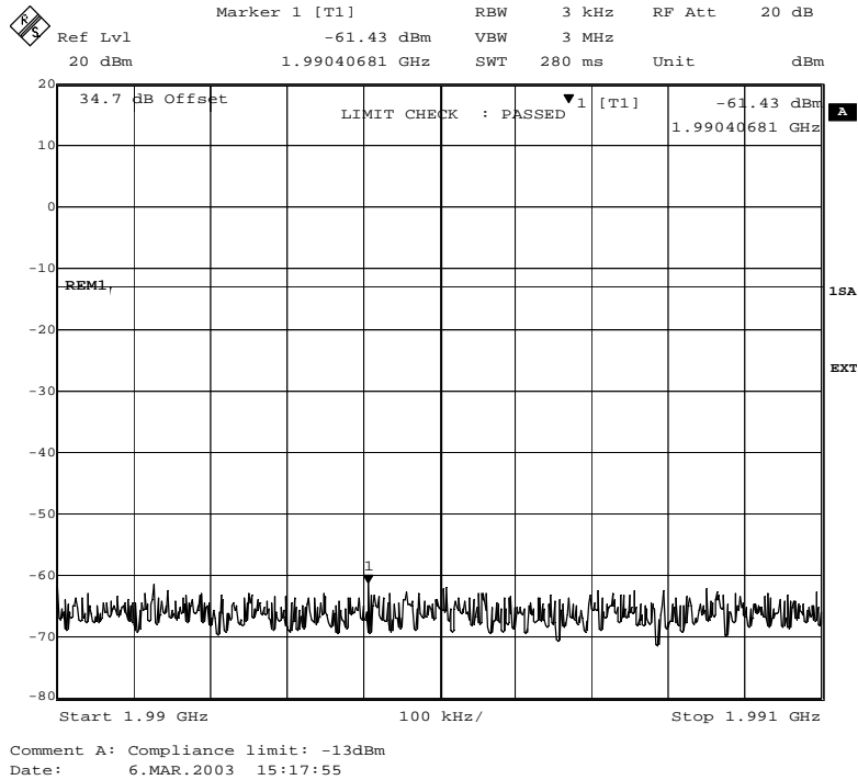
Fig. 67 – Spurious emissions in the frequency range 1990 MHz – 1991 MHz (8PSK modulation).
