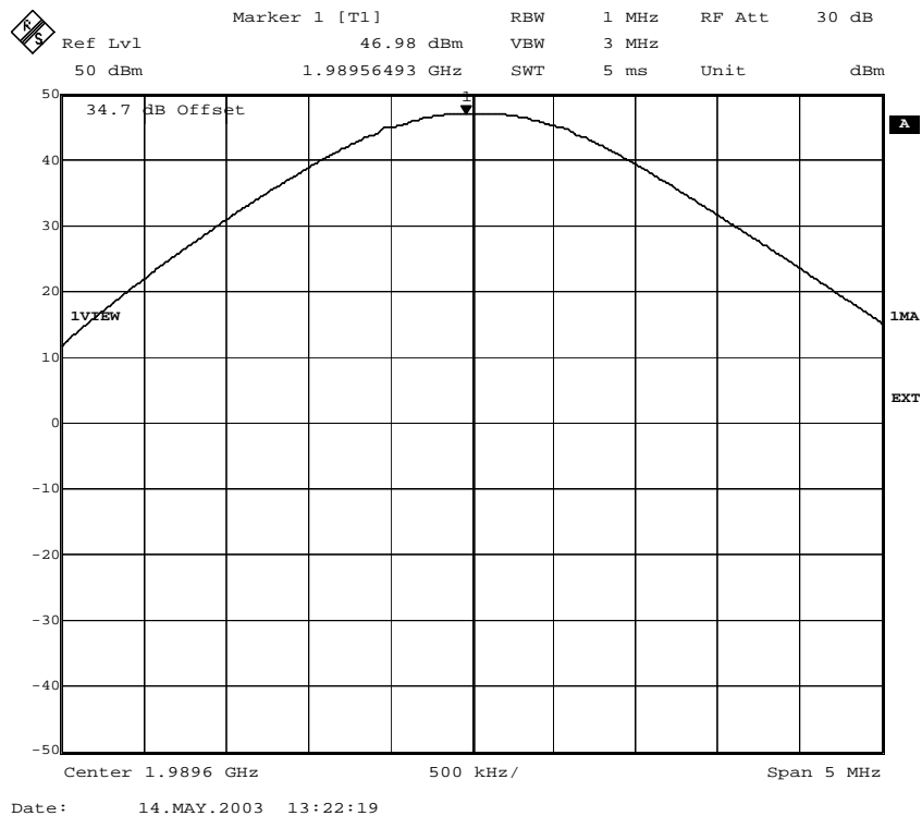
Fig. 16 – RF power at the antenna connector (GMSK modulation).
