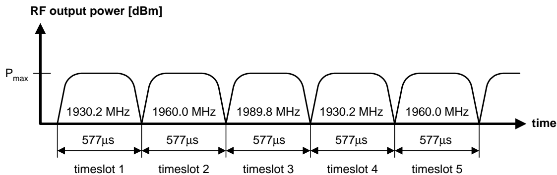
Fig. 3 – Slow frequency hopping (SFH) comprising 3 carrier test frequencies (1930.2 MHz, 1960.0 MHz, and 1989.8 MHz).
