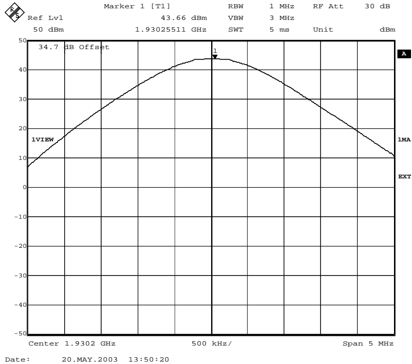
Fig. 7 – RF power at the antenna connector (8PSK modulation) for ECUPV2.
