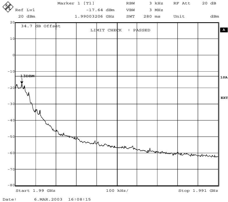
Fig. 81 – Spurious emissions in the frequency range 1990 MHz – 1991 MHz (8PSK modulation).
