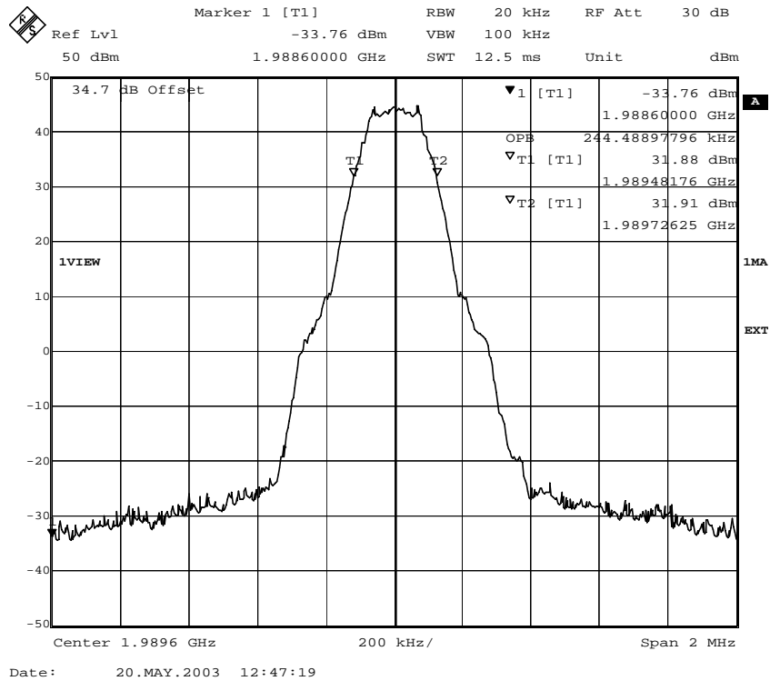
Fig. 38 – Occupied bandwidth (GMSK modulation) for ECUPV2.
