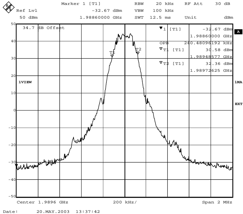
Fig. 39 – Occupied bandwidth (8PSK modulation) for ECUPV2.
