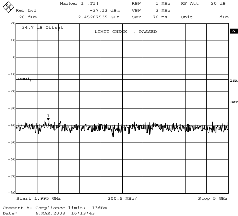
Fig. 87 – Spurious emissions in the frequency range 1995 MHz – 5000 MHz (8PSK modulation).
