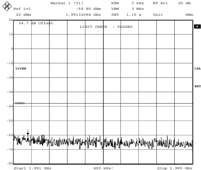
Fig. 84 – Spurious emissions in the frequency range 1991 MHz – 1995 MHz (GMSK modulation). Limit: -13dB–25.2dB–38.2dBm
