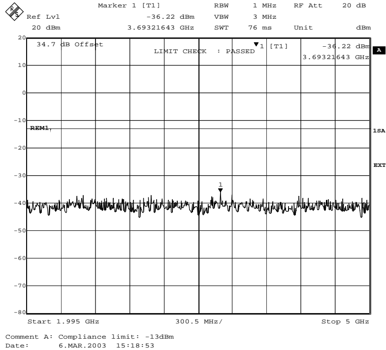
Fig. 71 – Spurious emissions in the frequency range 1995 MHz – 5000 MHz (8PSK modulation).
