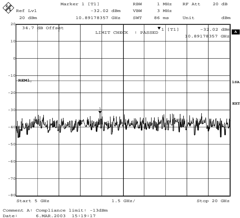
Fig. 73 – Spurious emissions in the frequency range 5000 MHz–20000 MHz (8PSK modulation).
