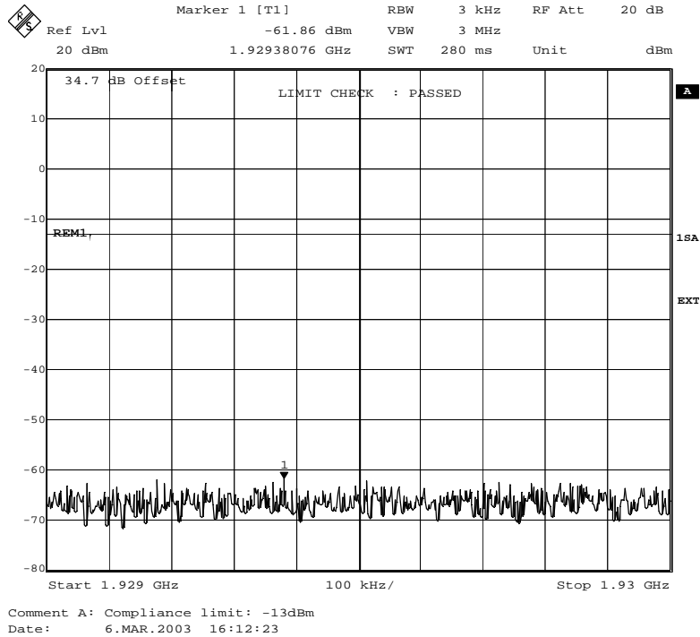
Fig. 79 – Spurious emissions in the frequency range 1929 MHz – 1930 MHz (8PSK modulation).
