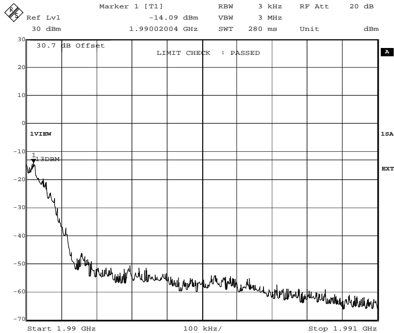
Fig. 82 – Spurious emissions in the frequency range 1990 MHz – 1991 MHz (GMSK modulation) for ECUPV2.
