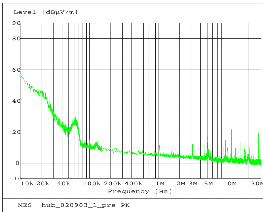
Fig. 93 – Radiated Emission 10 kHz – 30 MHz, GMSK modulation.
