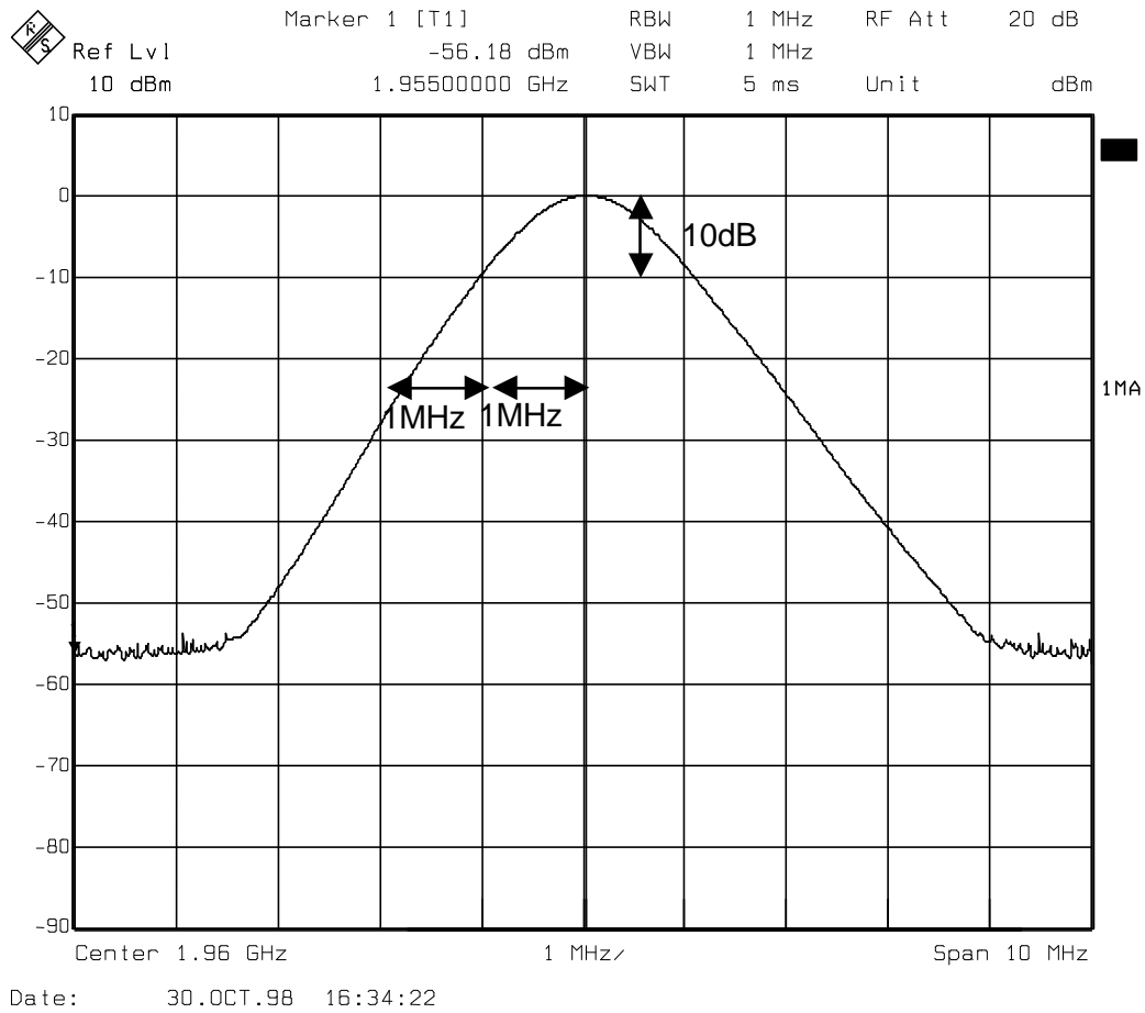
Fig. 90 – Filter characteristic of the 1 MHz resolution filter.
