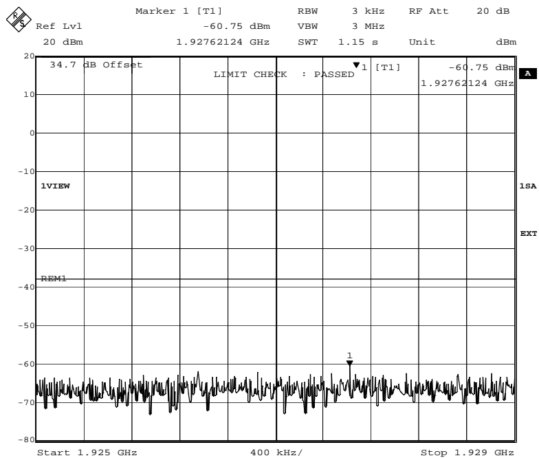
Fig. 62 – Spurious emissions in the frequency range 1925 MHz–1929 MHz (GMSK modulation). Limit: -13dBm–25.2dB=-38.2dBm
