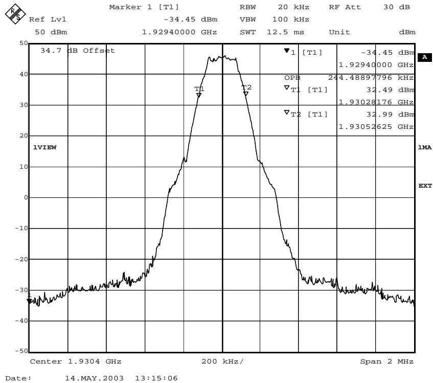
Fig. 28 – Occupied bandwidth (GMSK modulation).
