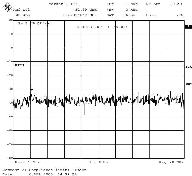
Fig. 59 – Spurious emissions in the frequency range 5000 MHz–20000 MHz (8PSK modulation).
