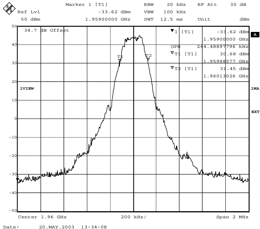
Fig. 35 – Occupied bandwidth (8PSK modulation) for ECUPV2.
