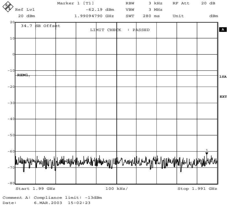
Fig. 52 – Spurious emissions in the frequency range 1990 MHz – 1991 MHz (GMSK modulation).
