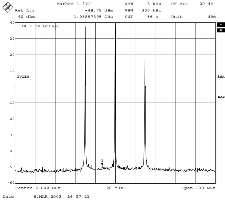
Fig. 117 – Slow frequency hopping – RBW = 3 kHz, reduced video bandwidth VBW = 300kHz (GMSK modulation)
