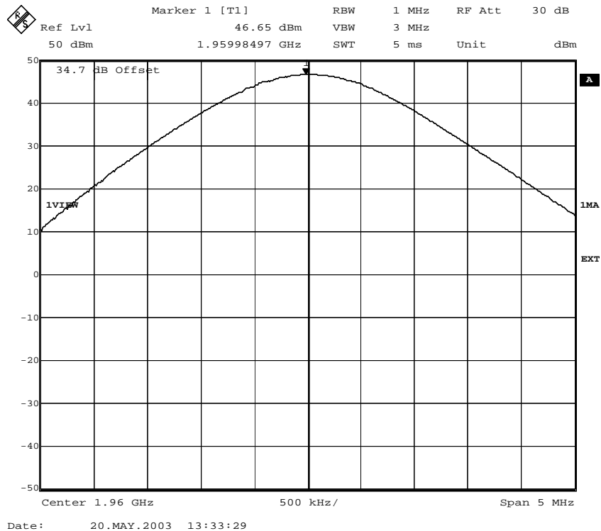
Fig. 15 – RF power at the antenna connector (8PSK modulation) for ECUPV2.
