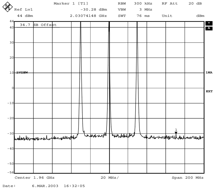
Fig. 113 – Slow frequency hopping – RBW = 300 kHz (GMSK modulation)
