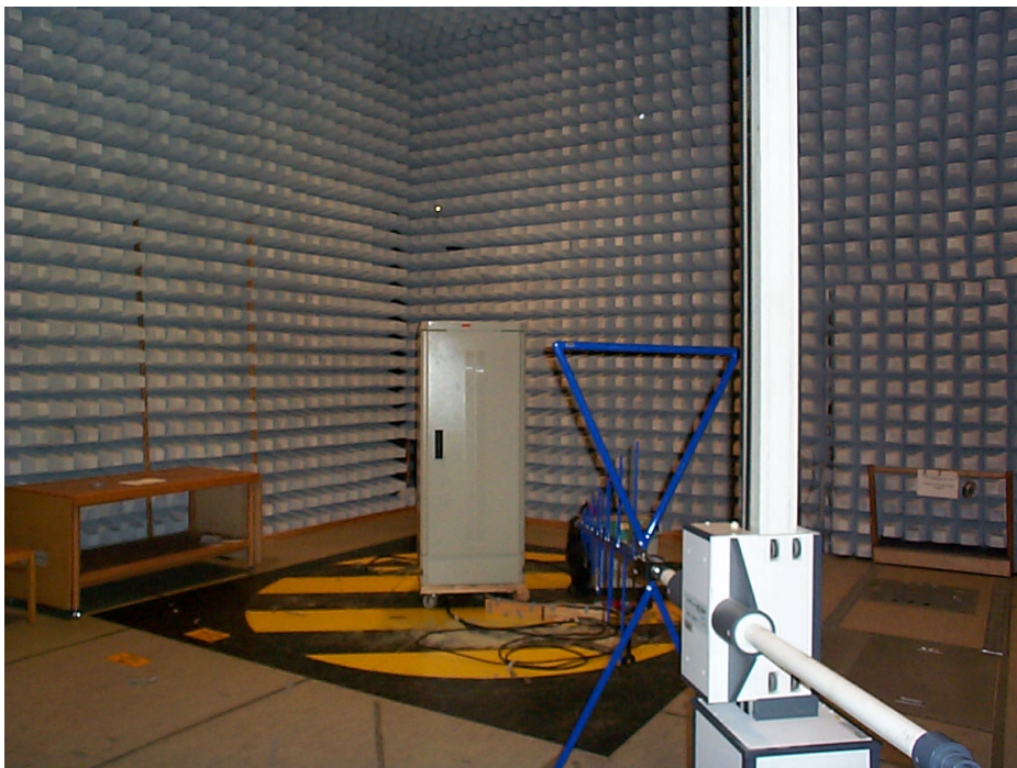
Fig. 91 -- Test setup for radiated emission measurement, 10 kHz to 30 MHz
