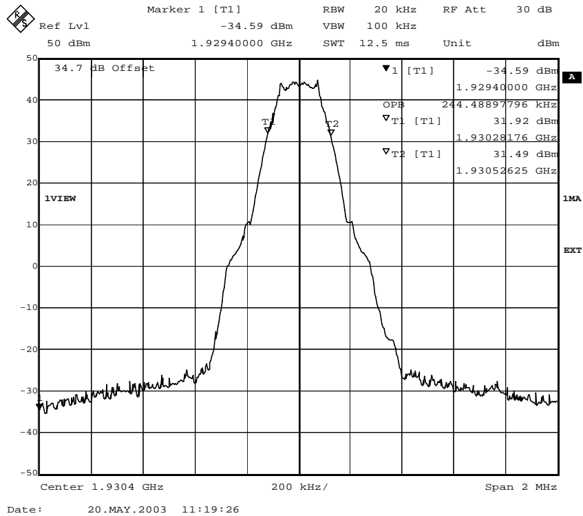
Fig. 30 – Occupied bandwidth (GMSK modulation) for ECUPV2.
