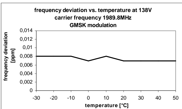
Fig. 107 – Frequency deviation vs. temperature (138V, 1989.8 MHz, GMSK modulation)
