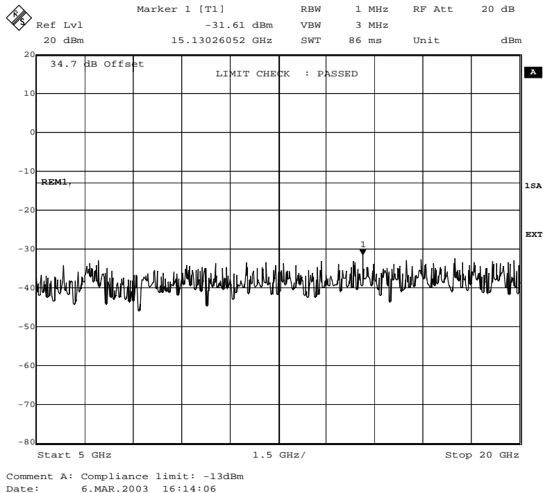
Fig. 89 – Spurious emissions in the frequency range 5000 MHz–20000 MHz (8PSK modulation).
