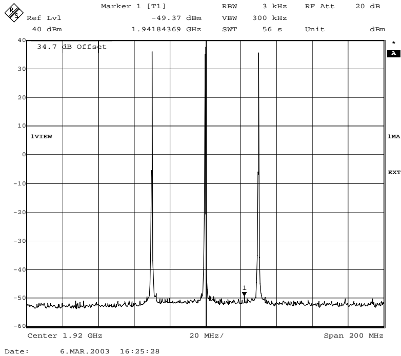
Fig. 118 – Slow frequency hopping – RBW = 3 kHz, reduced video bandwidth VBW = 300kHz (8PSK modulation)
