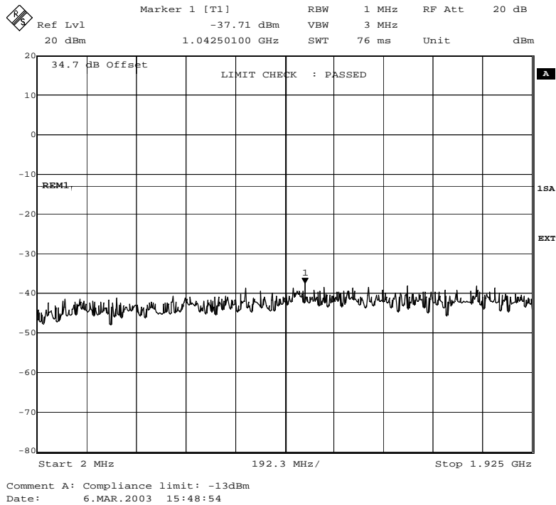
Fig. 74 – Spurious emissions in the frequency range 2 MHz – 1925 MHz (GMSK modulation).
