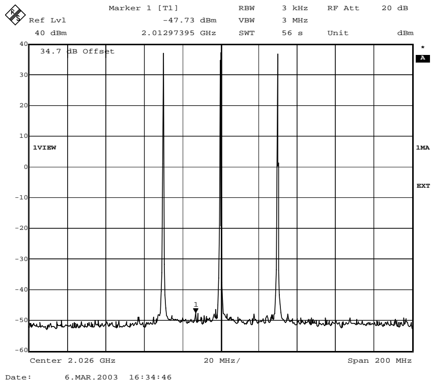
Fig. 115 – Slow frequency hopping – RBW = 3 kHz (GMSK modulation)
