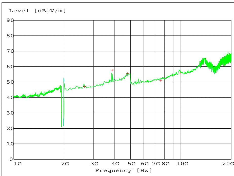
Fig. 98 – Radiated Emission 1 GHz – 20 GHz, 8PSK modulation.
