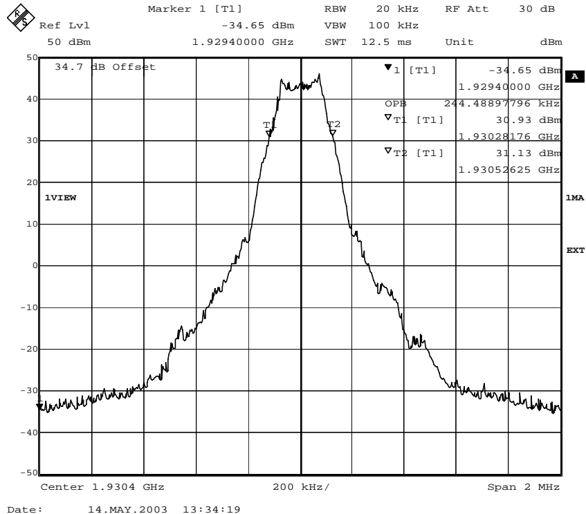
Fig. 29 – Occupied bandwidth (8PSK modulation).
