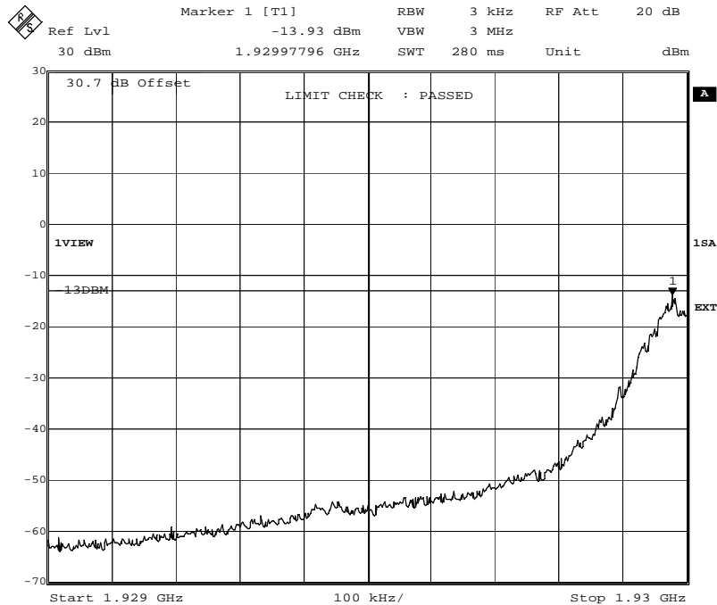
Fig. 50 – Spurious emissions in the frequency range 1929 MHz – 1930 MHz (GMSK modulation) for ECUPV2.
