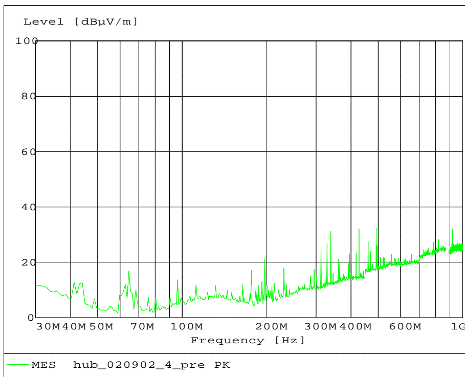
Fig. 95 – Radiated Emission 30 MHz – 1 GHz, GMSK modulation.
