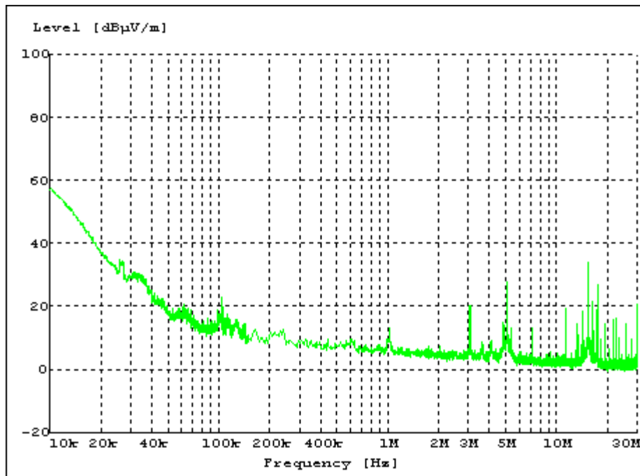
Fig. 36 – Radiated Emission 10 kHz – 30 MHz, GSM modulation.
