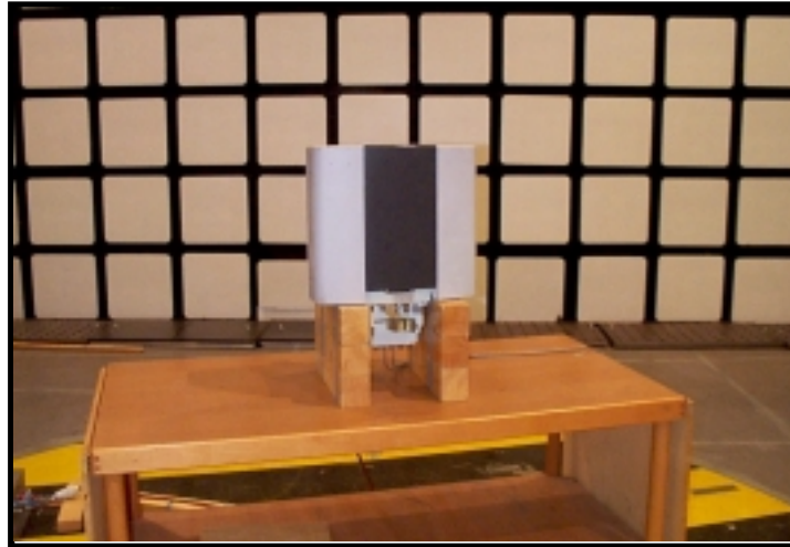
Fig. 1 -- Photograph of the anechoic chamber with the EUT.
