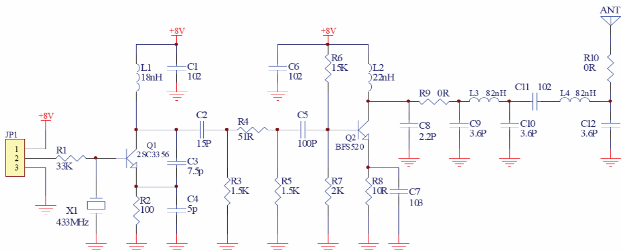
Schematic of transmission module
