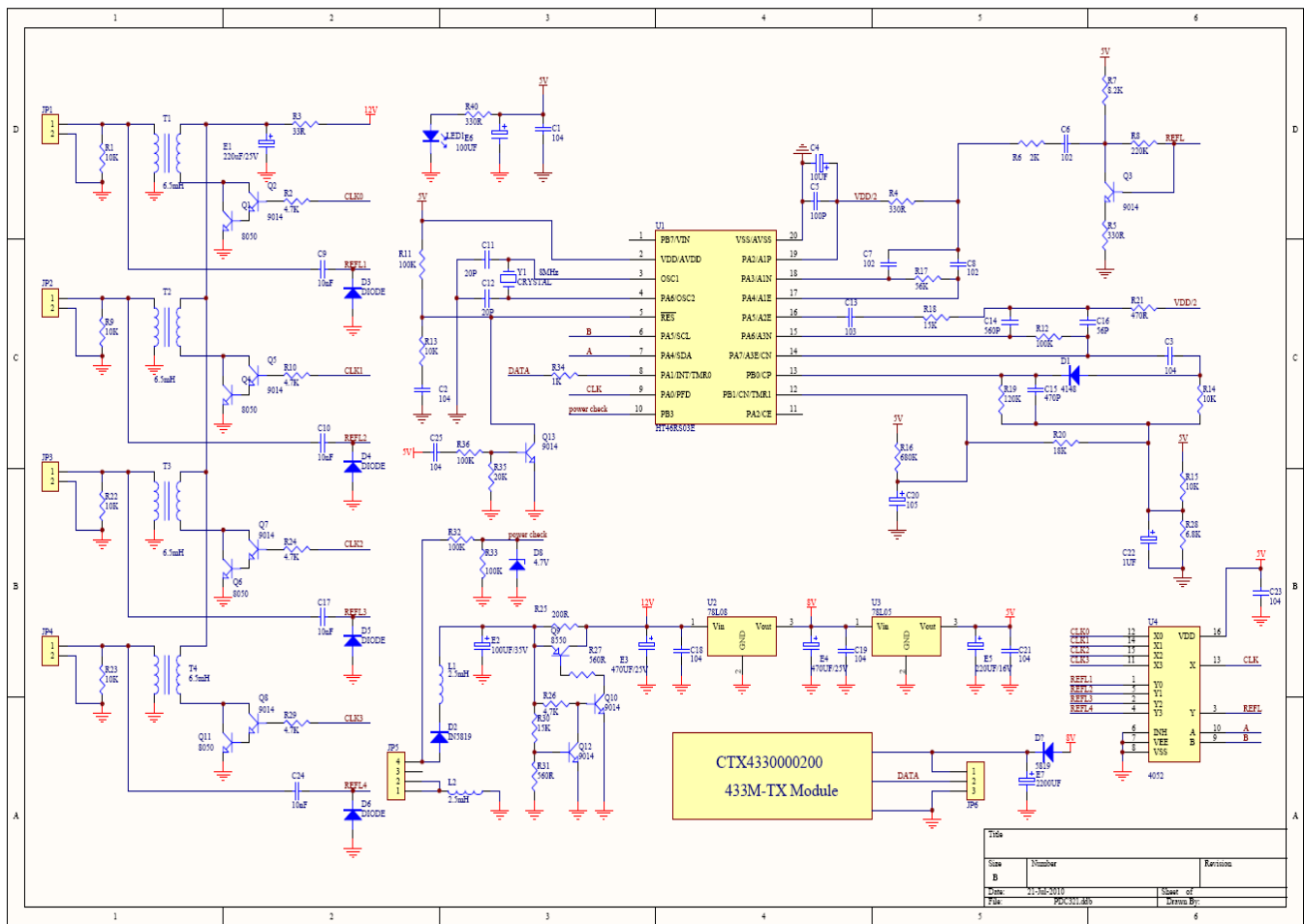
Schematic of transmission module
