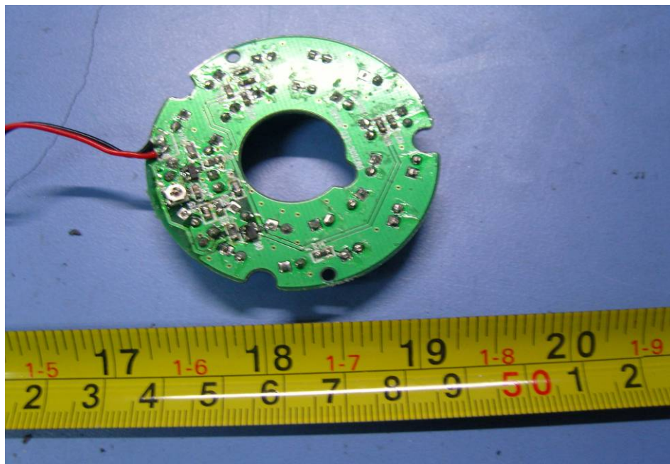
16.17 PCB5- Back View
