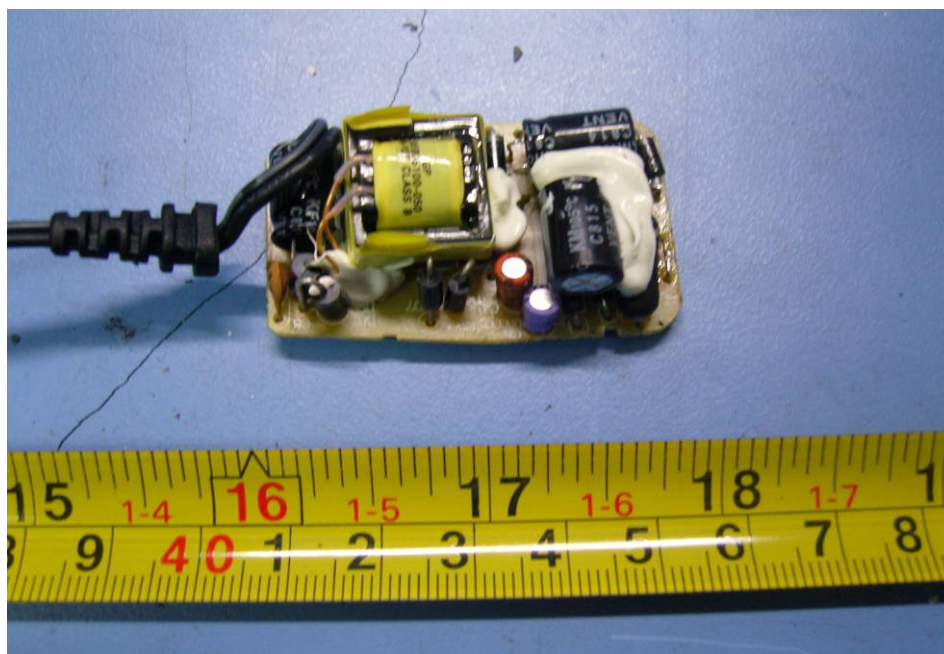
16.18 Adapter - Front View
