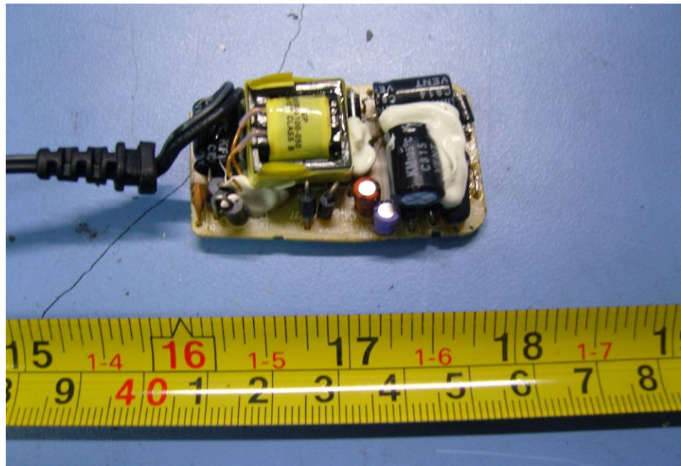
2.11 Adapter - Front View
