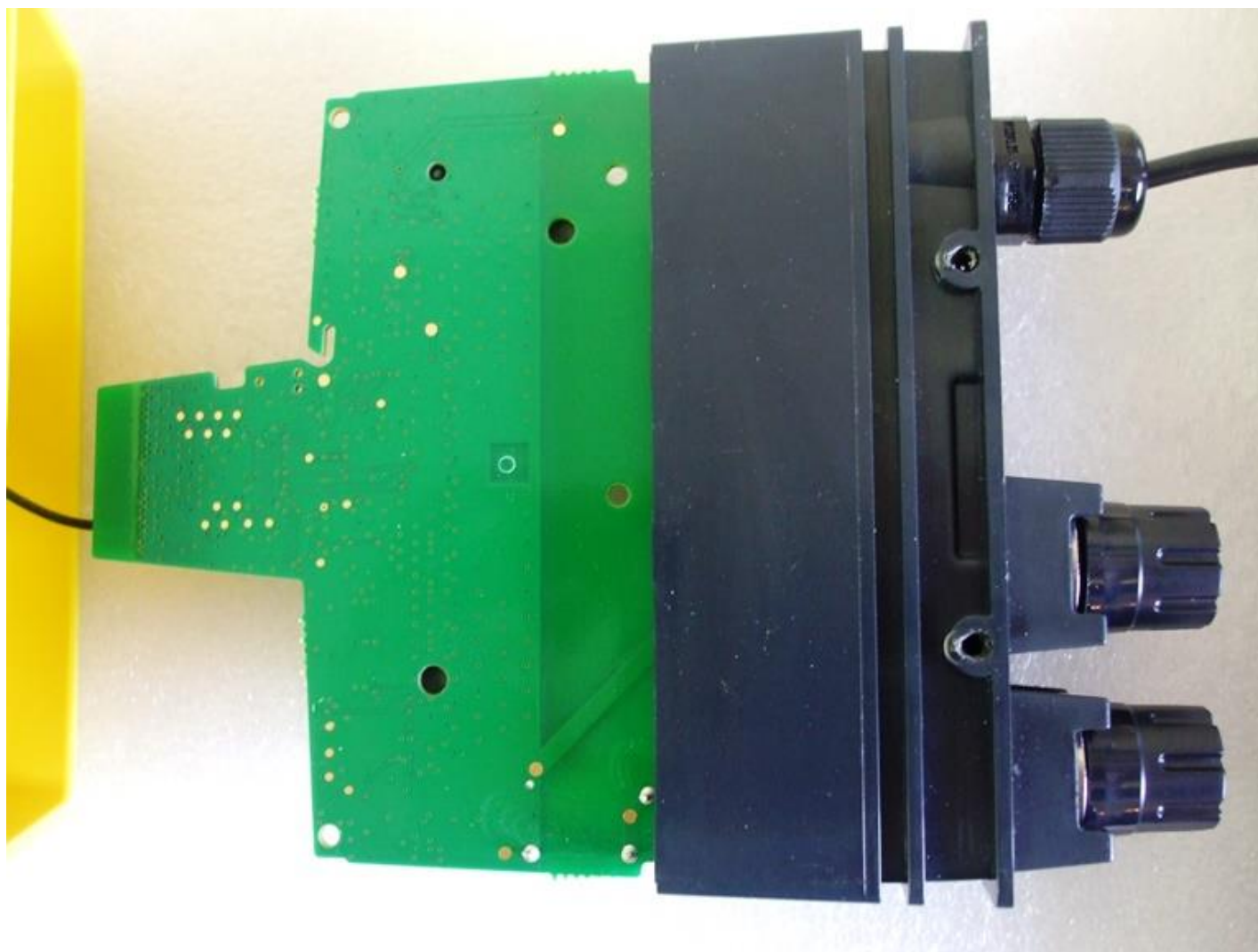
Trutest FN1F 4W Fence Monitoring Node, Rear side of PCB
