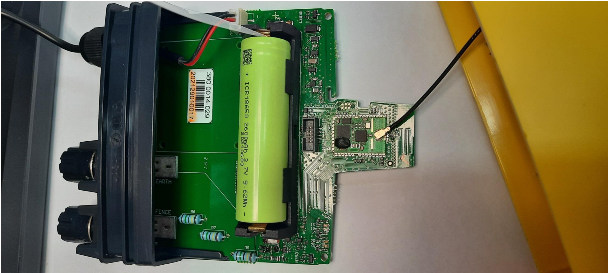
Internal Photo in host device: Trutest FN1F 4W Fence Monitoring Node
