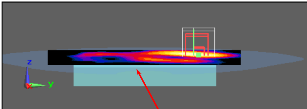
802.11b_Body SAR Test Setup (Flat Section)
