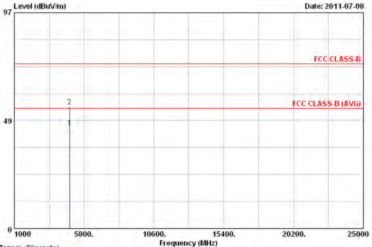
Trace: (Discrete)
