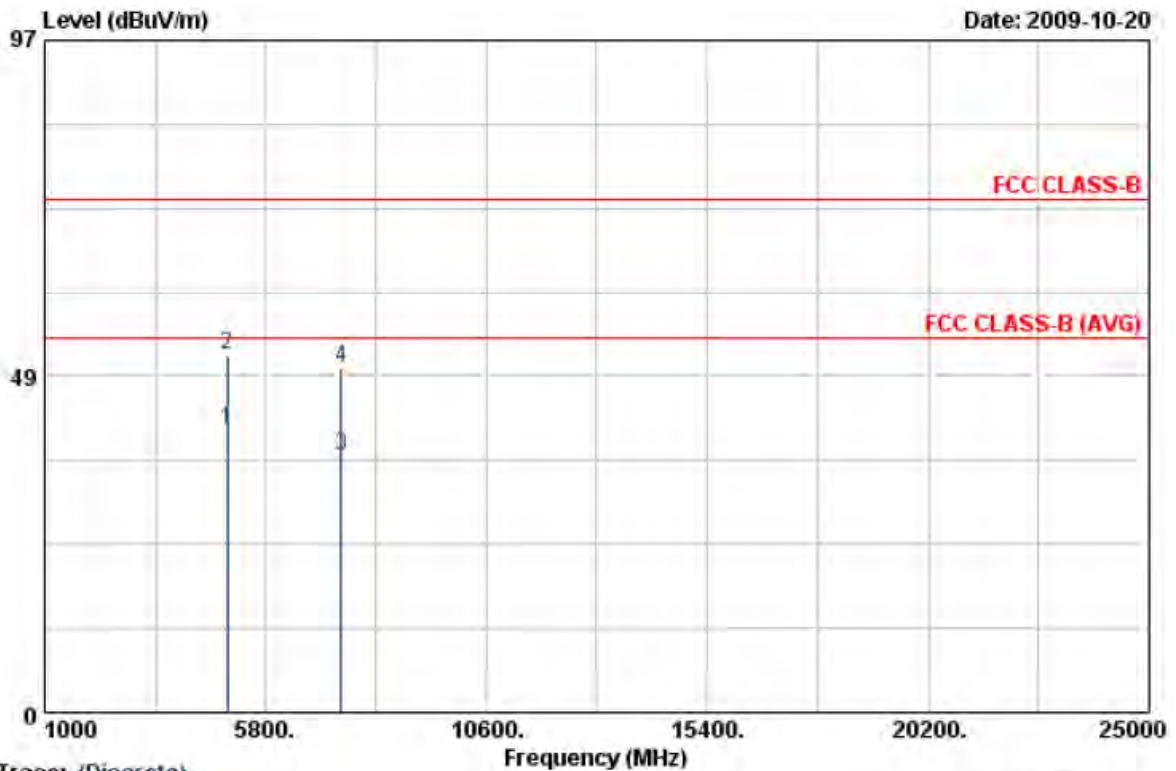
Trace: (Discrete)
