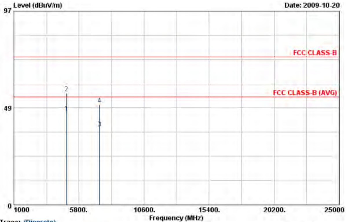
Trace: (Discrete)
