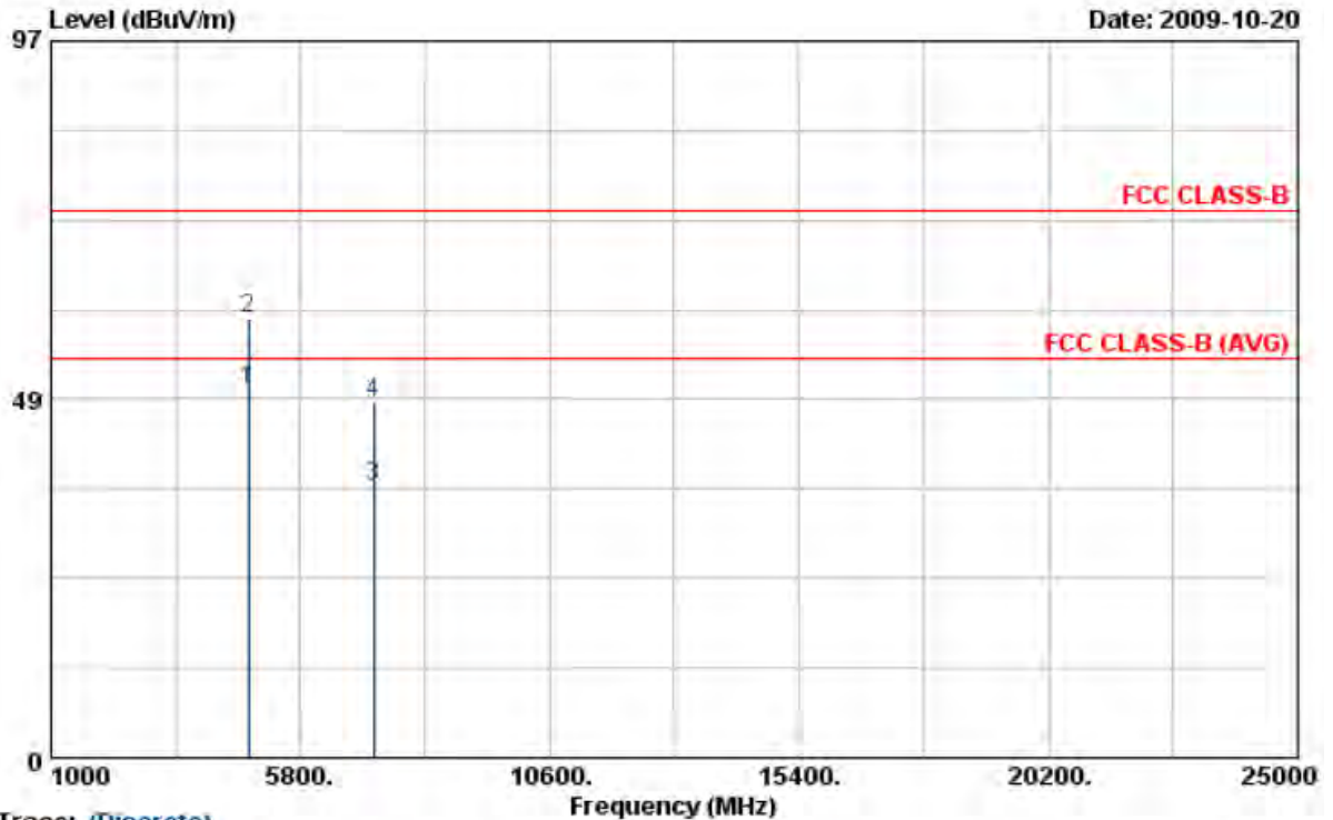
Trace: (Discrete)
