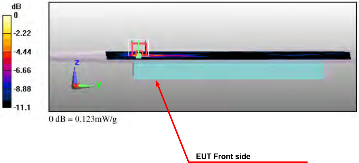
Figure 1. Body SAR Test Setup (Flat Section)
