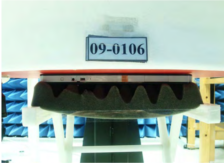
Figure 1. Body SAR Test Setup (Flat Section)
