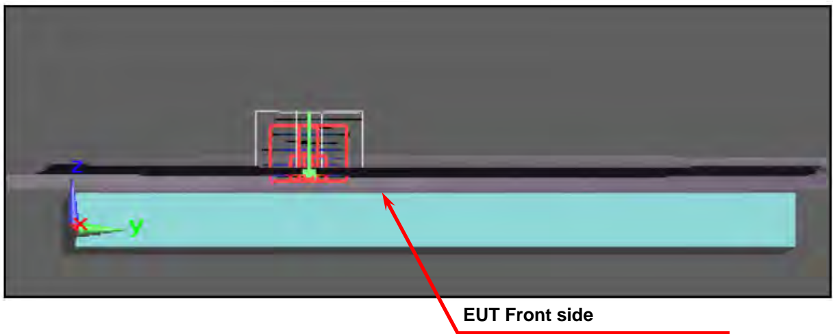
Figure 1. Body SAR Test Setup (Flat Section)
