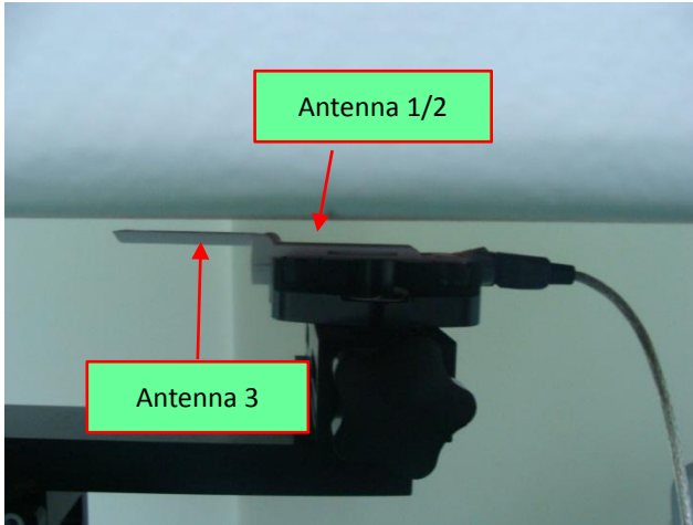
USB Cable Plug-in Horizontal Down_Flip 180° 5 mm Gap to Phantom
