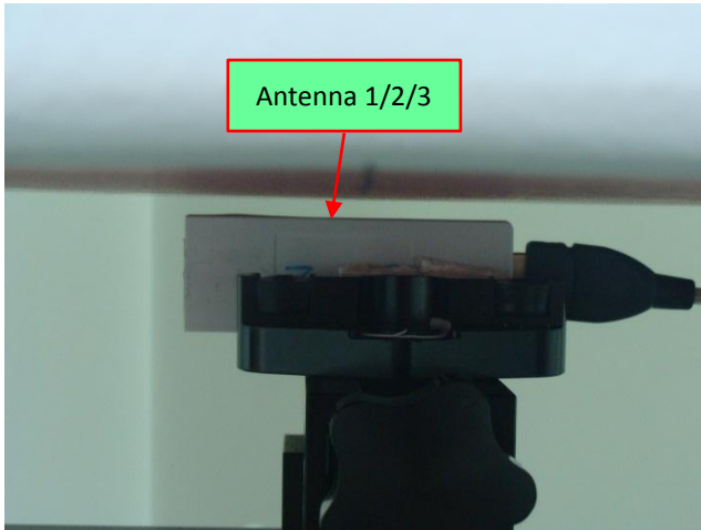
USB Cable Plug-in for Vertical Front_Flip 90° 5 mm Gap to Phantom
