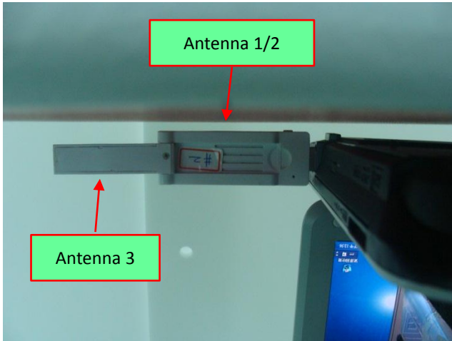
Direct Laptop Plug-in Vertical Back_Flip 180° 5 mm Gap to Phantom
