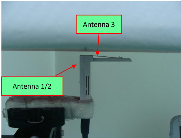
USB Cable Plug-in Horizontal Down_Flip 90° (Flip Front) 5 mm Gap to Phantom
