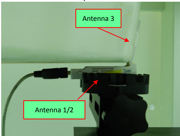
USB Cable Plug-in Horizontal Down_Flip 90° 5 mm Gap to Phantom Revised test configuration for Ant. 1/2
