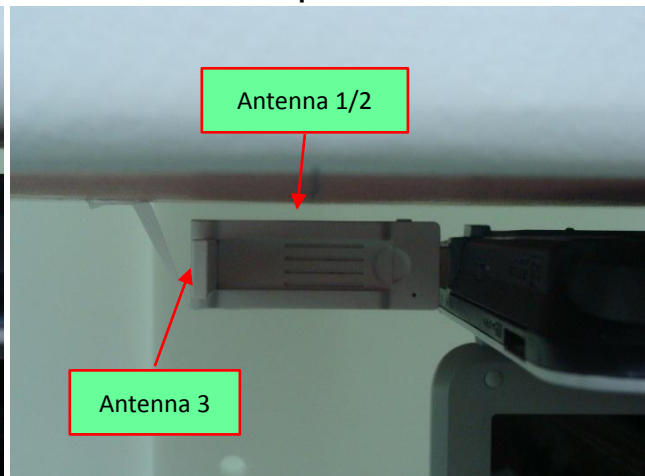
Direct Laptop Plug-in Vertical Back_Flip 90° 5 mm Gap to Phantom
