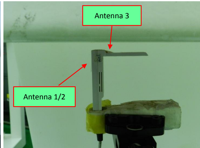
USB Cable Plug-in Horizontal Down_Flip 90° (Flip Front) 10 mm Gap to Phantom
