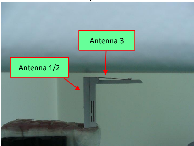
USB Cable Plug-in Horizontal Down_Flip 90° (Flip Front) 5 mm Gap to Phantom
