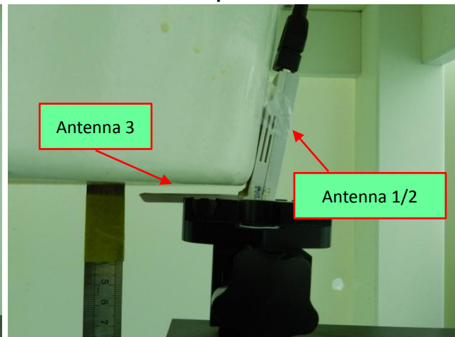
USB Cable Plug-in Horizontal Down_Flip 90° (Flip Back) 5 mm Gap to Phantom Revised test configuration for Ant. 3
