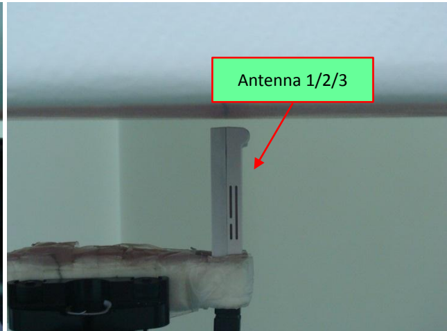
Direct Laptop Plug-in Tip Mode_Flip closed 5 mm Gap to Phantom
