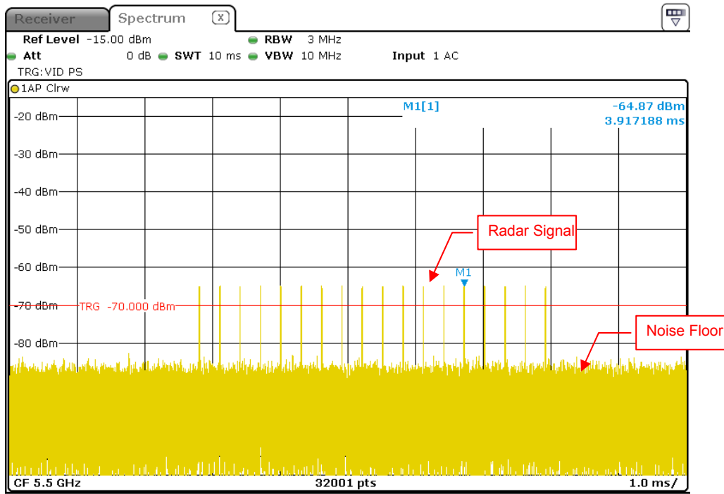
Radar Signal 3
