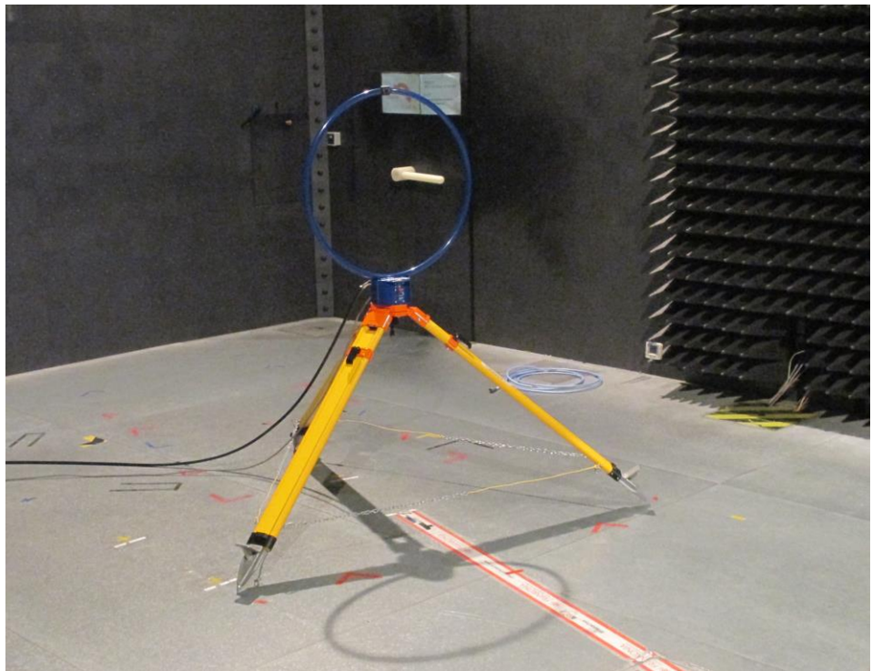
REAR VIEW
