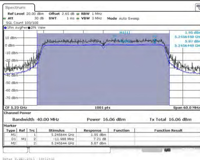
5150-5250MHz - Worst RF Output Power Plots
