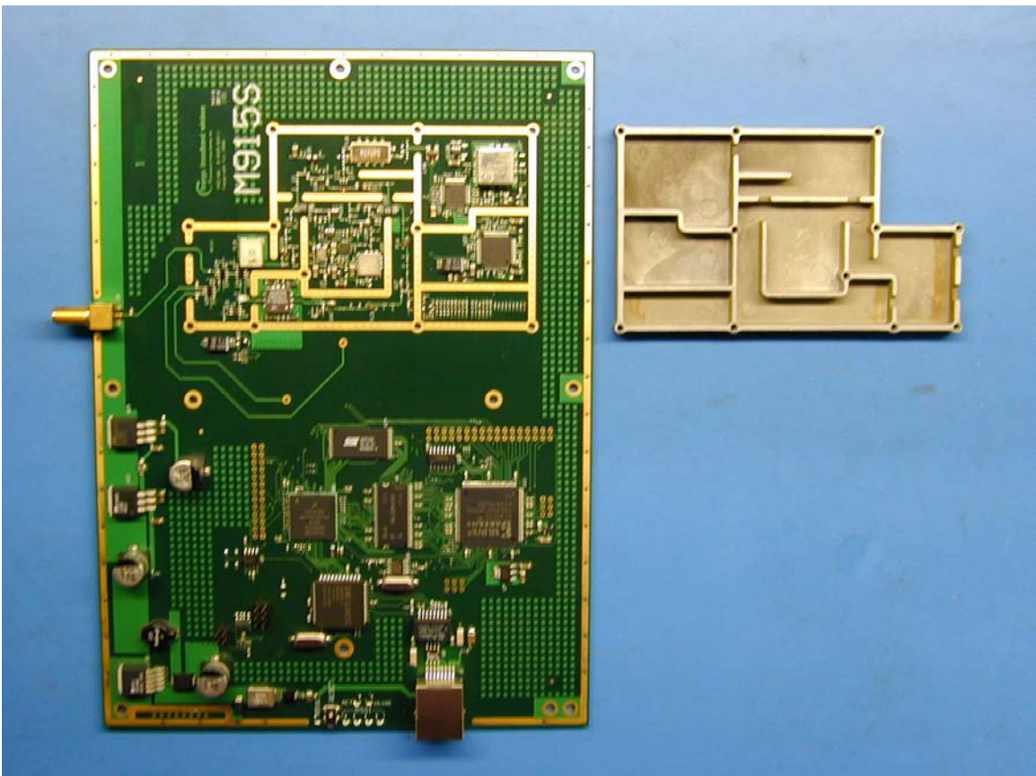
Top with shield removed, showing RF section.
