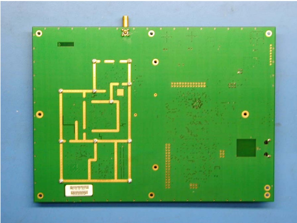
Bottom with Patch antenna removed
