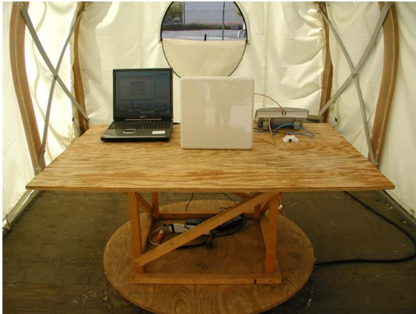
Radiated Emission - Front View for 23 dBi Patch Antenna
