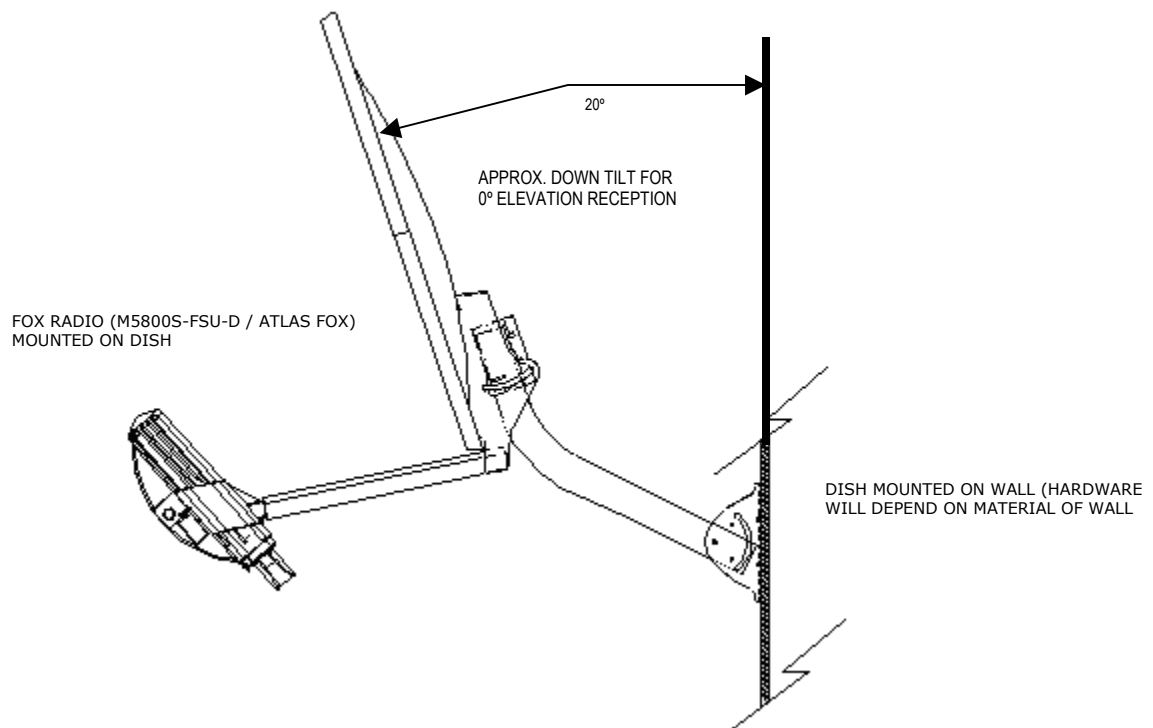
Figure 7-8: FOX5800-D / AD5800-25 Reflector Dish on Wall
