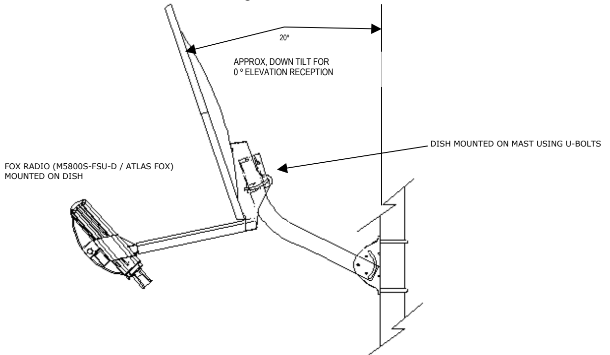
Figure 7-7: FOX5800-D / AD5800-25 Reflector Dish on Pole
