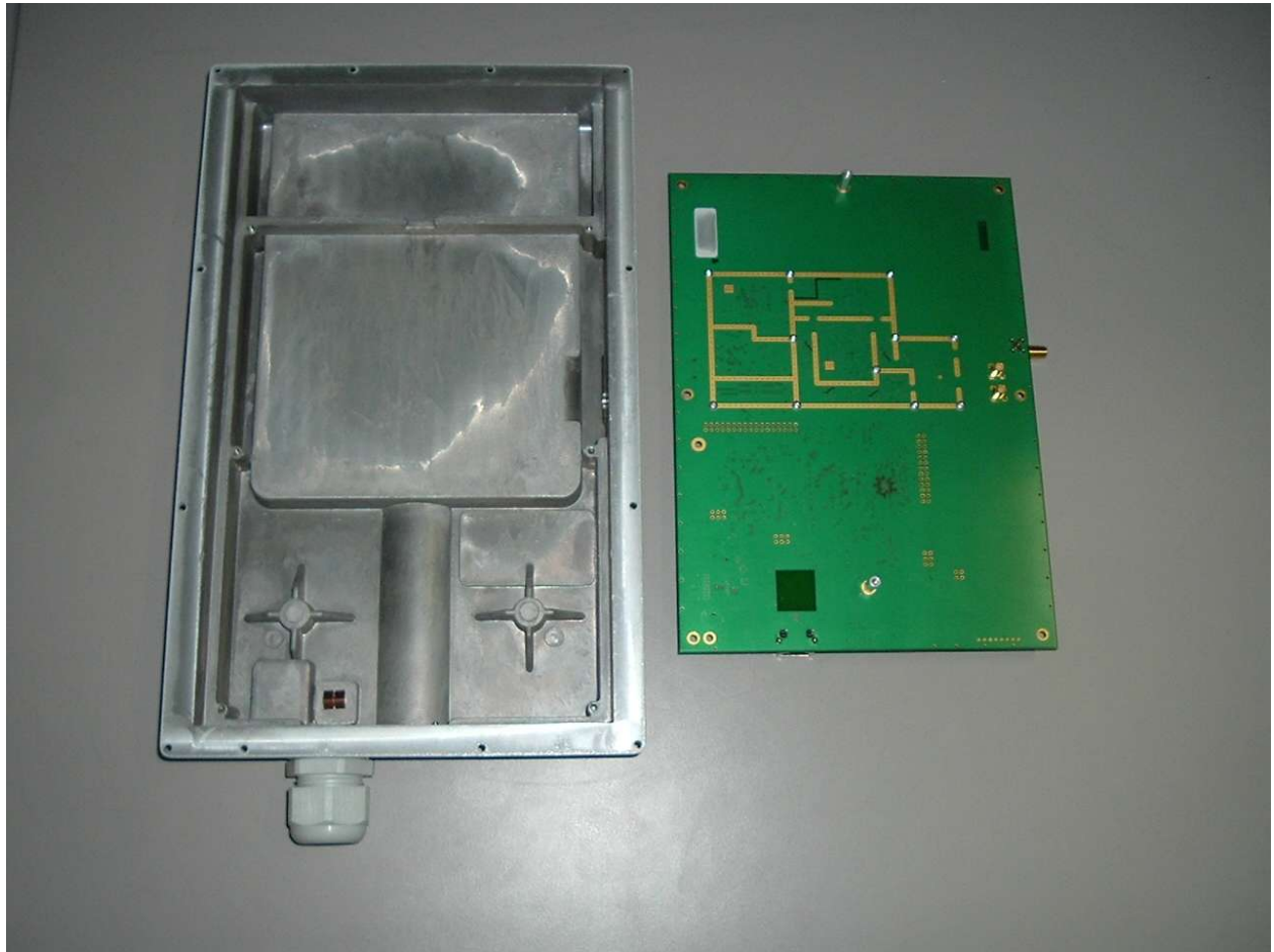
PCB Front and External Shield:
