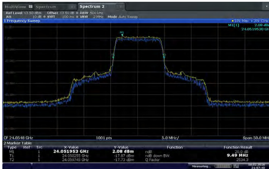
10 MHz BW (Low Channel)
