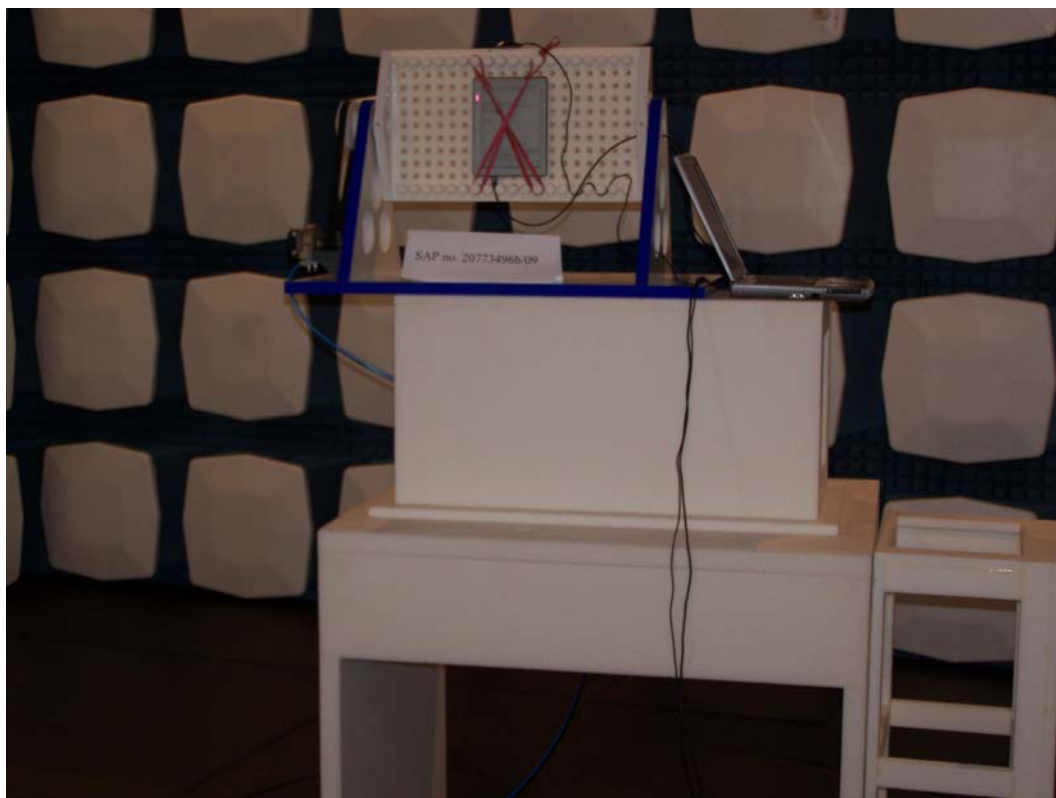
Measurement set-up 1
