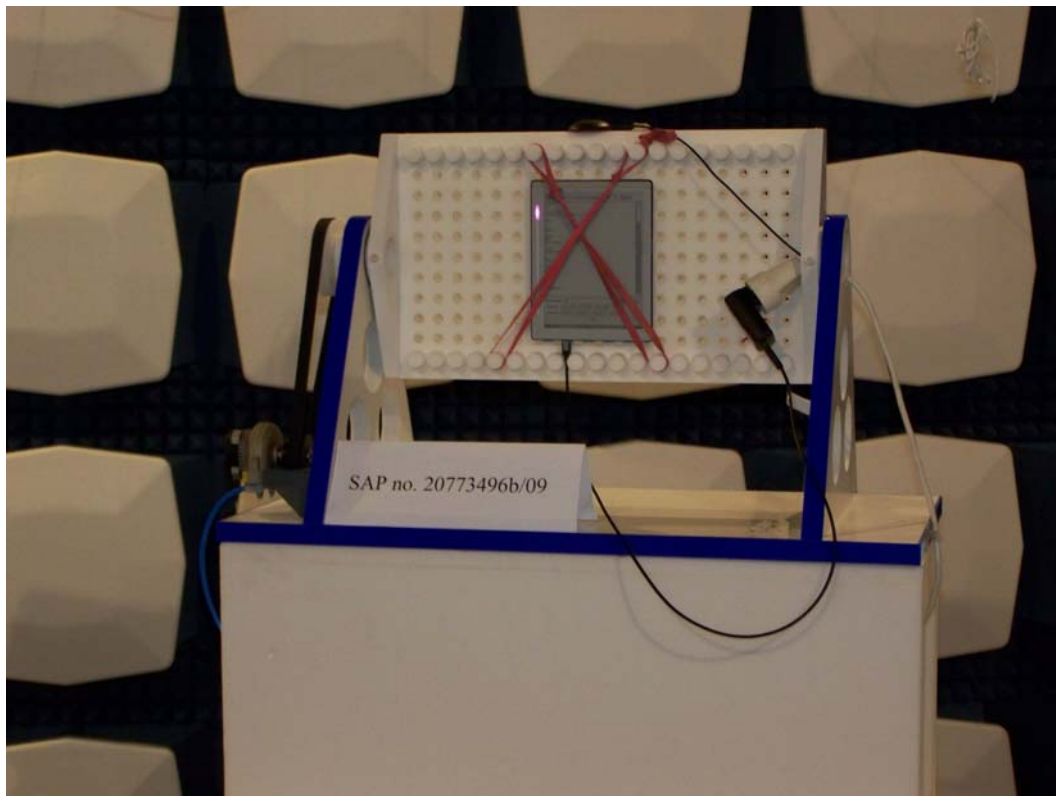
Measurement set-up 2+3
