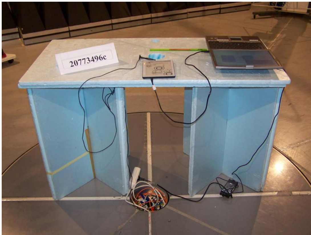
Radiated measurement set-up – radiated EMI measurements
