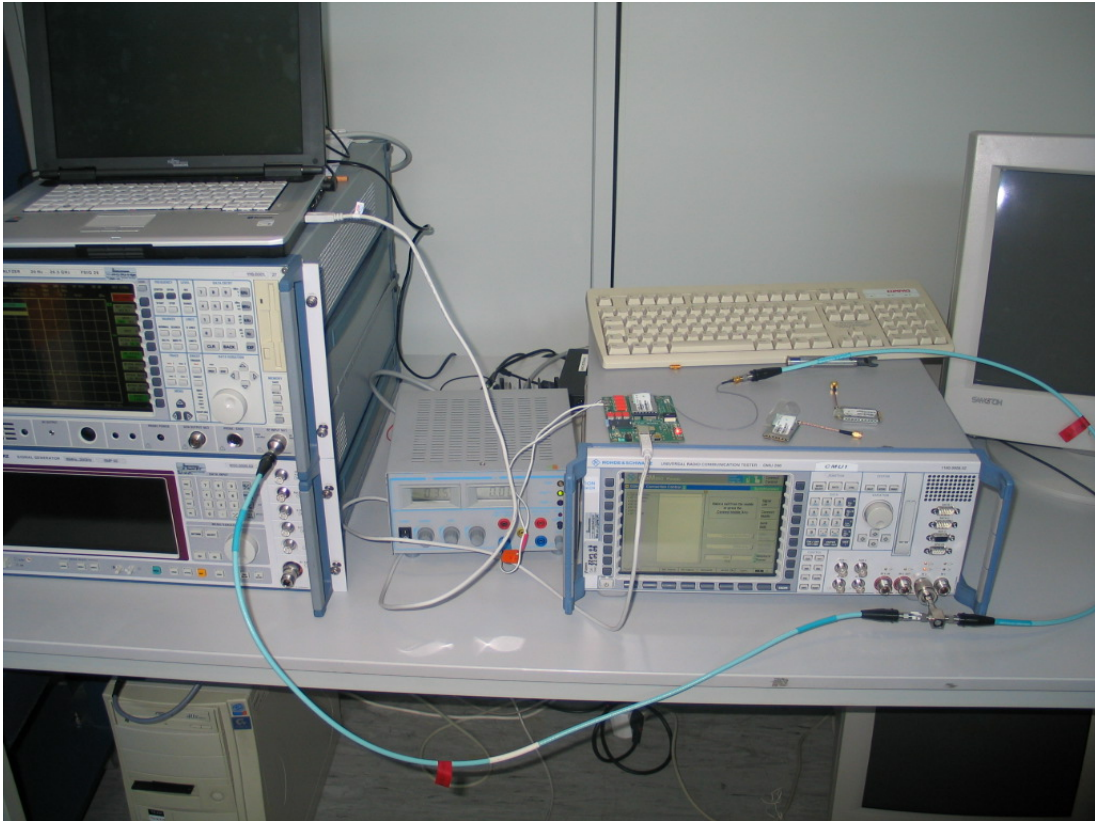
Photo 2: Setup for conducted tests
