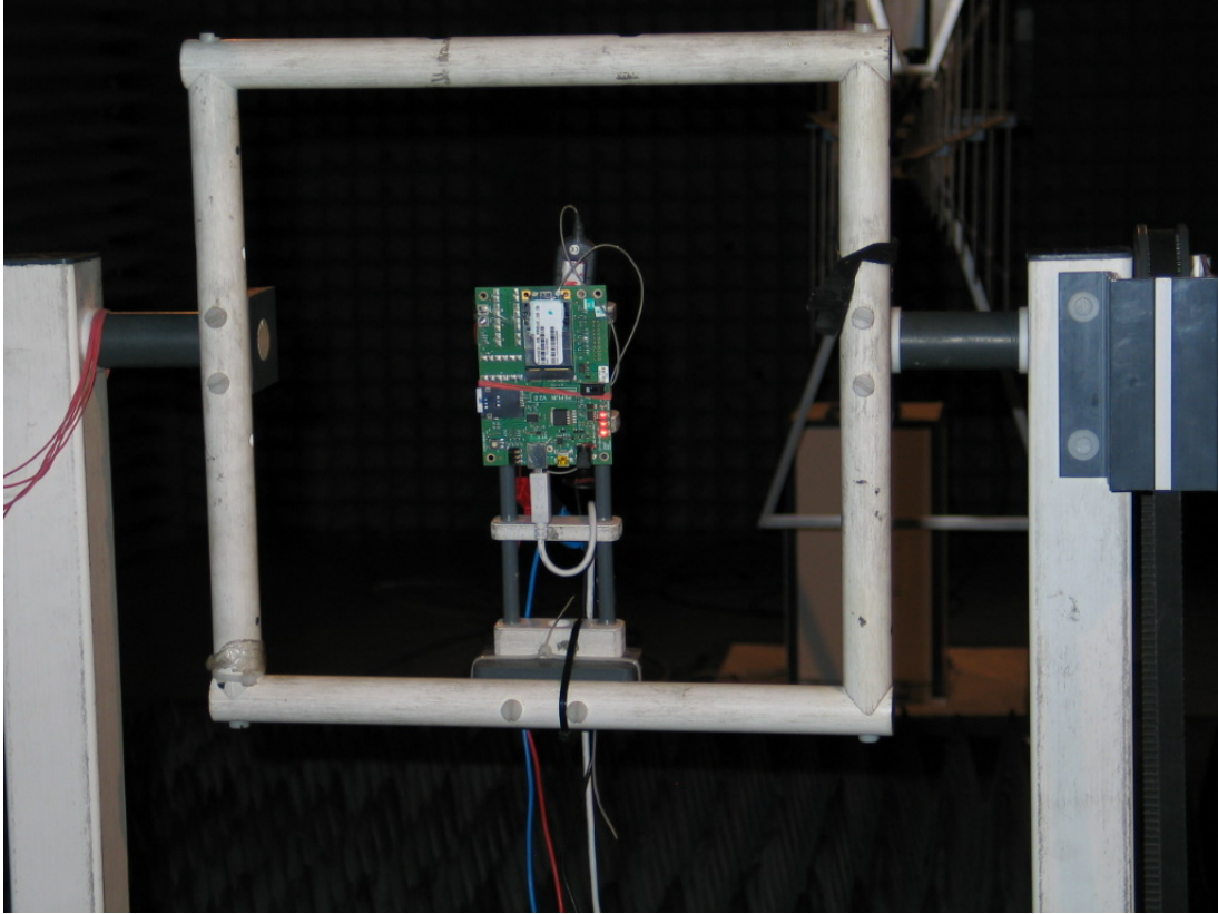
Photo 1: Setup for radiated tests
