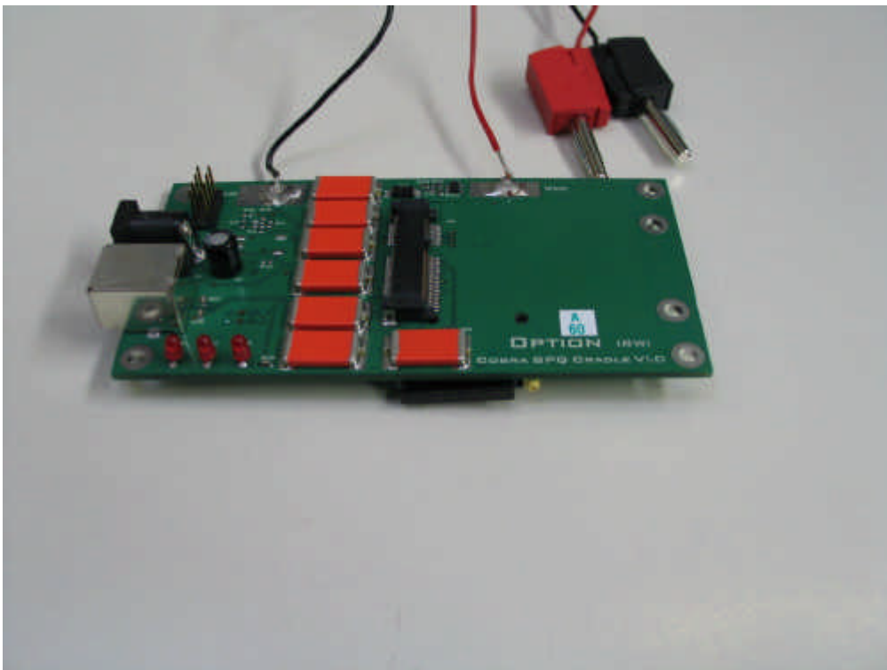
Photo 5: Test cradle Cobra SPQ
