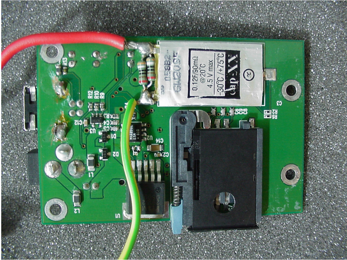
Photo 9: Cradle (rear side)
