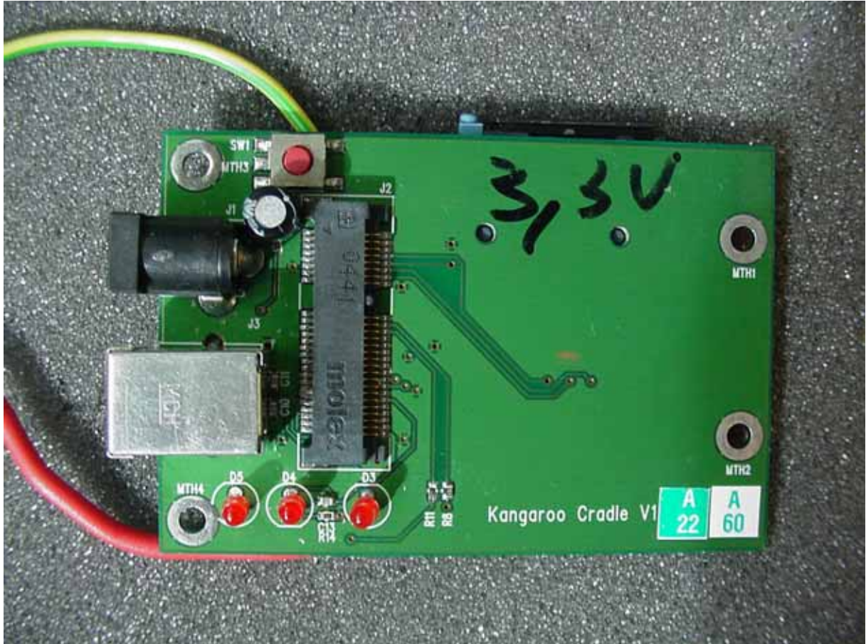
Photo 4: Cradle (front side)
