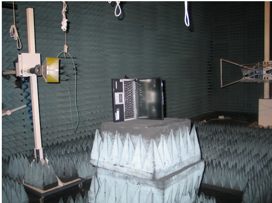
Photo 4: Test setup b01 in the anechoic chamber
