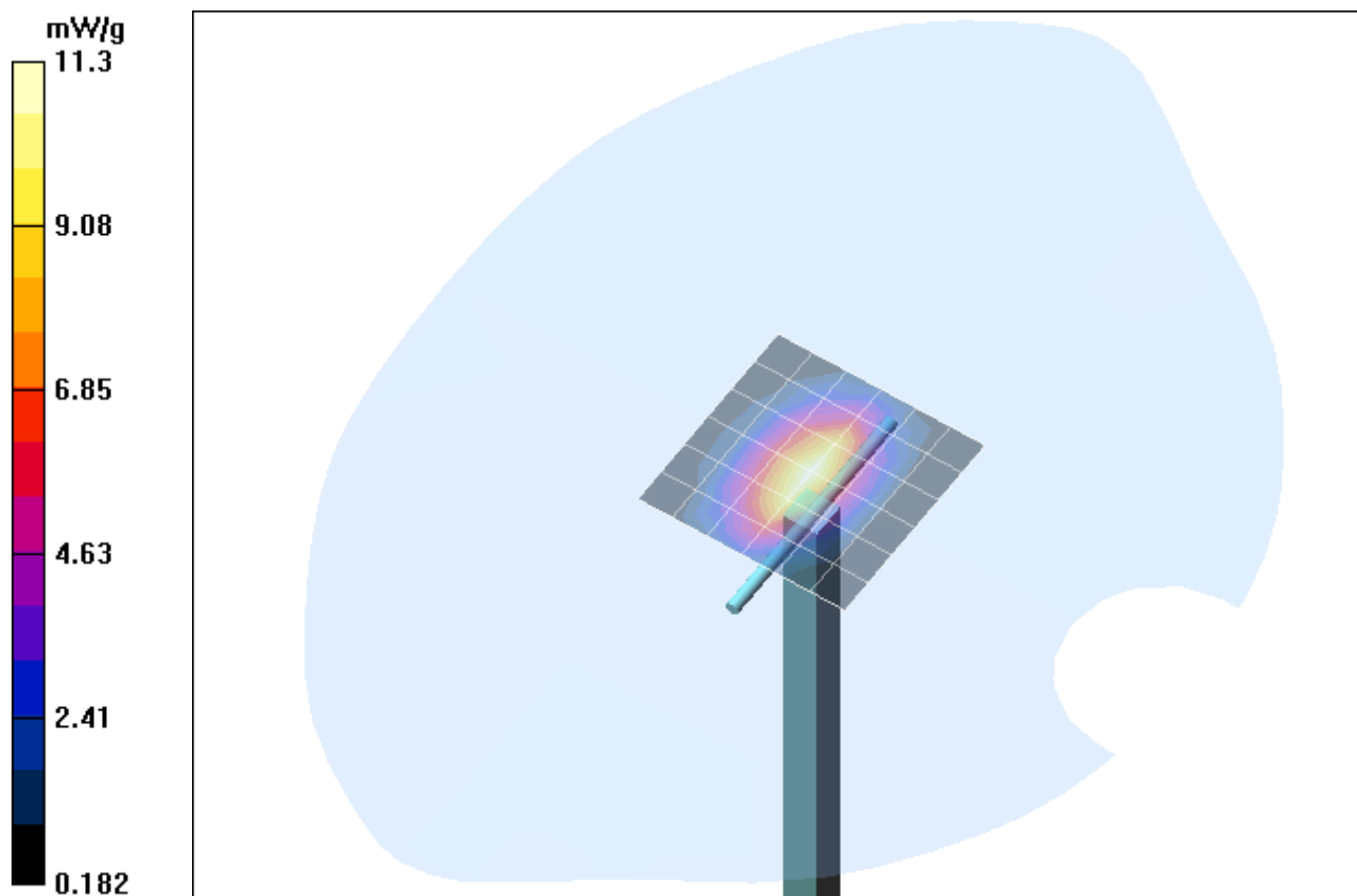
Fig. 16: Validation measurement 1900 MHz Body (WCDMA II, April 23, 2007), coarse grid. Ambient Temperature: 22.1°C, Liquid Temperature: 21.3°C.
