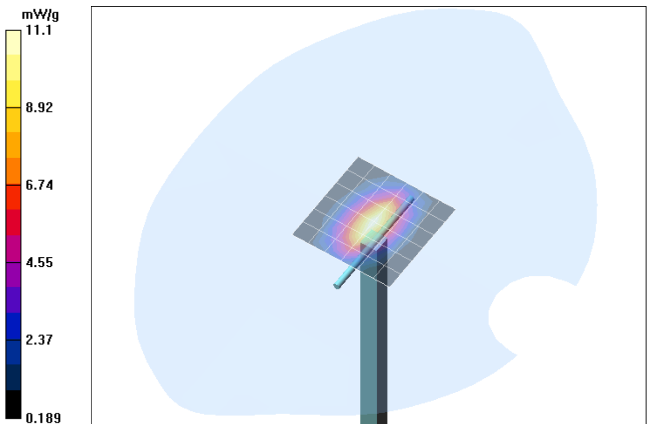
Fig. 15: Validation measurement 1900 MHz Body (GSM 1900, April 24, 2007), coarse grid. Ambient Temperature: 22.1°C, Liquid Temperature: 21.2°C.
