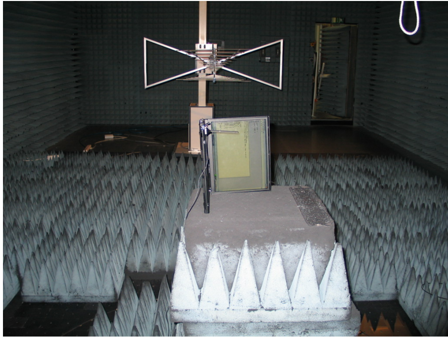
Photo 5: Test setup c01 in the anechoic chamber
