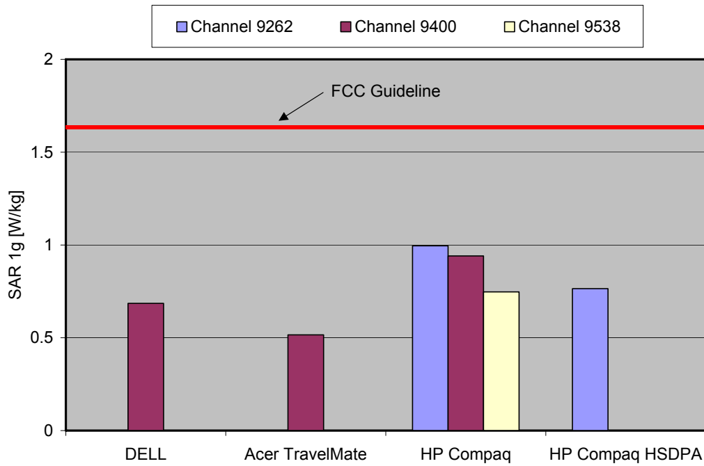
Fig. 11: The measured SAR values for the Option Globetrotter GT for WCDMA II (FDD) in comparison to the FCC exposure limit.
