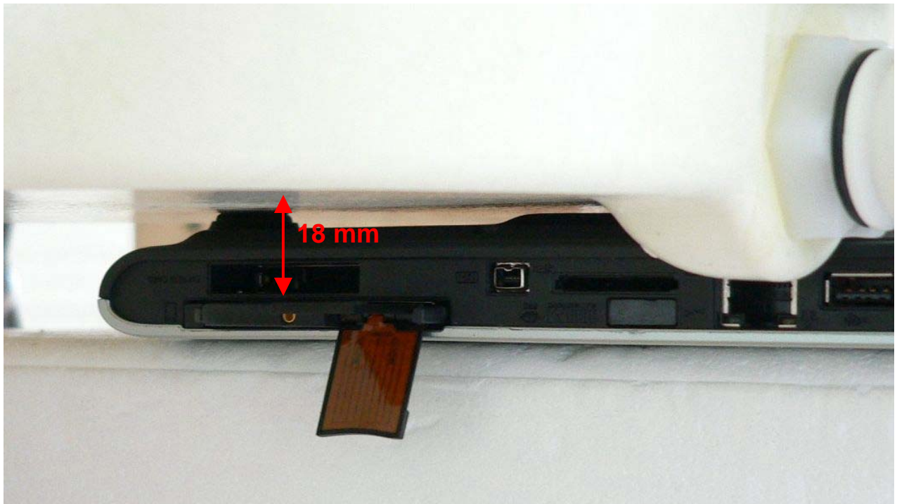
Fig. 25: Lap Held Position with the Acer TravelMate, antenna in intended use position.
