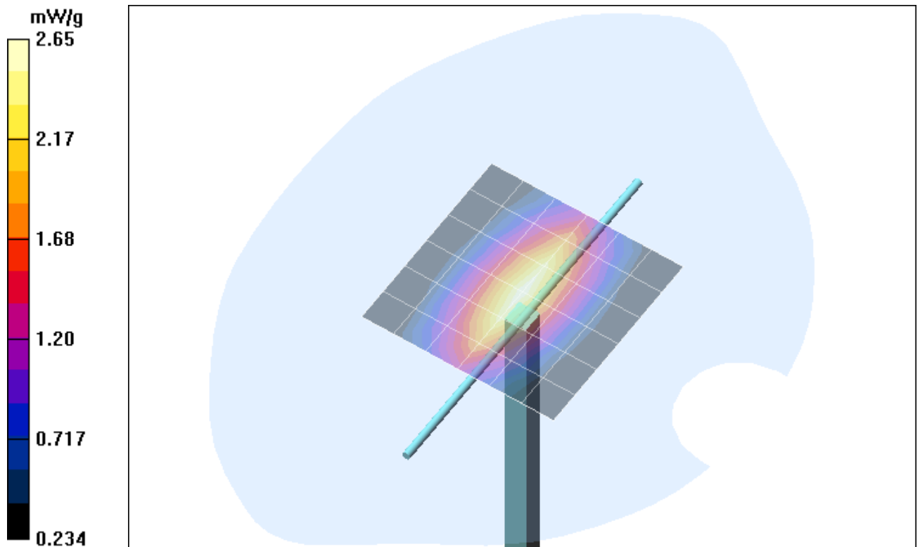
Fig. 14: Validation measurement 835 MHz Body (WCDMA V, April 25, 2007), coarse grid. Ambient Temperature: 22.1°C, Liquid Temperature: 21.0°C.
