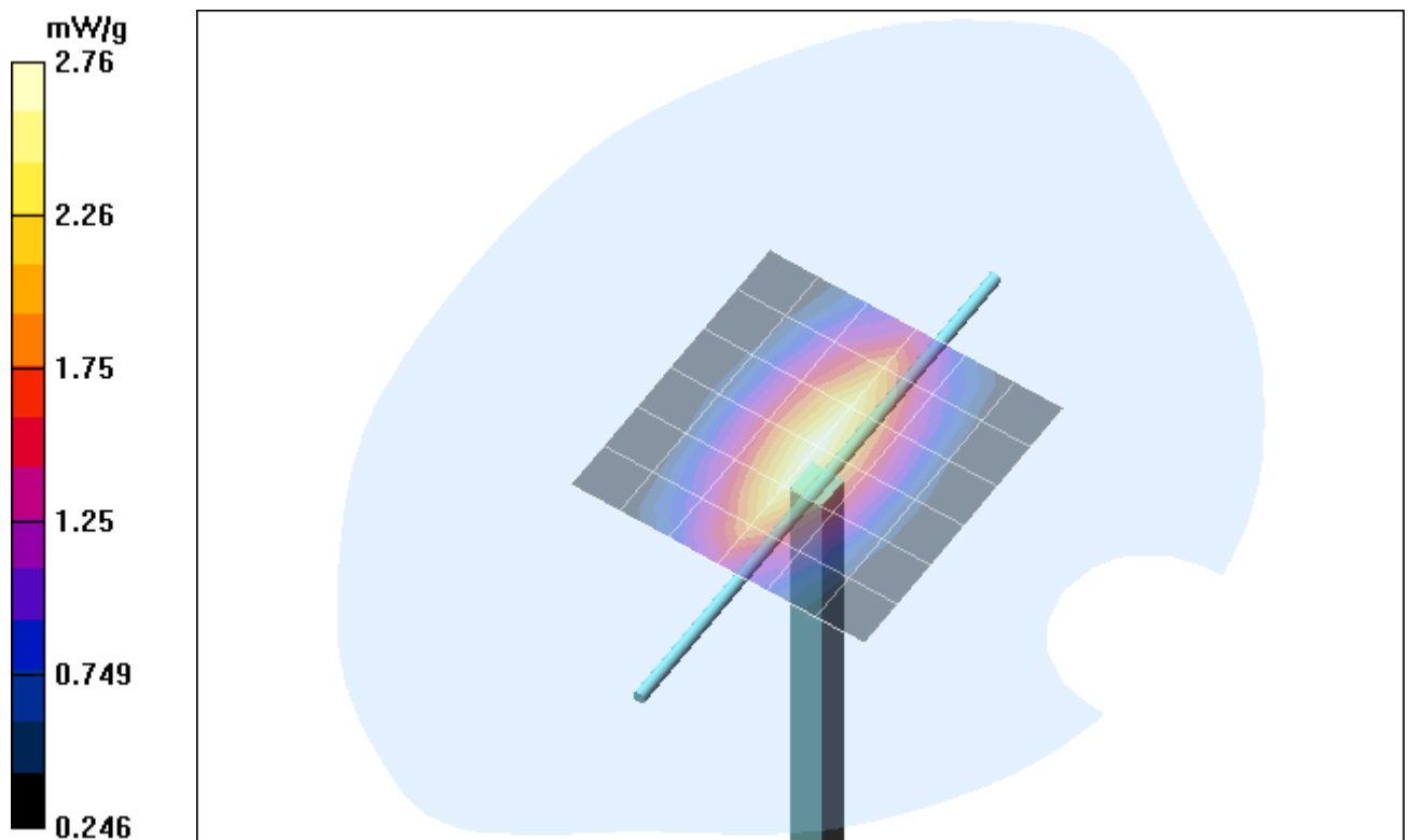
Fig. 13: Validation measurement 835 MHz Body (GSM 850, April 18, 2007), coarse grid. Ambient Temperature: 22.2C, Liquid Temperature: 21.3°C.
