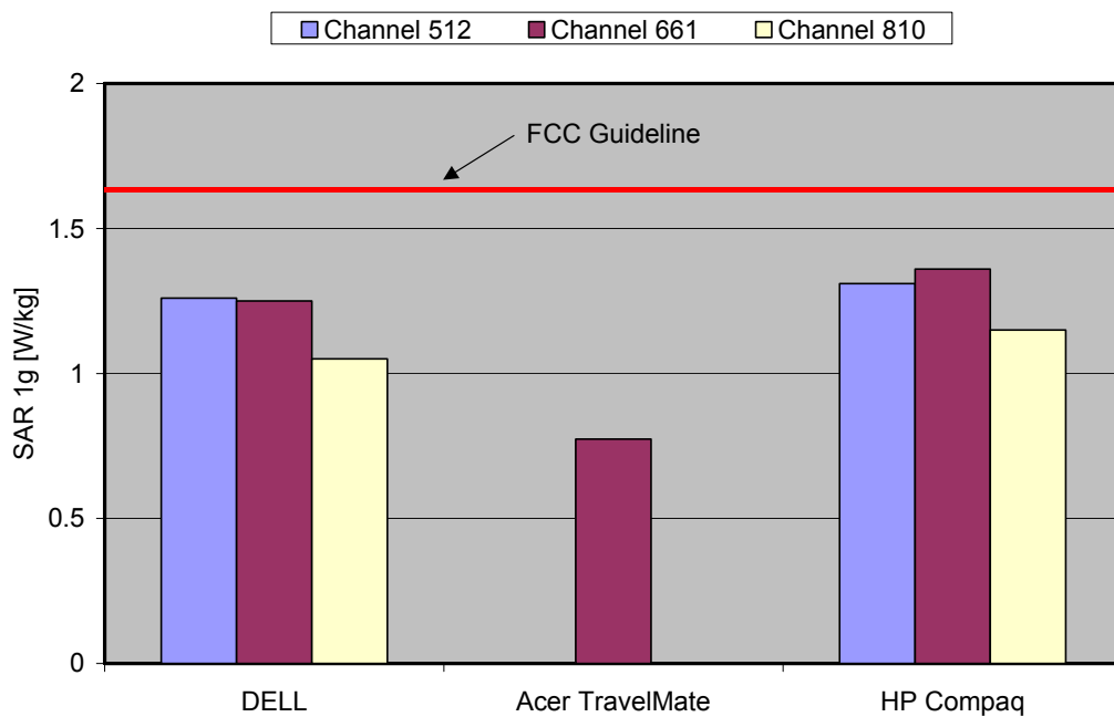
Fig. 10: The measured SAR values for the Option Globetrotter GT for GPRS 1900 (Class 12) in comparison to the FCC exposure limit.
