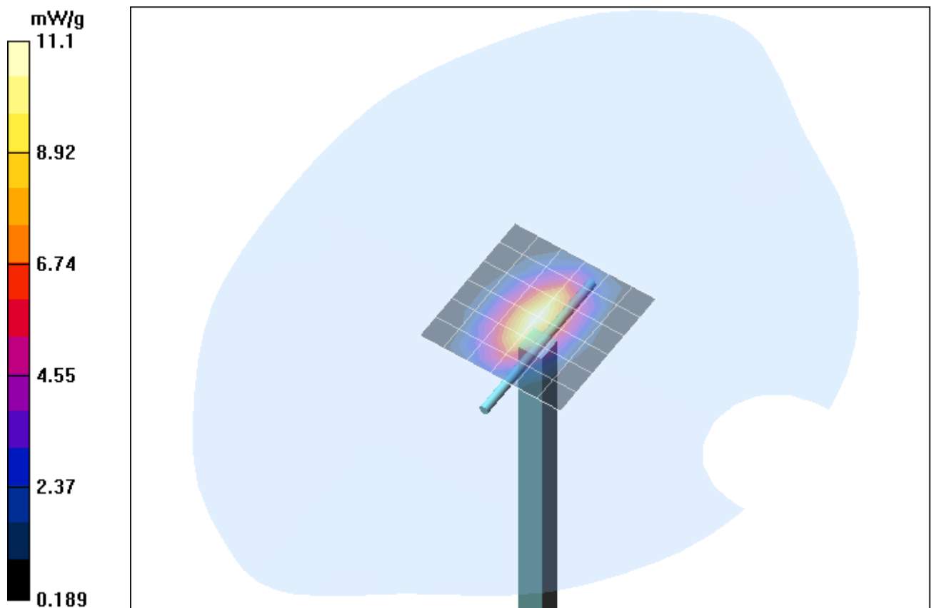
Fig. 15: Validation measurement 1900 MHz Body (GSM 1900, April 24, 2007), coarse grid. Ambient Temperature: 22.1°C, Liquid Temperature: 21.2°C.
