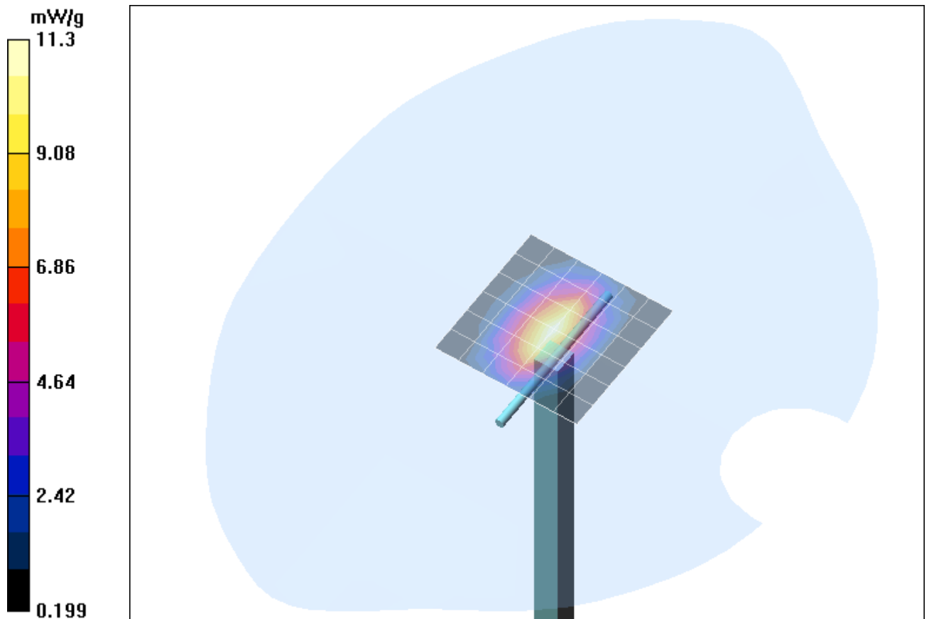
Fig. 18: Validation measurement 1900 MHz Body (WCDMA II, HSDPA, May 29, 2007), coarse grid. Ambient Temperature: 22.0°C, Liquid Temperature: 21.2°C.
