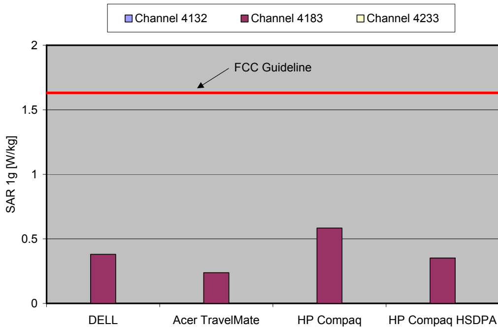
Fig. 12: The measured SAR values for the Option Globetrotter GT for WCDMA V (FDD) in comparison to the FCC exposure limit.
