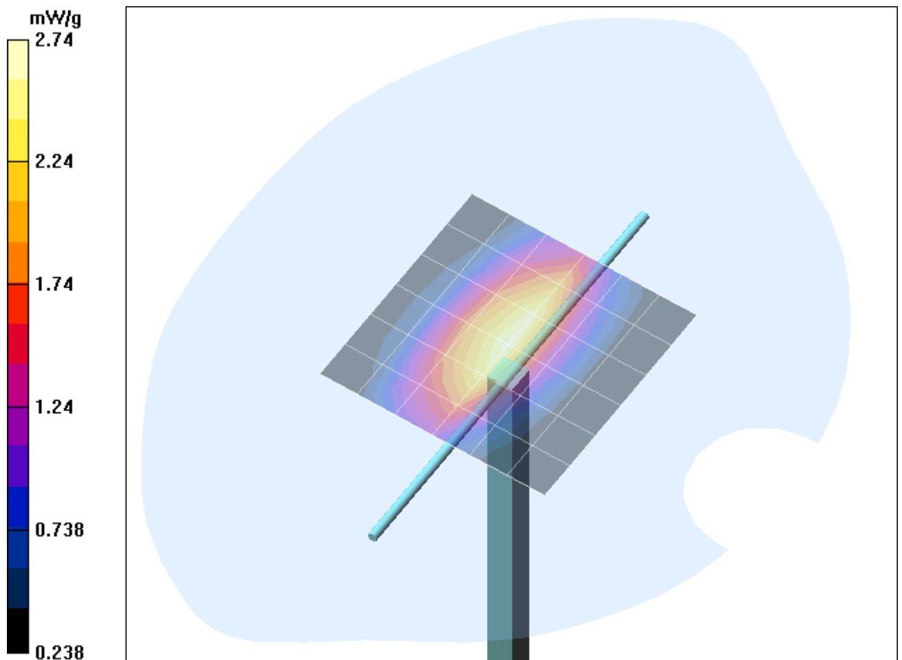
Fig. 17: Validation measurement 835 MHz Body (WCDMA V, HSDPA, May 29, 2007), coarse grid. Ambient Temperature: 22.3°C, Liquid Temperature: 21.5°C.
