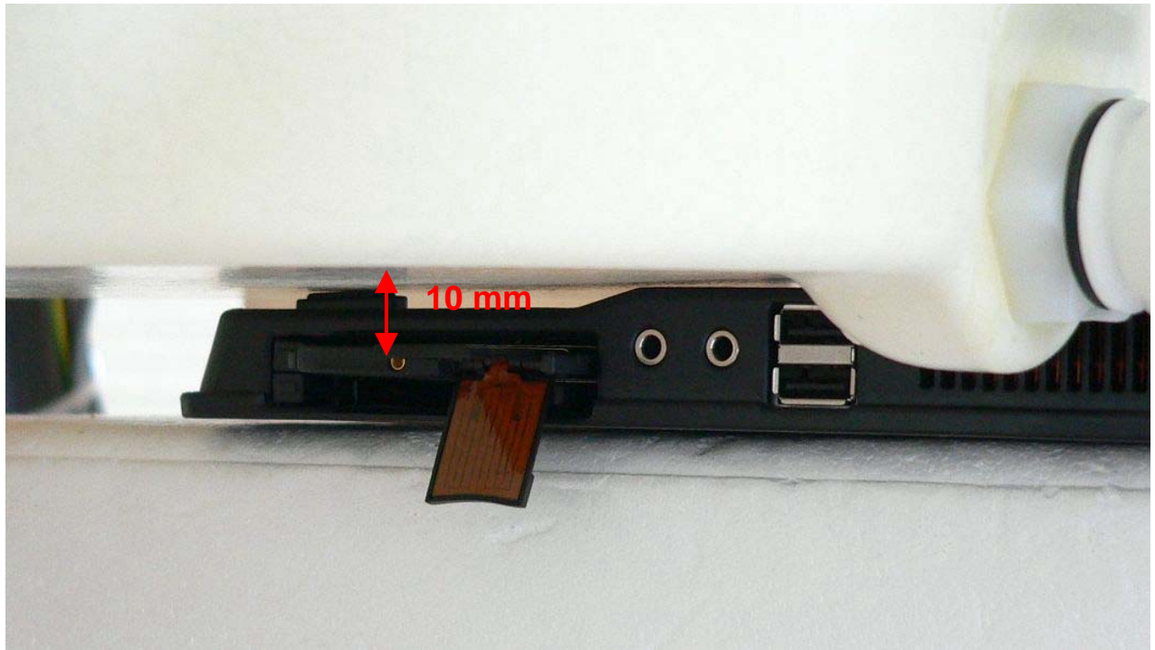
Fig. 26: Lap Held Position with the HP Compaq nc 6320, antenna in intended use position
