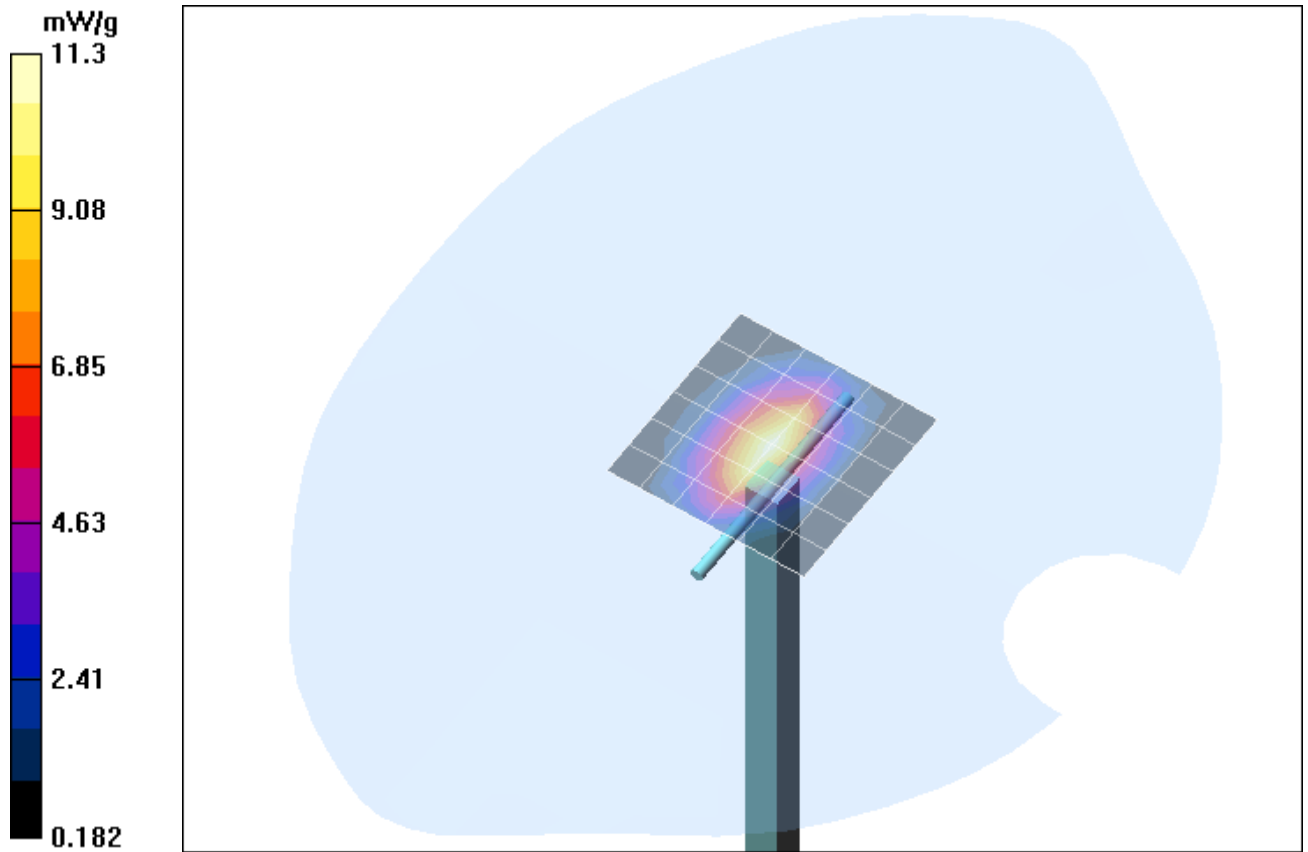
Fig. 16: Validation measurement 1900 MHz Body (WCDMA II, April 23, 2007), coarse grid. Ambient Temperature: 22.1°C, Liquid Temperature: 21.3°C.
